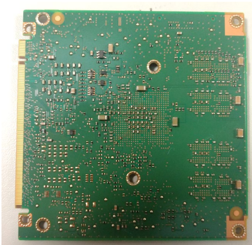
Daughterboard Bottom
