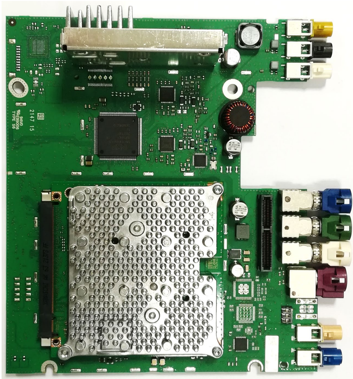
Motherboard Top
