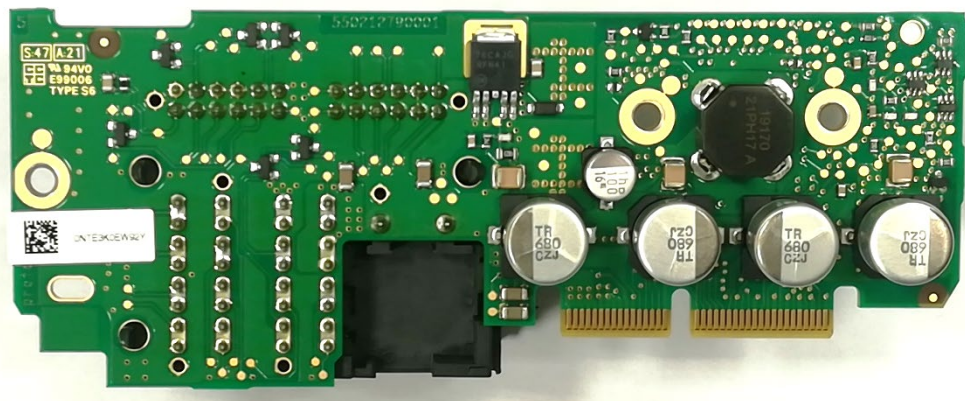
Powerboard Bottom
