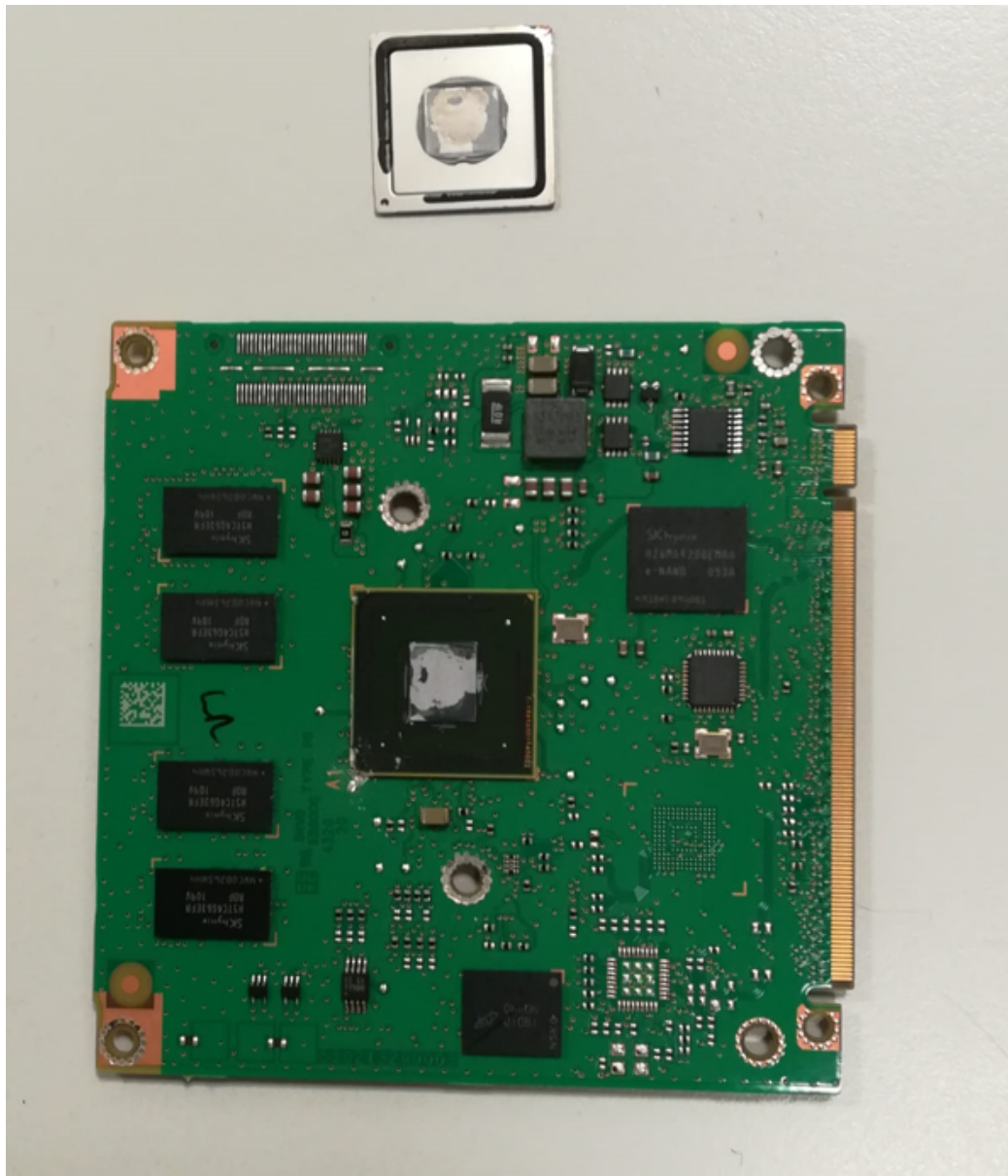
Daughterboard Top
