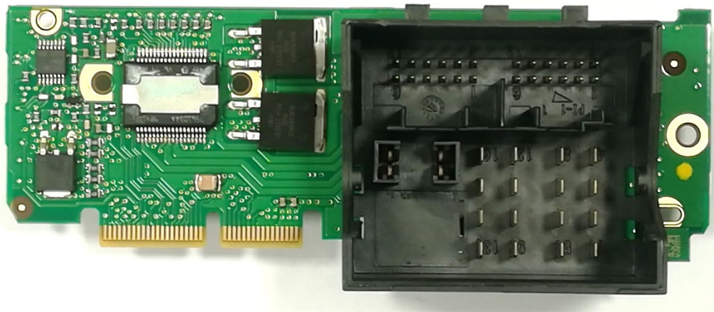
Powerboard Top
