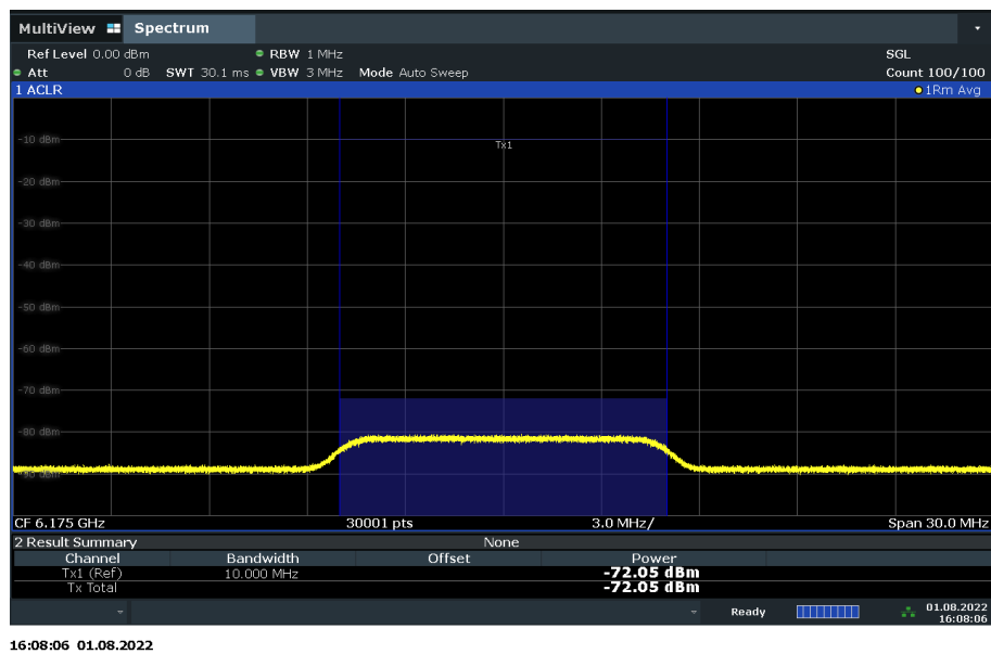
Fig.117 Contention Based Protocol 802.11ax HE160 (Upper edge Threshold Level)
