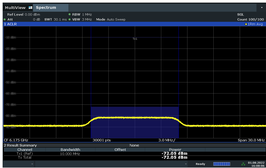
Fig.115 Contention Based Protocol 802.11ax HE20
