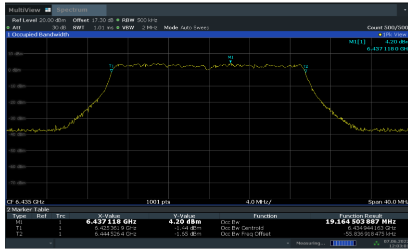
Fig.74 99% Occupied Bandwidth (802.11ax-HE20, 6435MHz)
