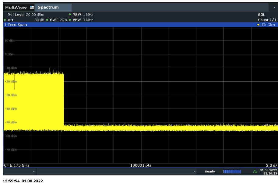
Fig.116 Contention Based Protocol 802.11ax HE20 (ceased transmission)
