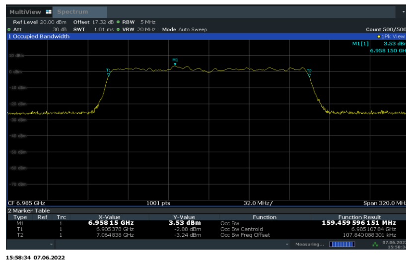
Fig.114 99% Occupied Bandwidth (802. 11ax-HE160 6985MHz)
