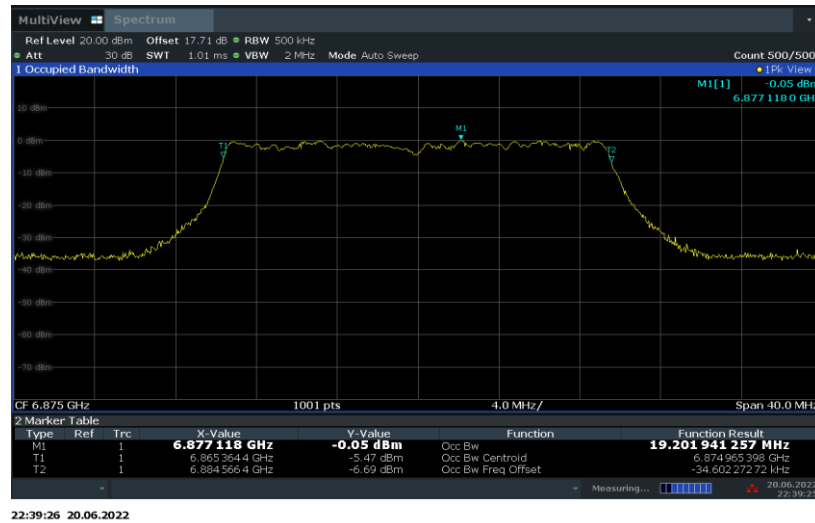
Fig.80 99% Occupied Bandwidth (802.11ax-HE20, 6875MHz)
