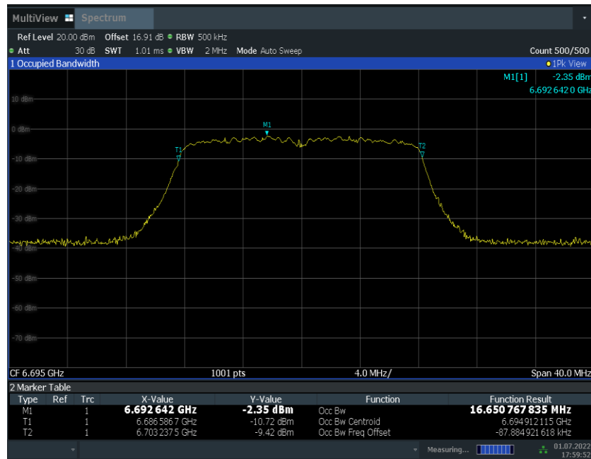
Fig.65 99% Occupied Bandwidth (802.11a, 6695MHz)
