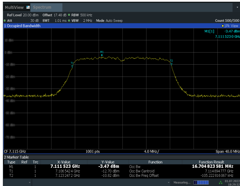
Fig.70 99% Occupied Bandwidth (802.11a, 7115MHz)
