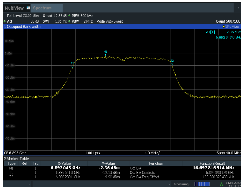
Fig.68 99% Occupied Bandwidth (802.11a, 6895MHz)
