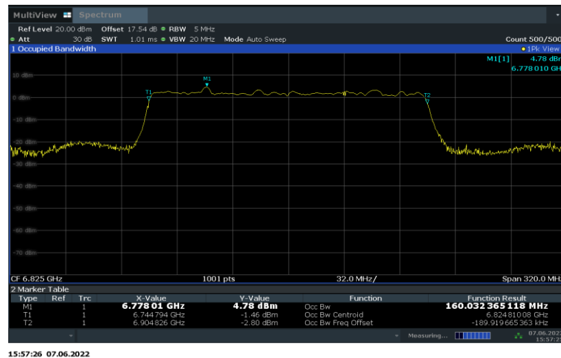
Fig.113 99% Occupied Bandwidth (802. 11ax-HE160, 6825MHz)
