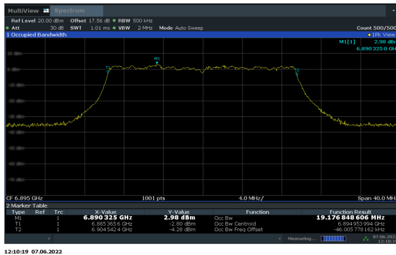
Fig.81 99% Occupied Bandwidth (802.11ax-HE20, 6895MHz)
