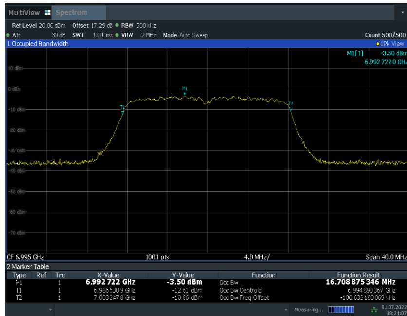
Fig.69 99% Occupied Bandwidth (802.11a 6995MHz)
