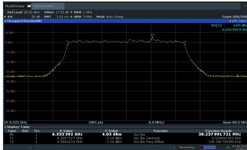
Fig.89 99% Occupied Bandwidth (802.11ax-HE40, 6525MHz)
