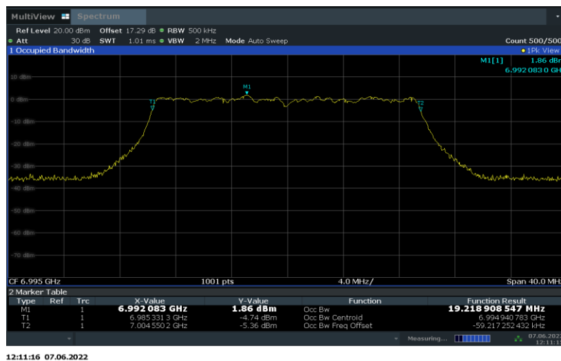
Fig.82 99% Occupied Bandwidth (802.11ax-HE20, 6995MHz)
