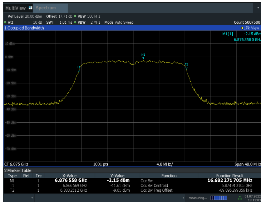
Fig.67 99% Occupied Bandwidth (802.11a, 6875MHz)
