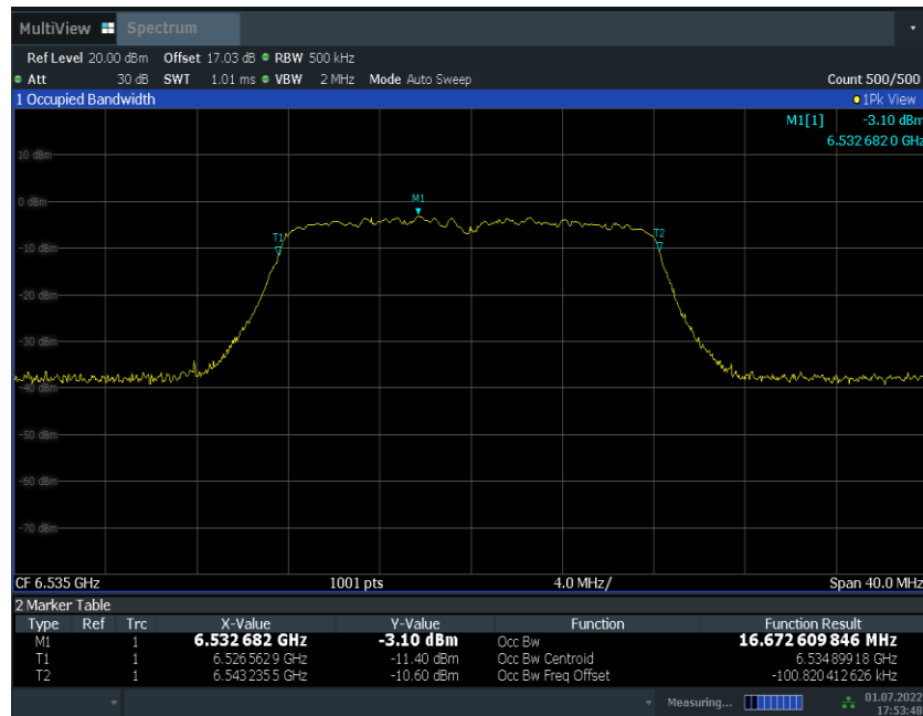
Fig.64 99% Occupied Bandwidth (802.11a, 6535MHz)
