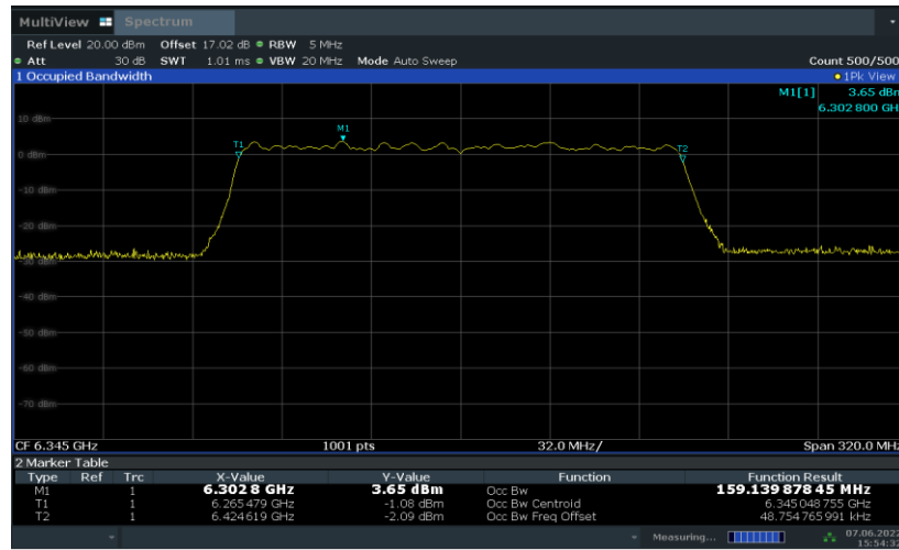
Fig.110 99% Occupied Bandwidth (802. 11ax-HE160, 6345MHz)
