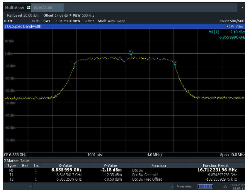
Fig.66 99% Occupied Bandwidth (802.11a, 6855MHz)
