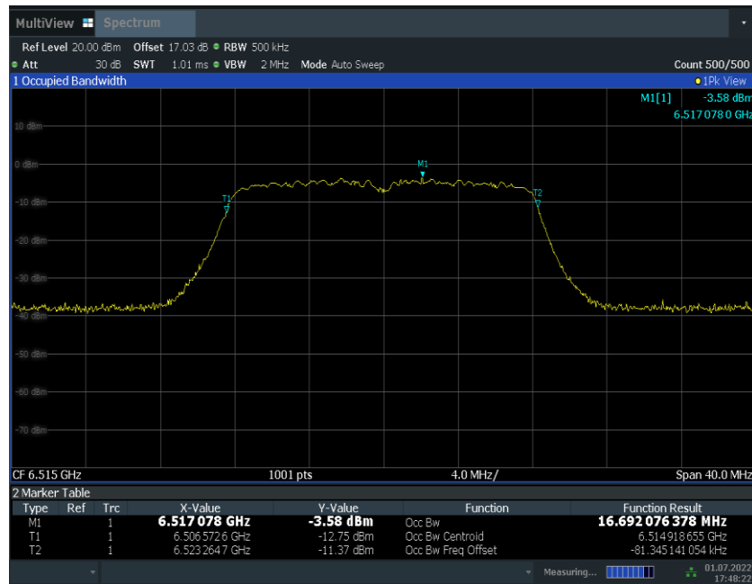
Fig.63 99% Occupied Bandwidth (802.11a, 6515MHz)
