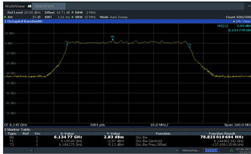
Fig.98 99% Occupied Bandwidth (802. 11ax-HE80, 6145MHz)
