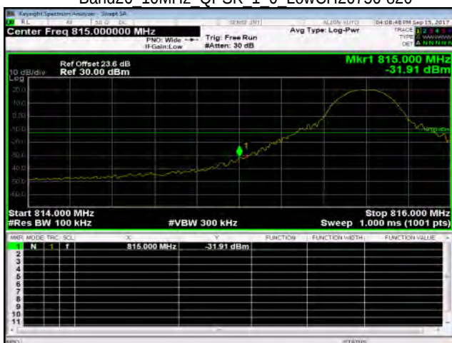
Band26 10MHz QPSK 1_0 LowCH26750-820
