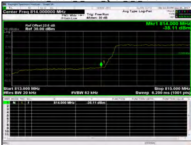
Part 90 Band26 1 4MHz QPSK 6 0 LowCH26697
