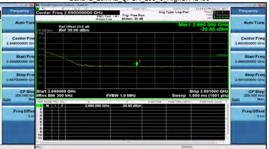
Band41 20MHz QPSK 100 0 HighCH41490
