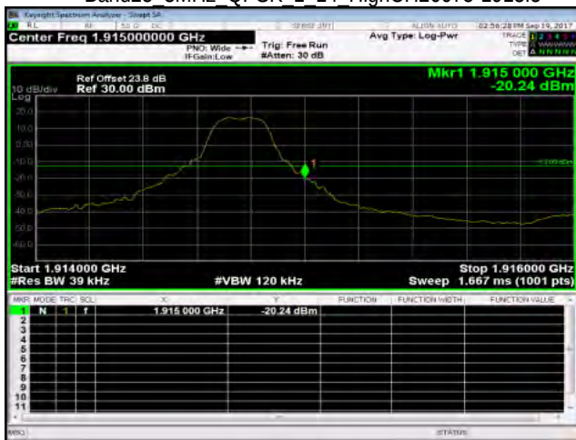
Band25 3MHz QPSK 1 14 HighCH26675-1913.5
