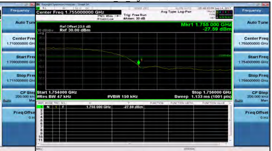
HSDPA B4 HighCH1513-1752.6
