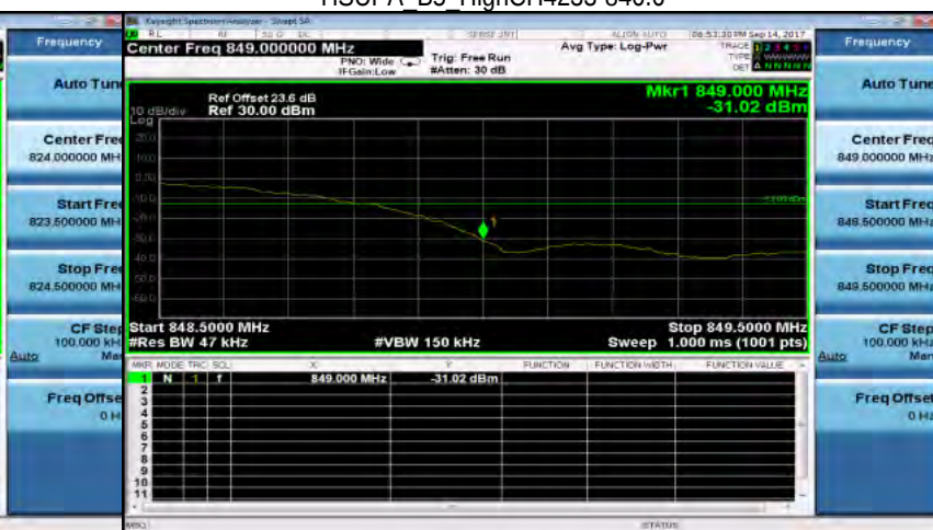
HSUPA B5 HighCH4233-846.6
