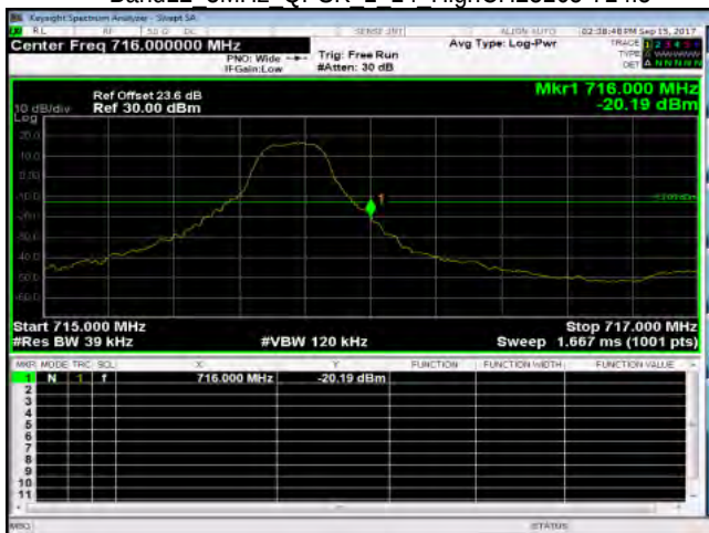
Band12 3MHz QPSK 1 14 HighCH23165-714.5
