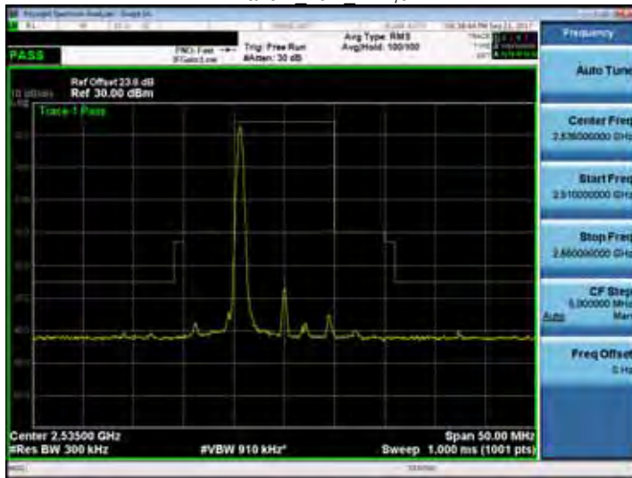
Band 7 10M RB1,49
