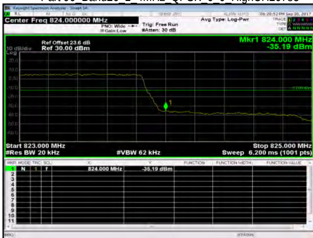
Part 90 Band26 1 4MHz QPSK 6 0 HighCH26783
