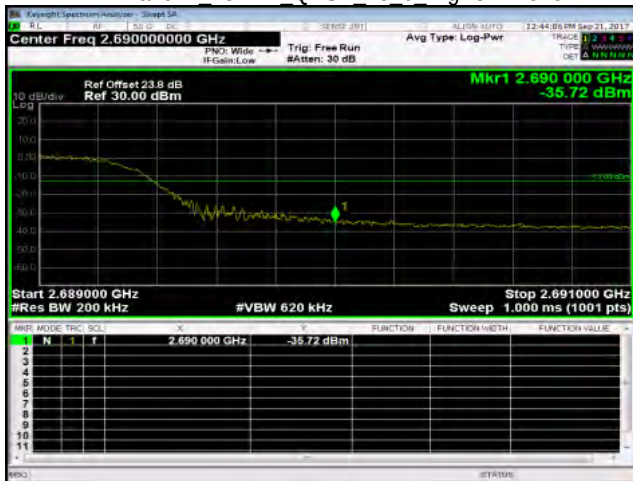
Band41 15MHz QPSK 75 0 HighCH41515
