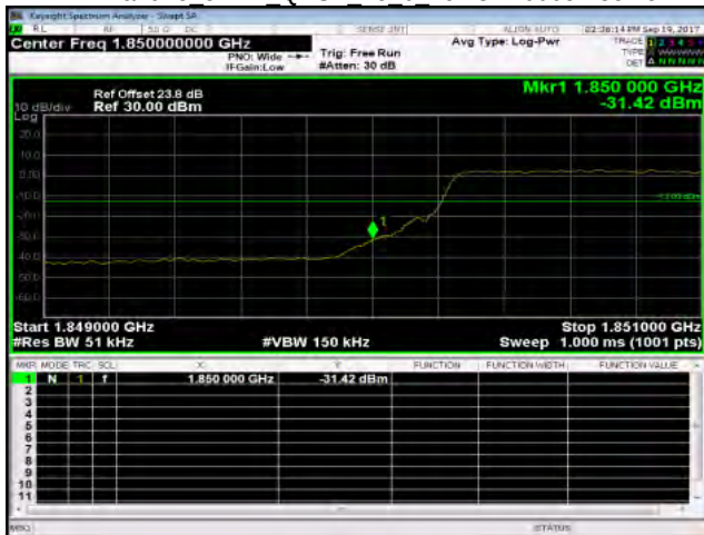
Band25 5MHz QPSK 25 0 LowCH26065-1852.5
