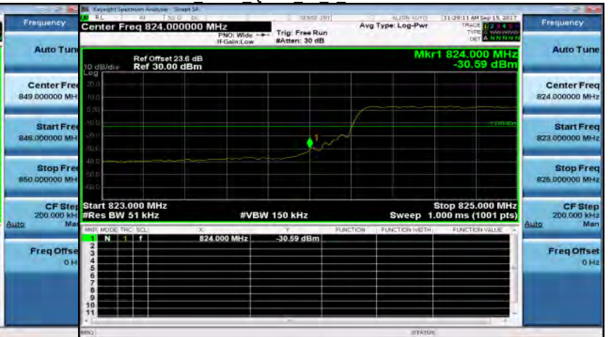
Band5 5MHz QPSK 25 0 LowCH20425-826.5
