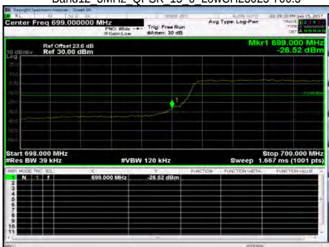
Band12 3MHz QPSK 15 0 LowCH23025-700.5
