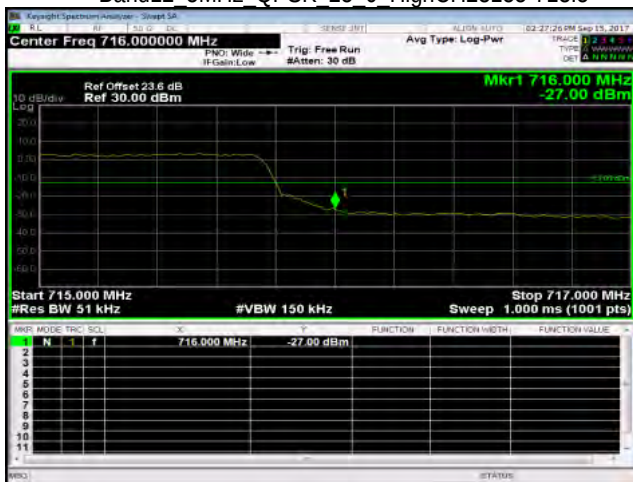
Band12 5MHz QPSK 25_0 HighCH23155-713.5
