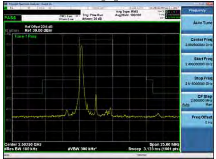
Band 7 5M RB1,24
