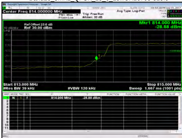
Band26 3MHz QPSK 15 0 LowCH26705-815.5
