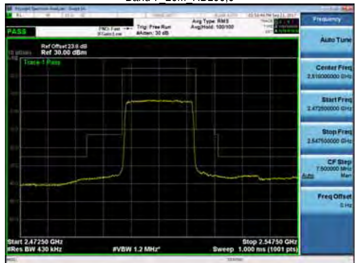
Band 7 20M RB100,0
