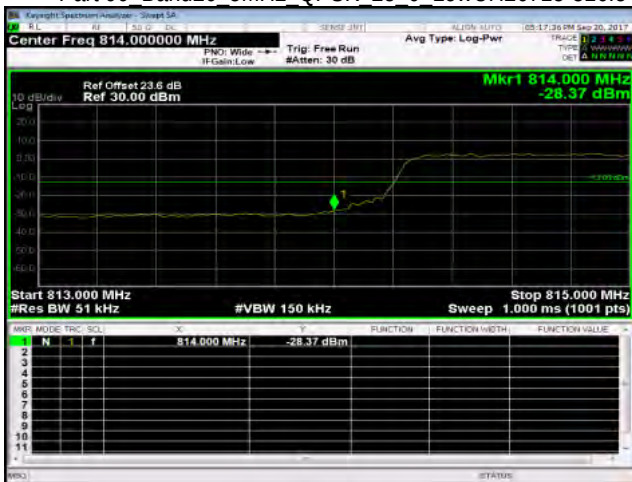
Part 90 Band26 5MHz QPSK 25 0 LowCH26715-816.5
