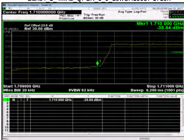
Band4 1 4MHz QPSK 6 0 LowCH19957-1710.7
