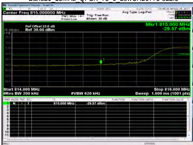
Band26 15MHz QPSK 75 0 LowCH26775-822.5
