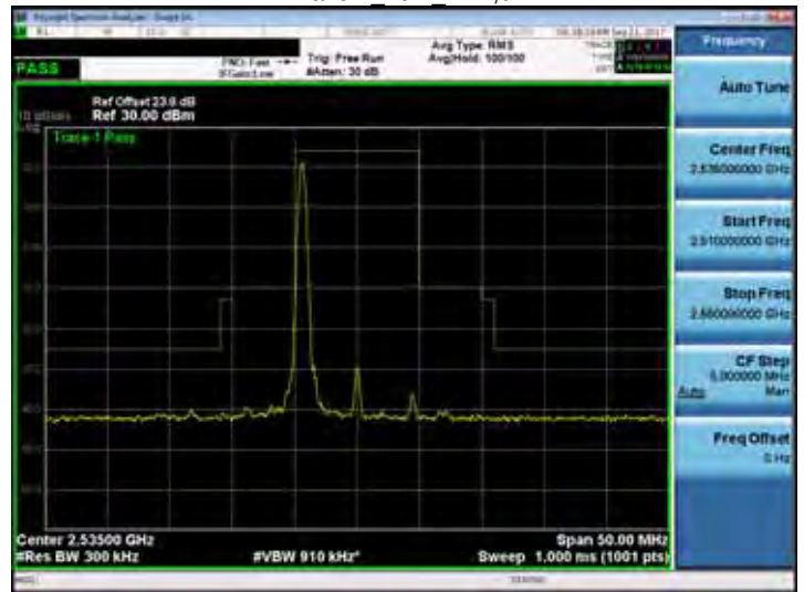
Band 7 10M RB1,49
