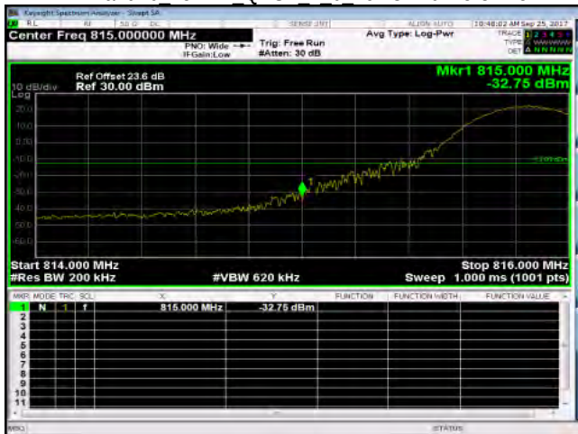
Band26 15MHz QPSK 1 0 LowCH26775-822.5
