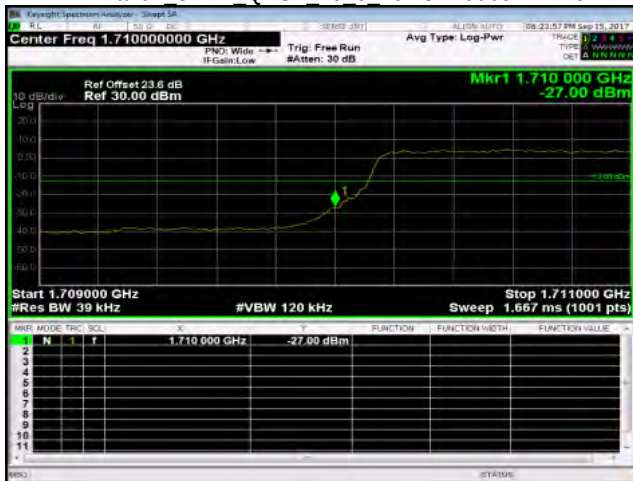
Band4 3MHz QPSK 15 0 LowCH19965-1711.5
