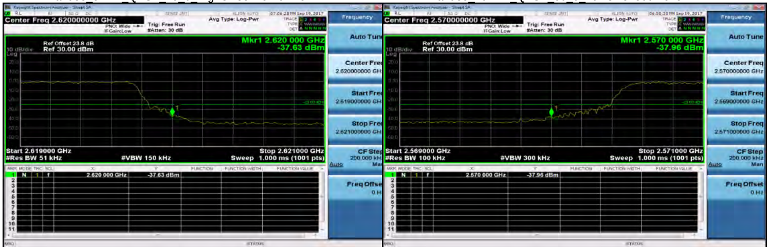
Band38 5MHz QPSK 25 0 HighCH38225-2617.5
