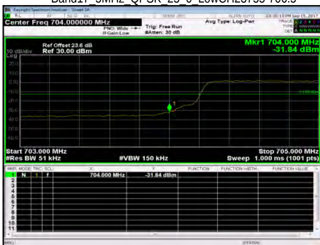
Band17 5MHz QPSK 25 0 LowCH23755-706.5
