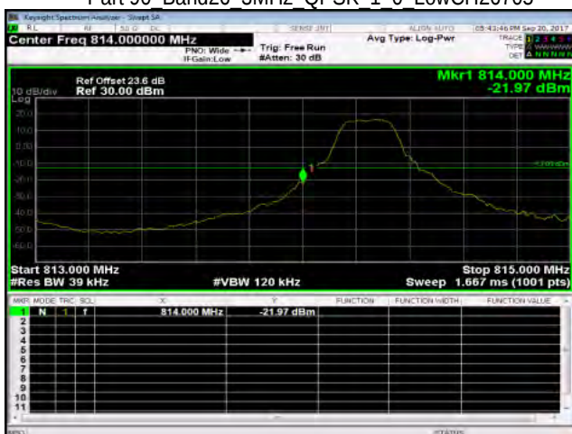
Part 90 Band26 3MHz QPSK 1 0 LowCH26705
