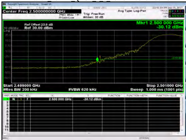
Band7 15MHz QPSK 1 0 LowCH20825-2507.5
