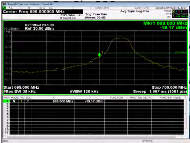
Band12 3MHz QPSK 1 0 LowCH23025-700.5
