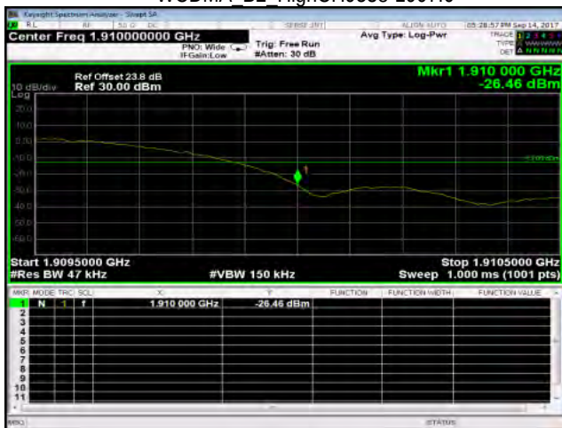
WCDMA B2 HighCH9538-1907.6
