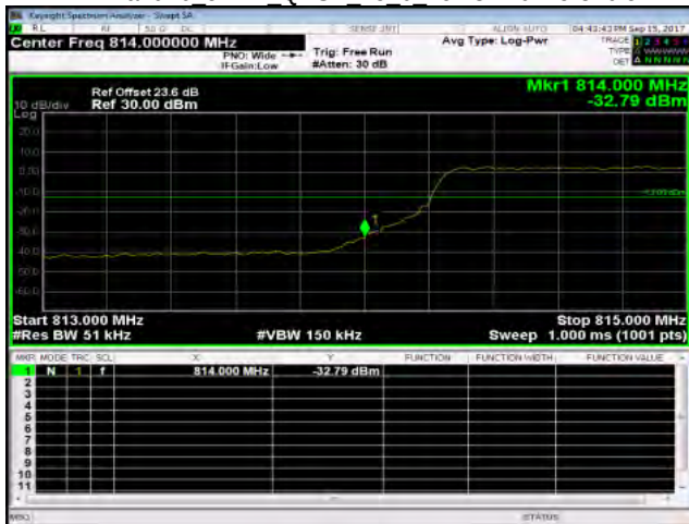
Band26 5MHz QPSK 25_0 LowCH26715-816.5
