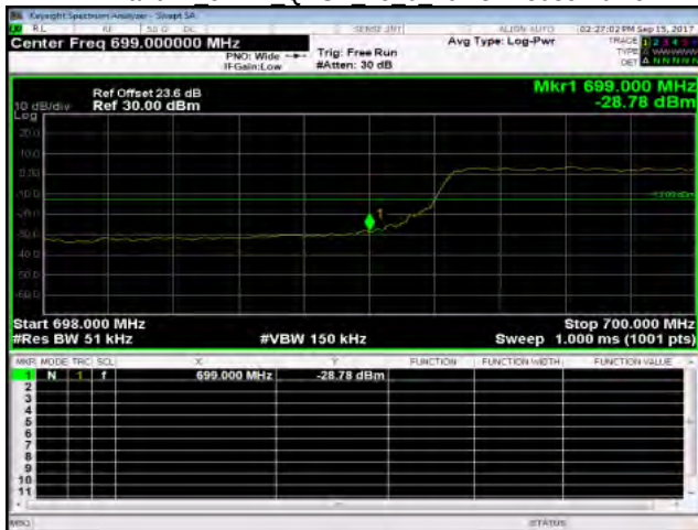
Band12 5MHz QPSK 25_0 LowCH23035-701.5
