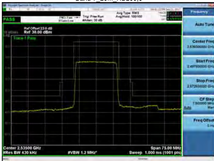
Band 7 20M RB100,0
