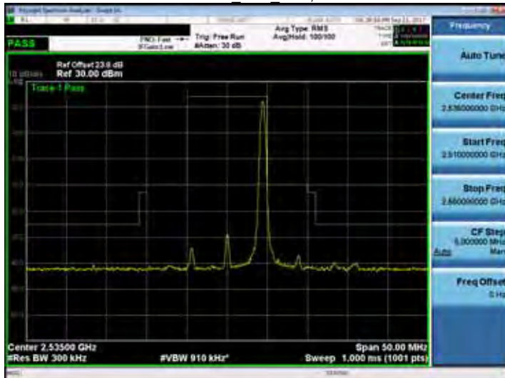
Band 7 10M RB50,0
