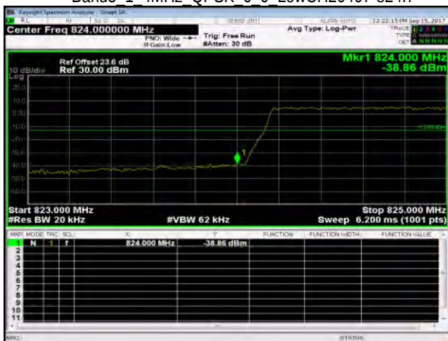
Band5 1 4MHz QPSK 6 0 LowCH20407-824.7
