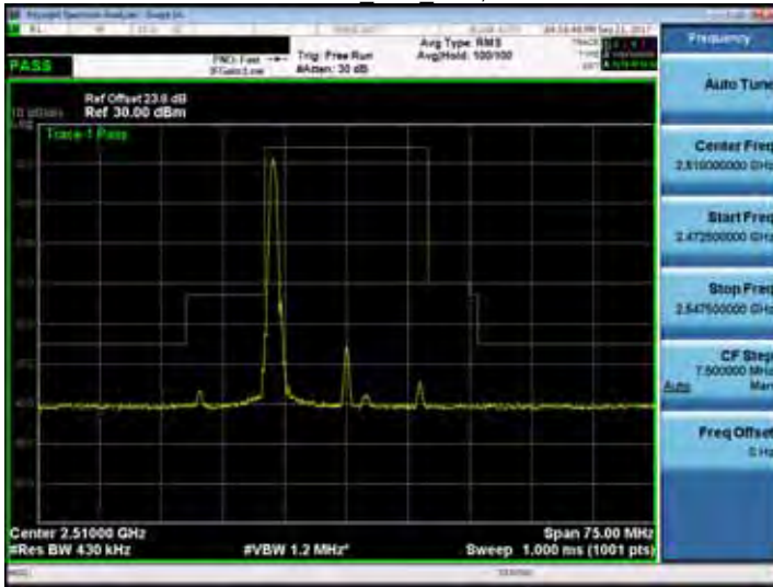
Band 7 20M RB1,99
