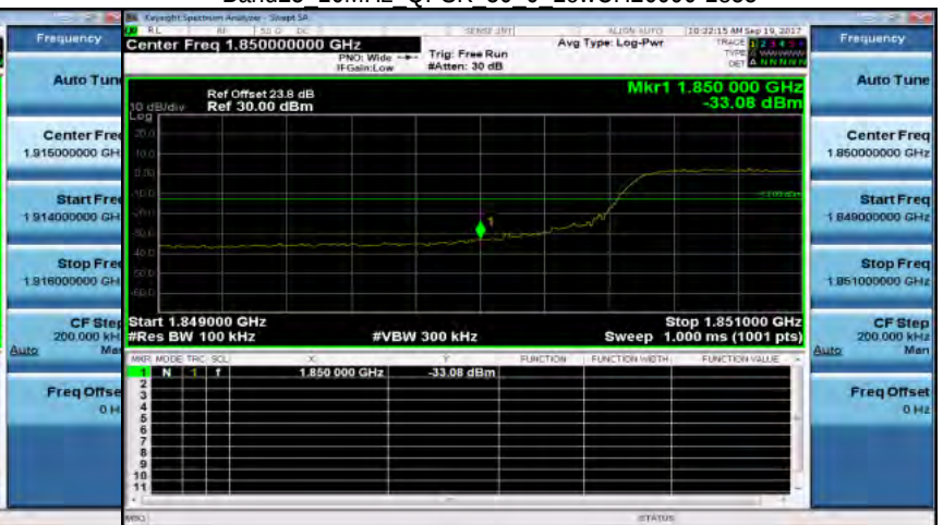
Band25 10MHz QPSK 50 0 LowCH26090-1855
