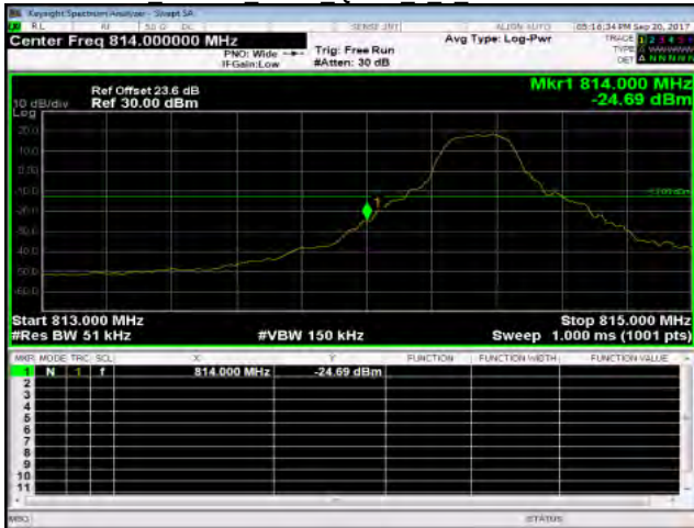
Part 90 Band26 5MHz QPSK 1 0 LowCH26715-816.5
