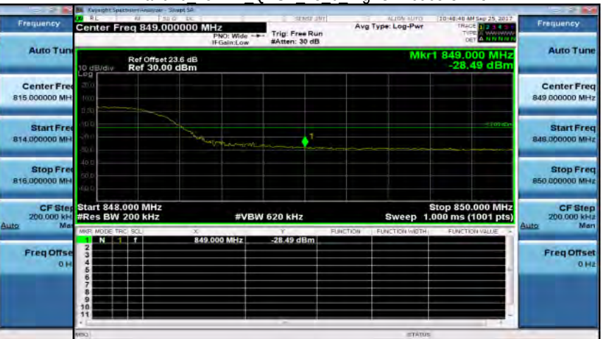
Band26 15MHz QPSK 75 0 HighCH26965-841.5
