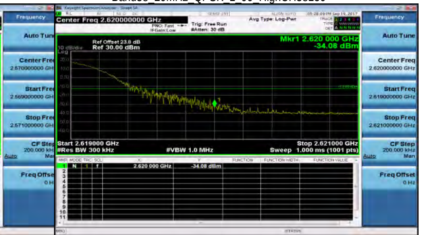
Band38 20MHz QPSK 1 99 HighCH38150
