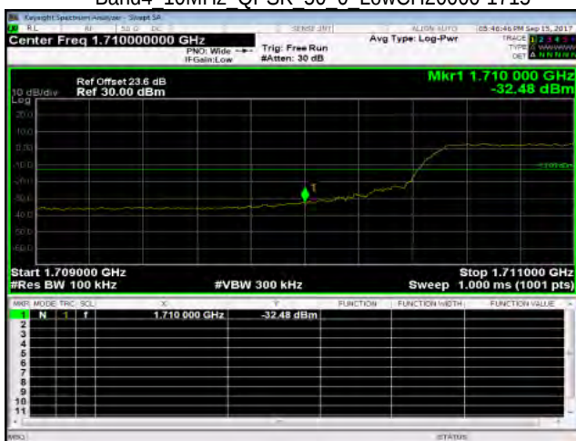
Band4 10MHz QPSK 50 0 LowCH20000-1715
