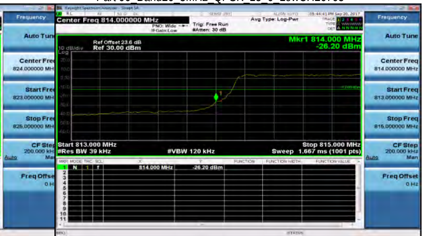
Part 90 Band26 3MHz QPSK 15 0 LowCH26705
