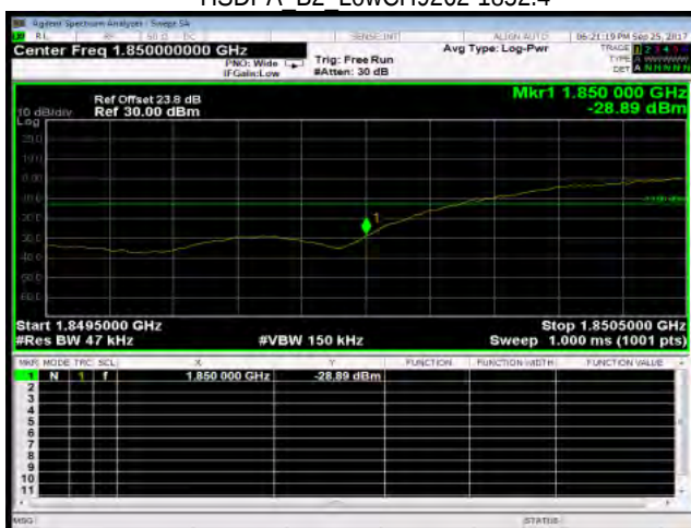
HSDPA B2 LowCH9262-1852.4
