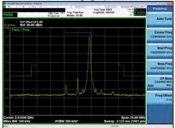
Band 7 5M RB25,0
