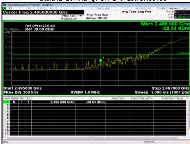
Band41 20MHz QPSK 1 0 LowCH39750
