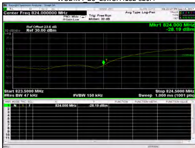
WCDMA B5 LowCH4132-826.4
