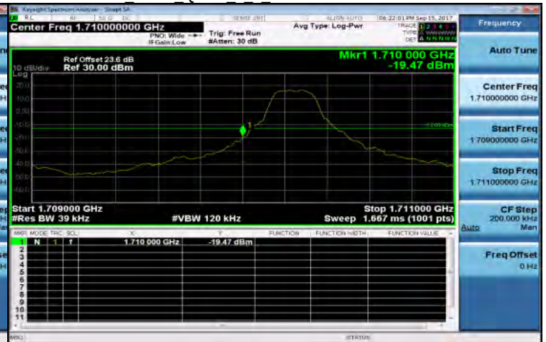
Band4 3MHz QPSK 1 0 LowCH19965-1711.5
