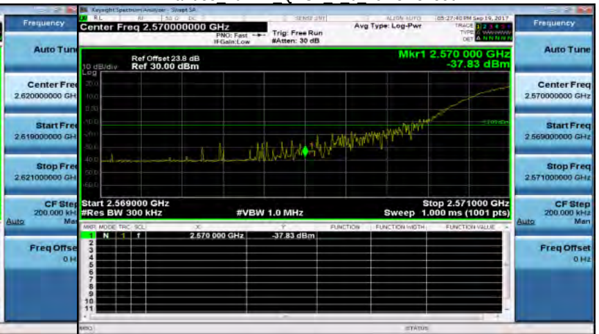
Band38 20MHz QPSK 1 0 LowCH37850
