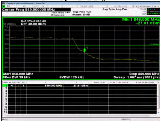
Band5 3MHz QPSK 15 0 HighCH20635-847.5
