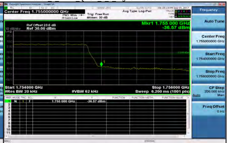
Band4 1 4MHz QPSK 6 0 HighCH20393-1754.3
