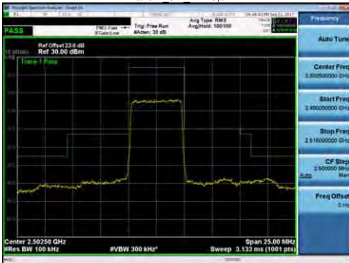
Band 7 5M RB25,0
