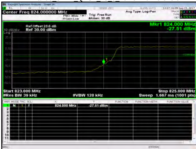
Band5 3MHz QPSK 15 0 LowCH20415-825.5
