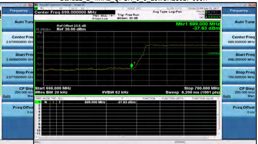
Band12 1 4MHz QPSK 6 0 LowCH23017-699.7
