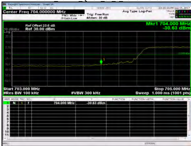
Band17 10MHz QPSK 50 0 LowCH23780-709
