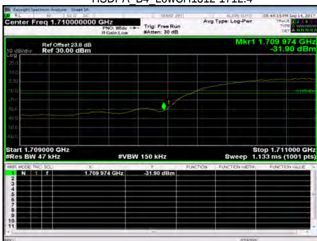
HSDPA B4 LowCH1312-1712.4
