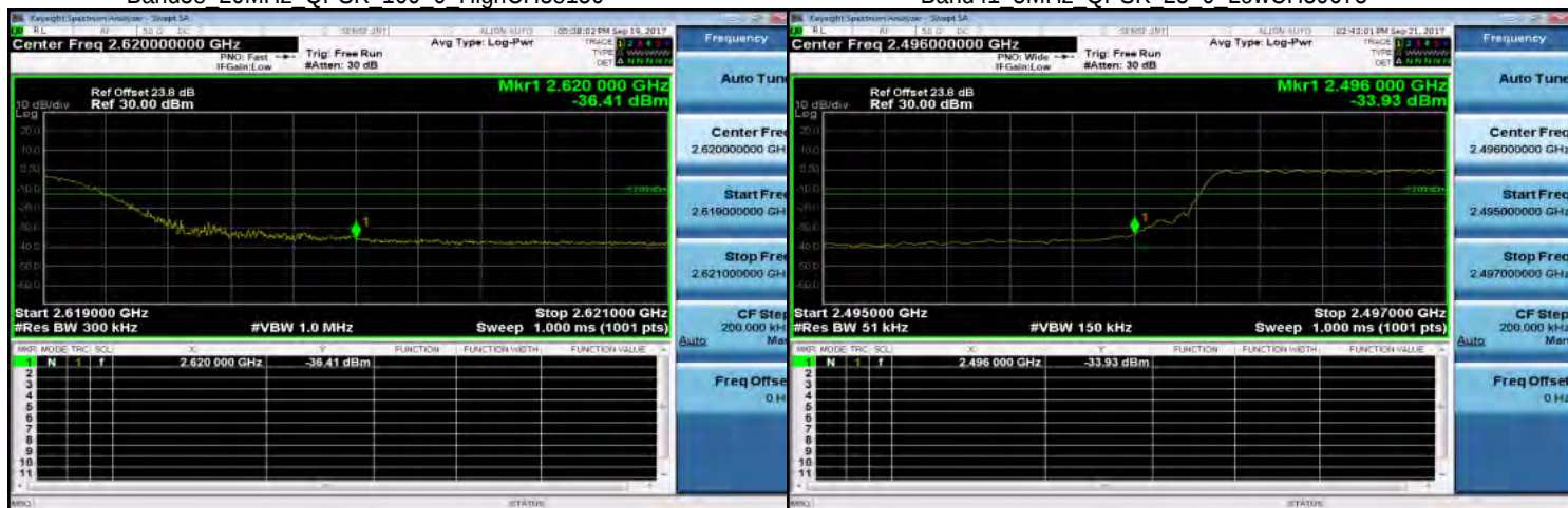
Band38 20MHz QPSK 100 0 HighCH38150
