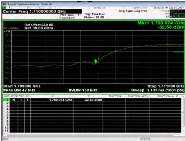
WCDMA B4 LowCH1312-1712.4
