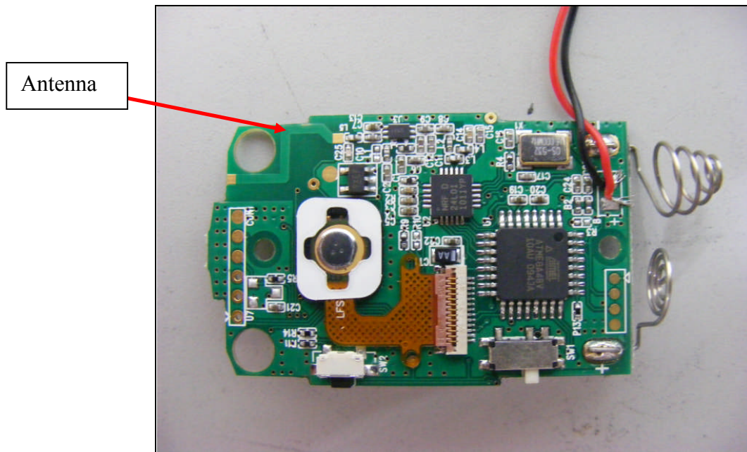
Bottom view of PCB
