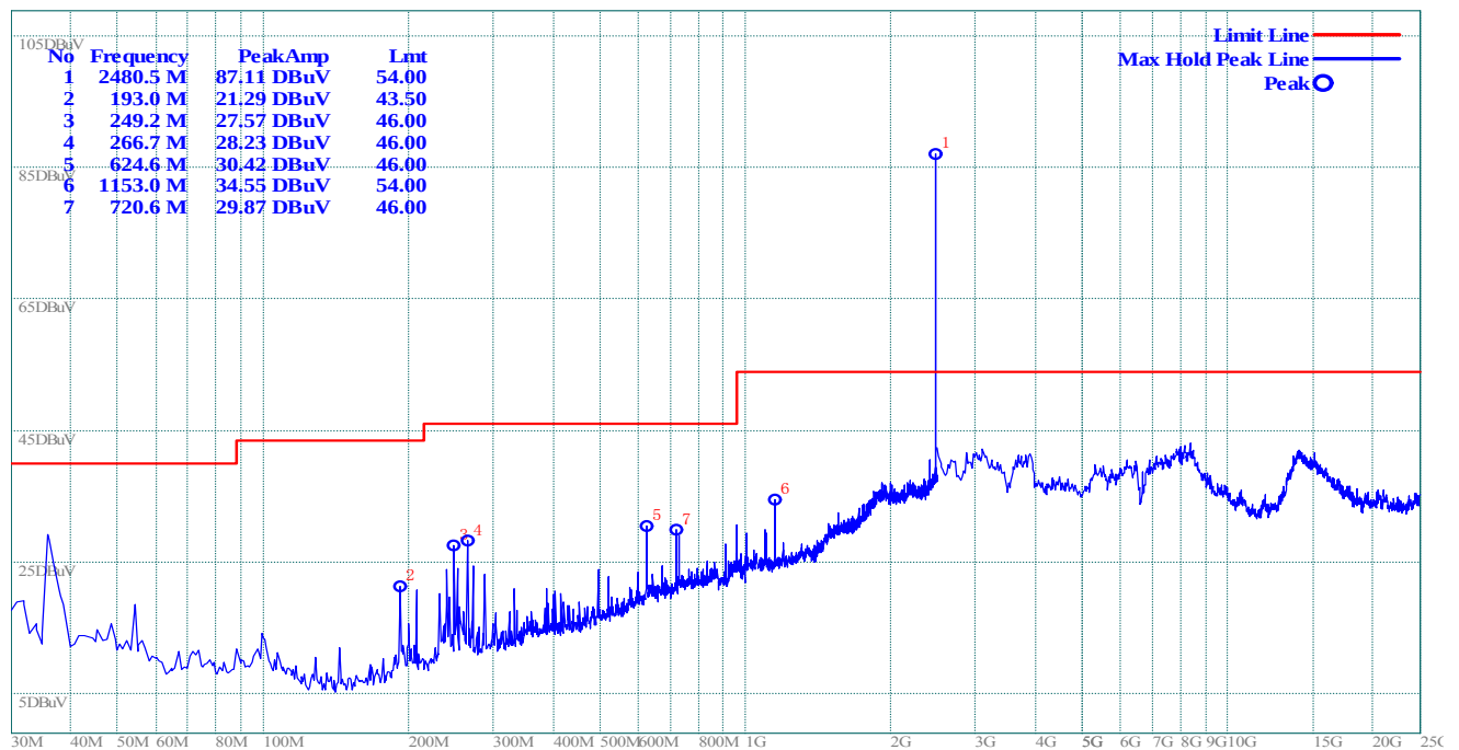
(Plot C.2: Antenna Vertical)
