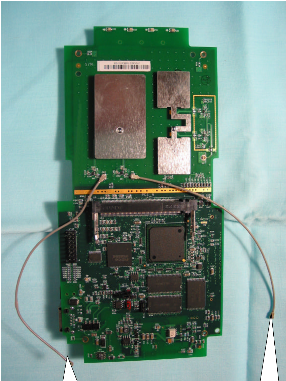
Coax to Ext 2.4 GHz antenna, Right
