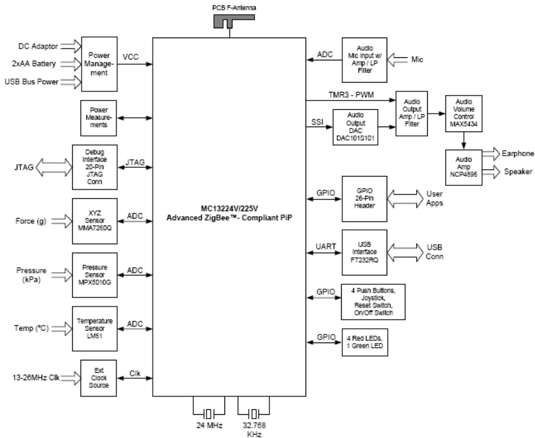
Figure 3-1. 1322x Sensor Node Block Diagram
