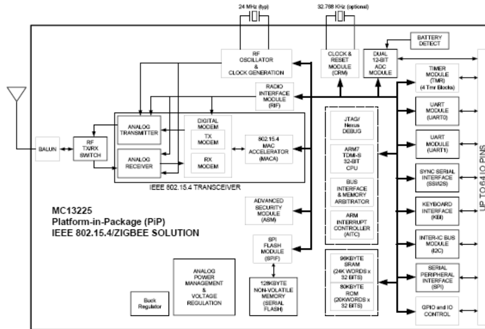
Figure 3-2. MC1322x Block Diagram
