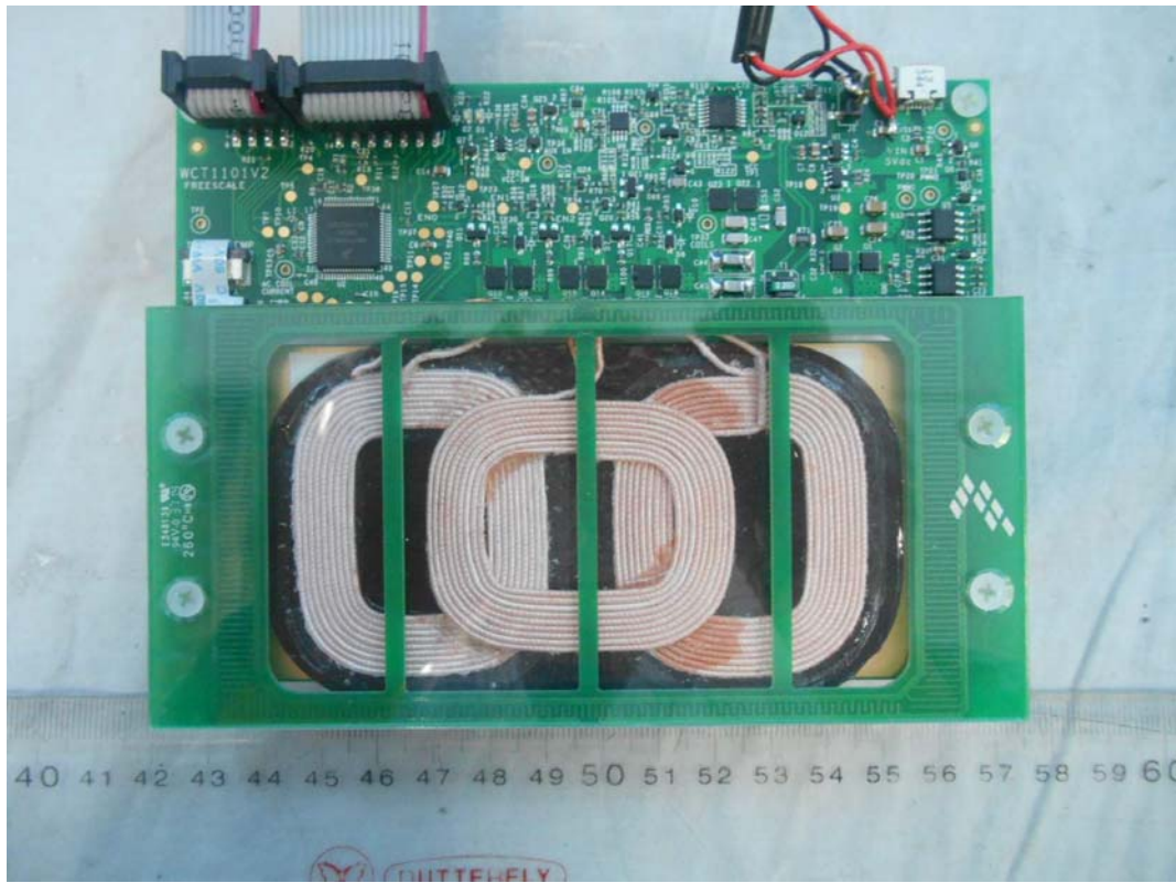
FIGURE 1 A28 MULTI-COIL WIRELESS CHARGER (M/N: WCT-5WTXMULTI) GENERAL APPEARANCE (FRONT VIEW)
