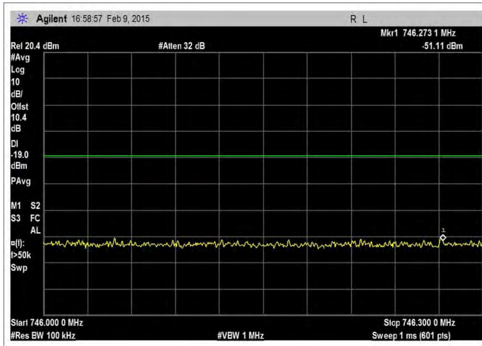
7.5_OBE_DL_728-746MHz_GSM_H_-20dBm
