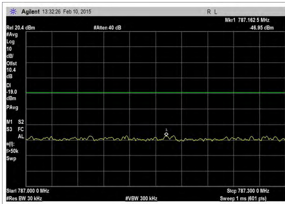
7.5_OBE_UL_776-787MHz_LTE_H_+10dBm
