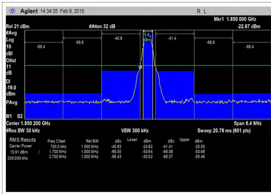
7.5_OBE_UL_1850-1915MHz_GSM_L_-17dBm
