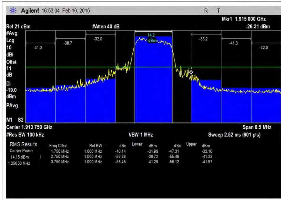
7.5_OBE_UL_1850-1915MHz_CDMA_H_-9dBm
