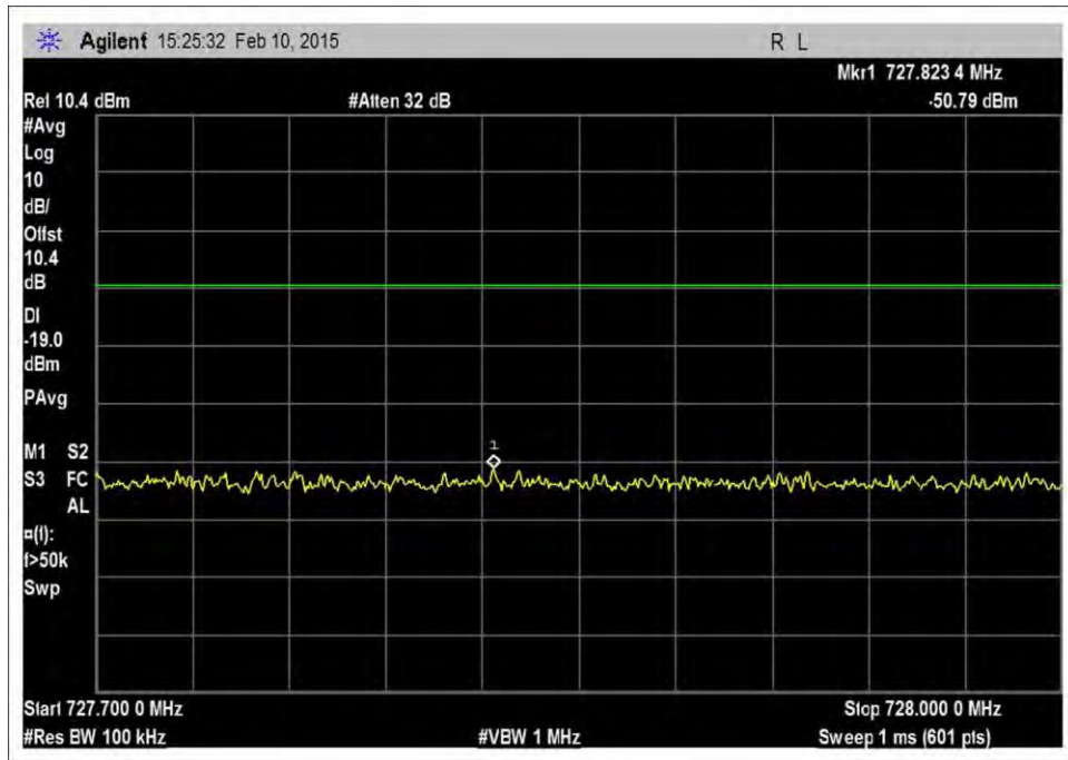
7.5_OBE_DL_728-746MHz_CDMA_L_-47dBm
