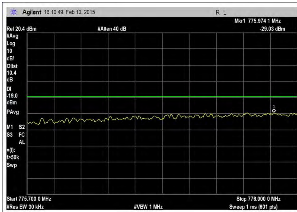
7.5_OBE_UL_776-787MHz_CDMA_L_-26dBm
