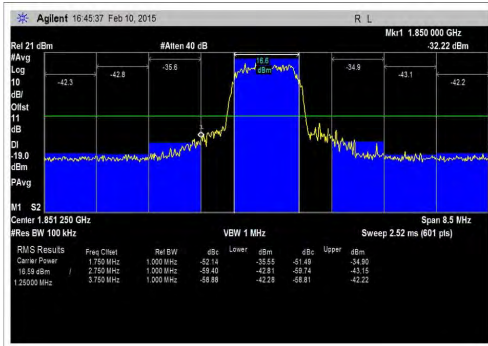
7.5_OBE_UL_1850-1915MHz_CDMA_L_-23dBm
