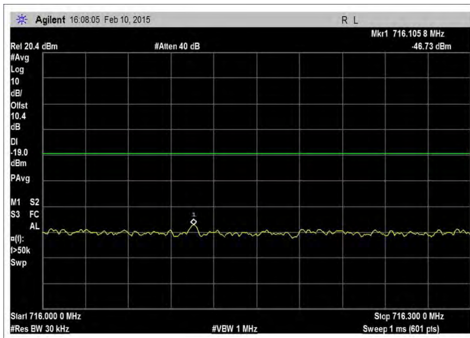
7.5_OBE_UL_698-716MHz_CDMA_H_+10dBm
