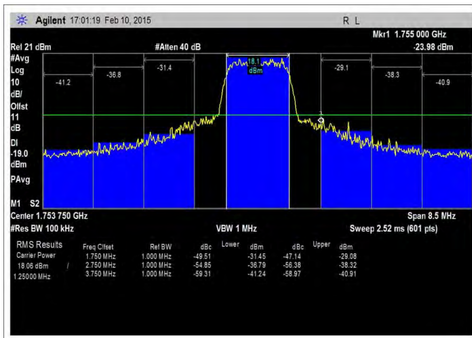
7.5_OBE_UL_1710-1755MHz_CDMA_H_-22dBm
