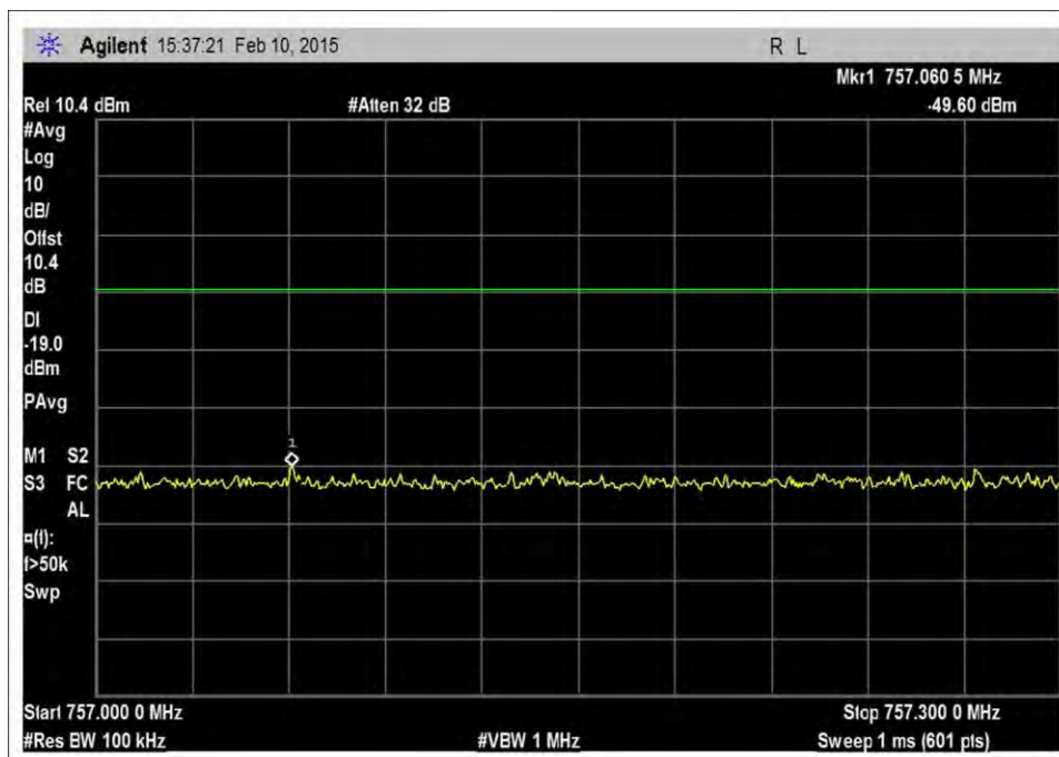
7.5_OBE_DL_746-757MHz_CDMA_H_-46dBm
