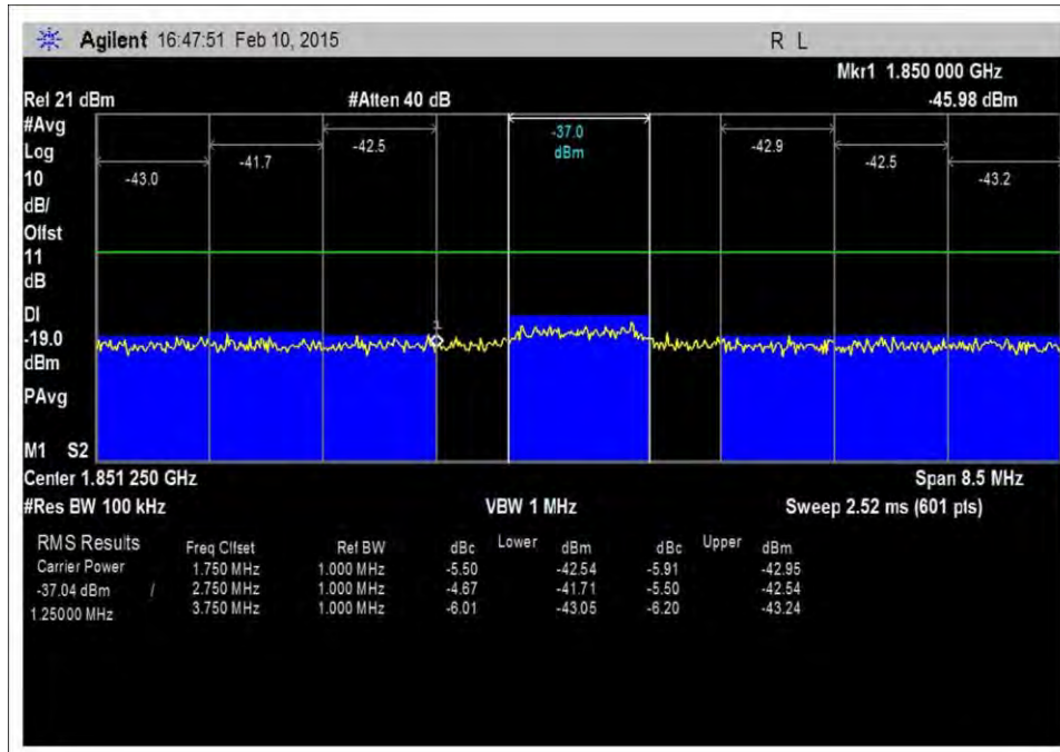
7.5_OBE_UL_1850-1915MHz_CDMA_L_+10dBm
