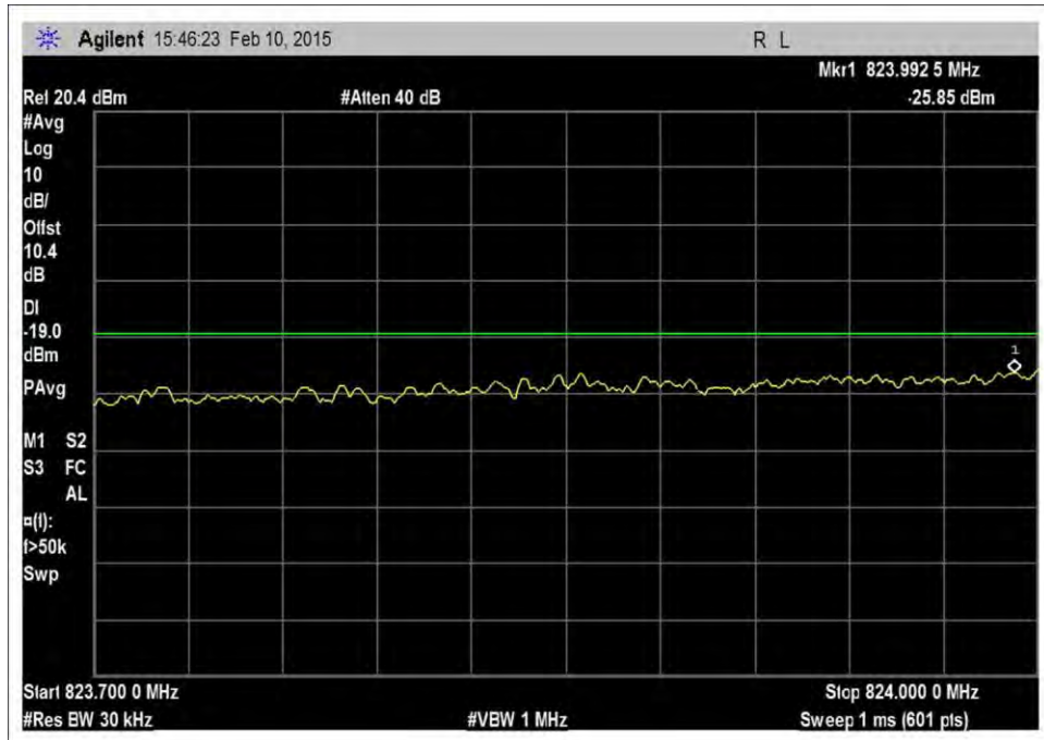
7.5_OBE_UL_824-835MHz_CDMA_L_-26dBm
