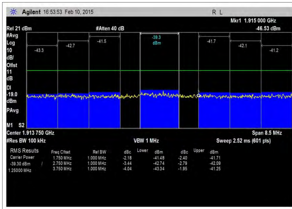
7.5_OBE_UL_1850-1915MHz_CDMA_H_+10dBm
