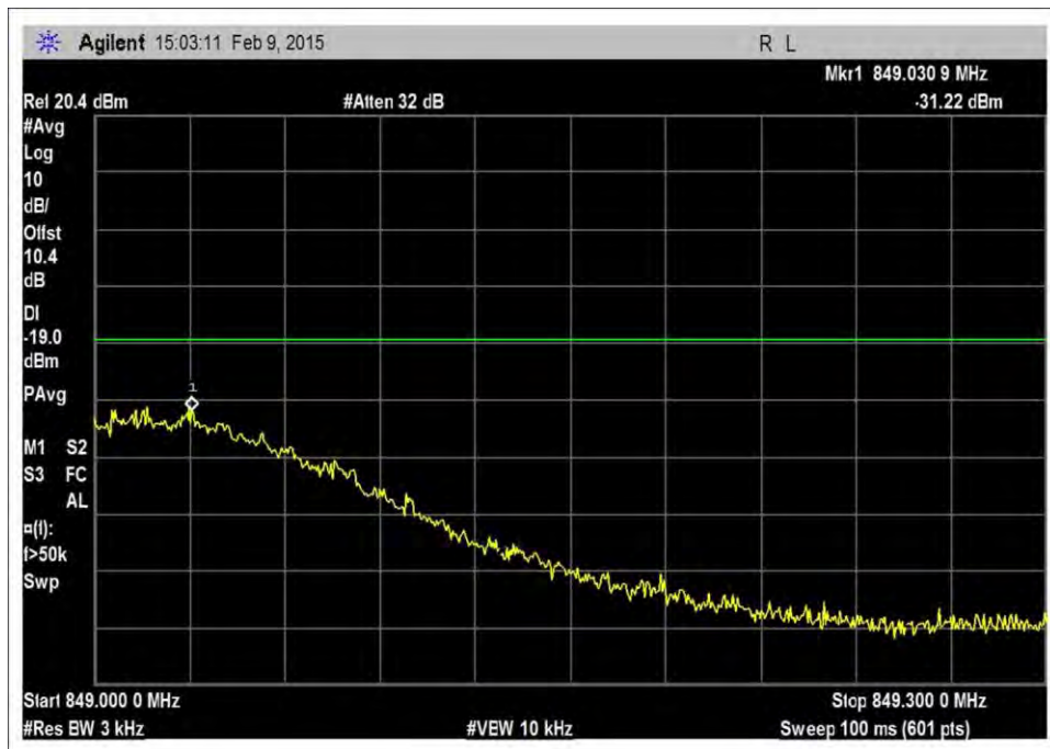
7.5_OBE_UL_824-849MHz_GSM_H_-27dBm
