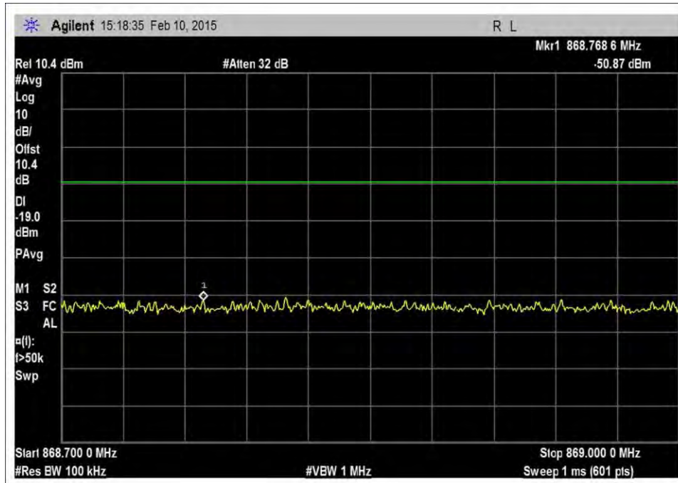
7.5_OBE_DL_869-880MHz_CDMA_L_-20dBm
