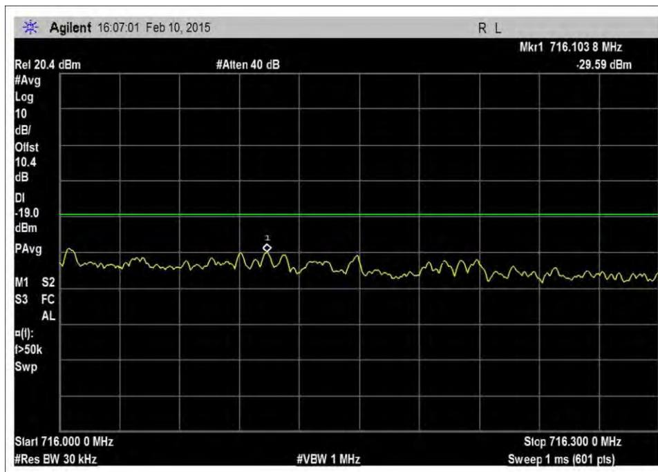
7.5_OBE_UL_698-716MHz_CDMA_H_-17dBm
