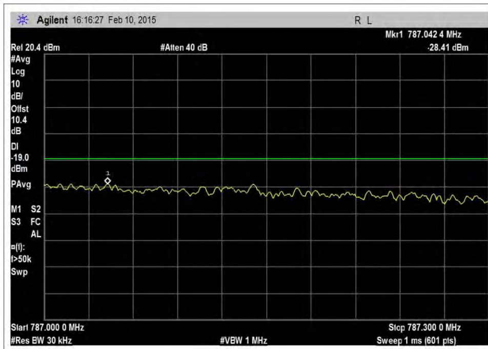
7.5_OBE_UL_776-787MHz_CDMA_H_-22dBm
