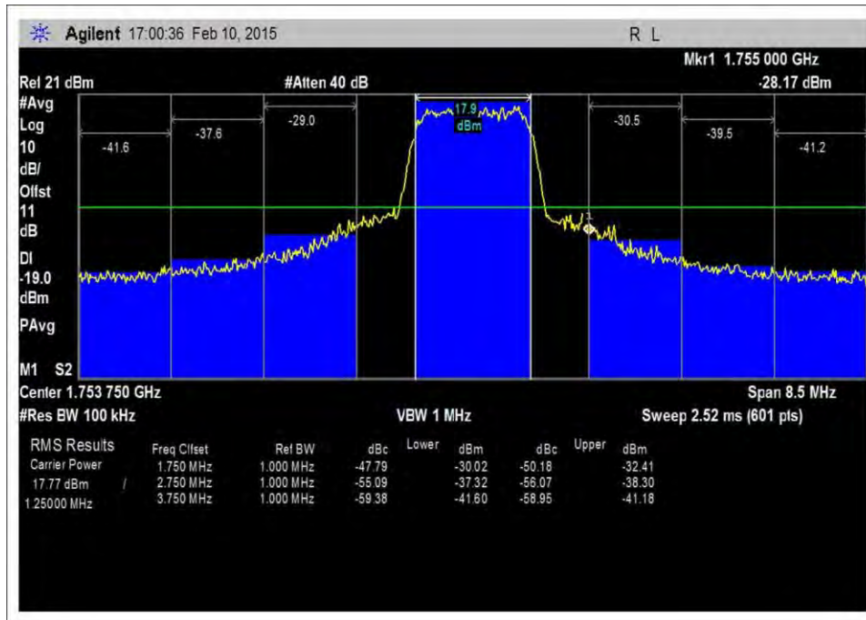
7.5_OBE_UL_1710-1755MHz_CDMA_H_-24dBm
