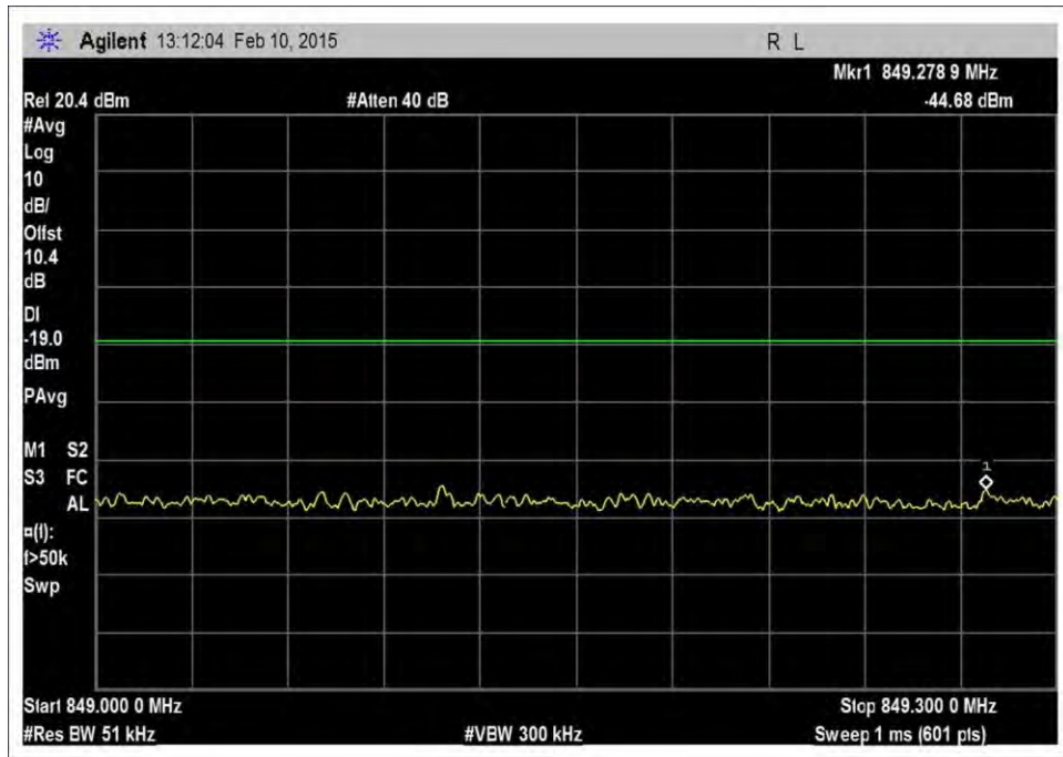
7.5_OBE_UL_824-849MHz_LTE_H_+10dBm
