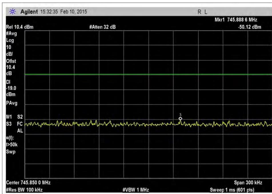
7.5_OBE_DL_746-757MHz_CDMA_L_-56dBm
