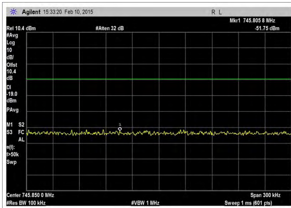
7.5_OBE_DL_746-757MHz_CDMA_L_-49dBm
