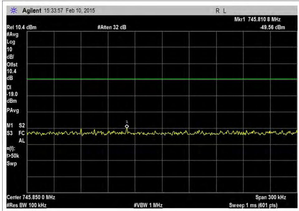
7.5_OBE_DL_746-757MHz_CDMA_L_-20dBm
