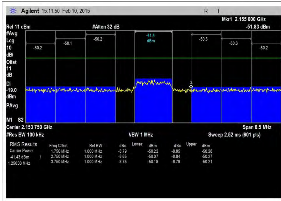
7.5_OBE_DL_2110-2155MHz_CDMA_H_-20dBm
