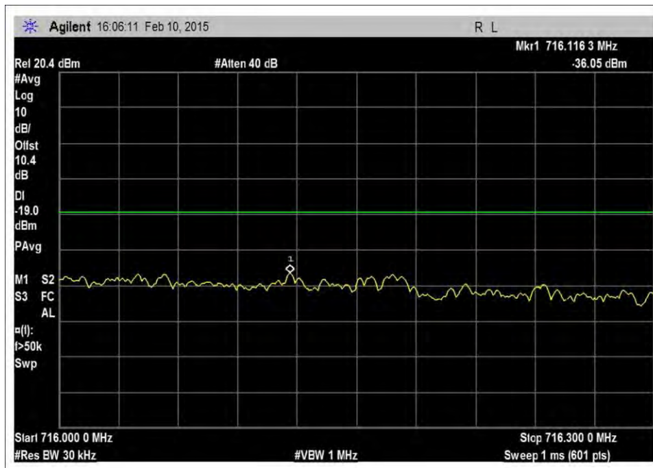
7.5_OBE_UL_698-716MHz_CDMA_H_-24dBm
