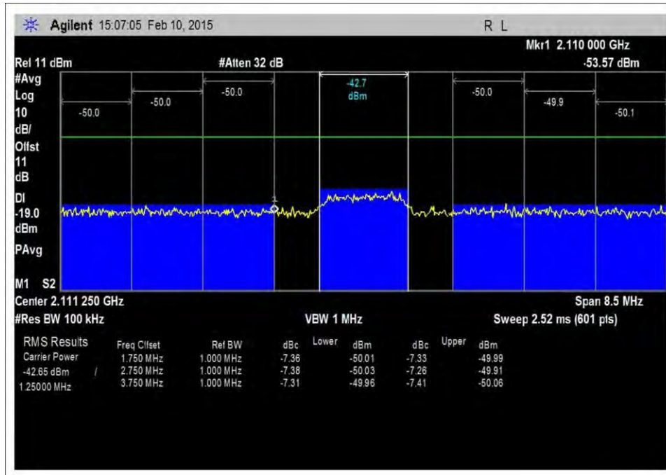
7.5_OBE_DL_2110-2155MHz_CDMA_L_-20dBm
