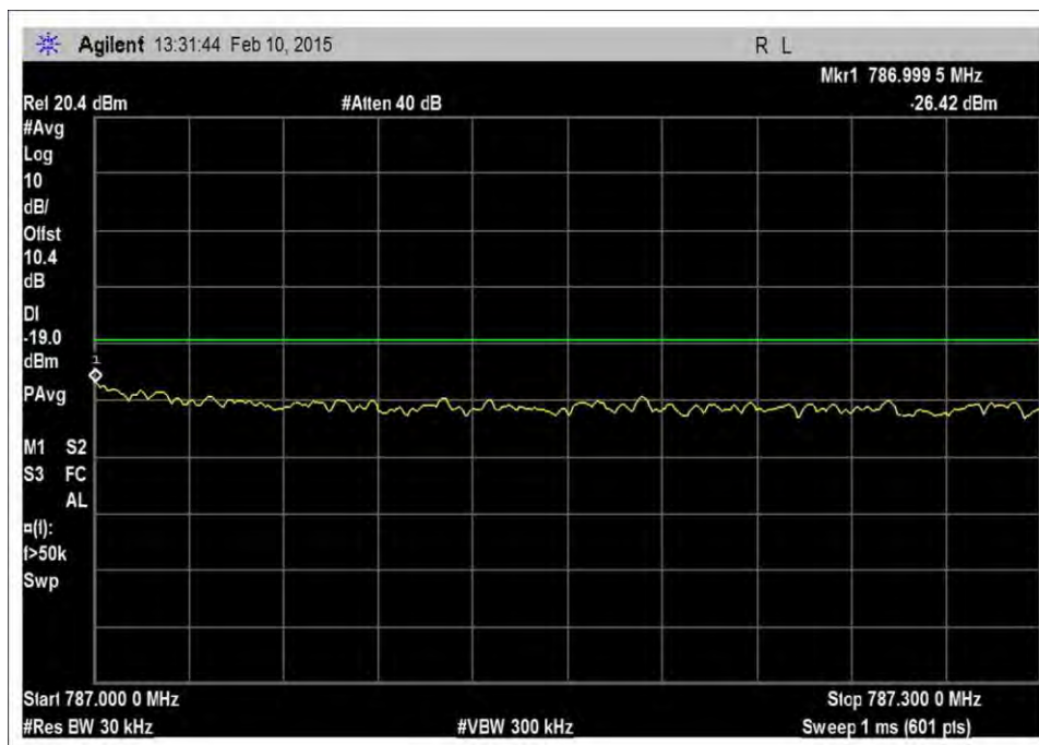
7.5_OBE_UL_776-787MHz_LTE_H_-22dBm
