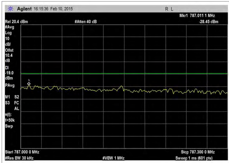
7.5_OBE_UL_776-787MHz_CDMA_H_-27dBm
