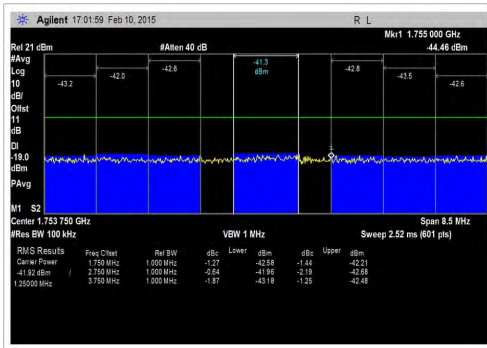
7.5_OBE_UL_1710-1755MHz_CDMA_H_+10dBm
