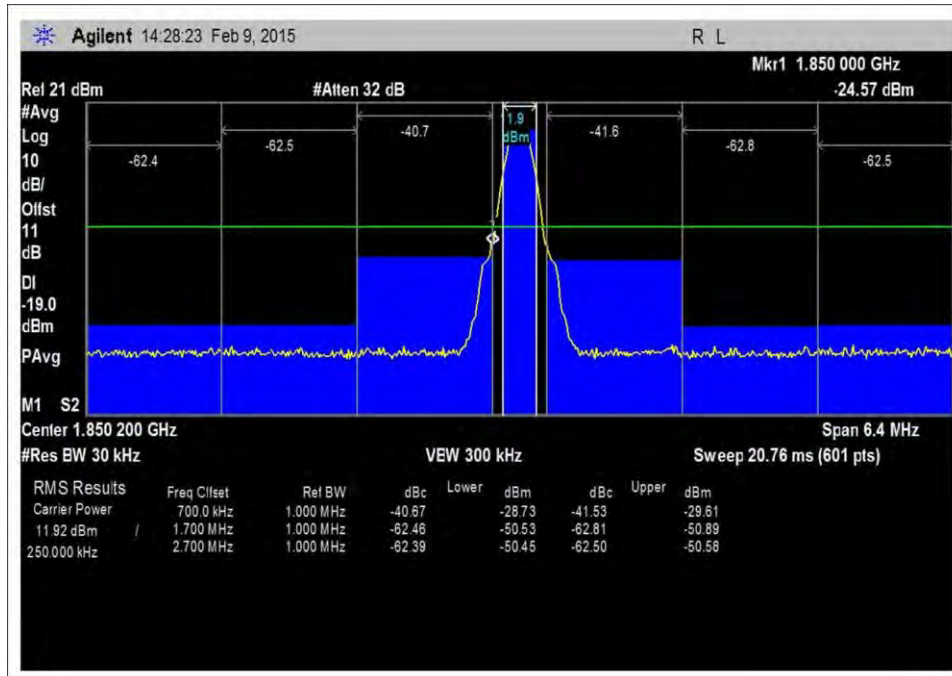
7.5_OBE_UL_1850-1915MHz_GSM_L_-27dBm
