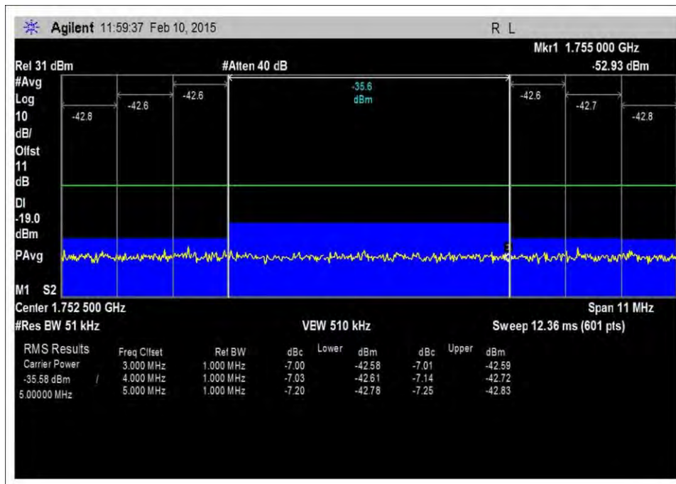
7.5_OBE_UL_1710-1755MHz_LTE_H_+10dBm
