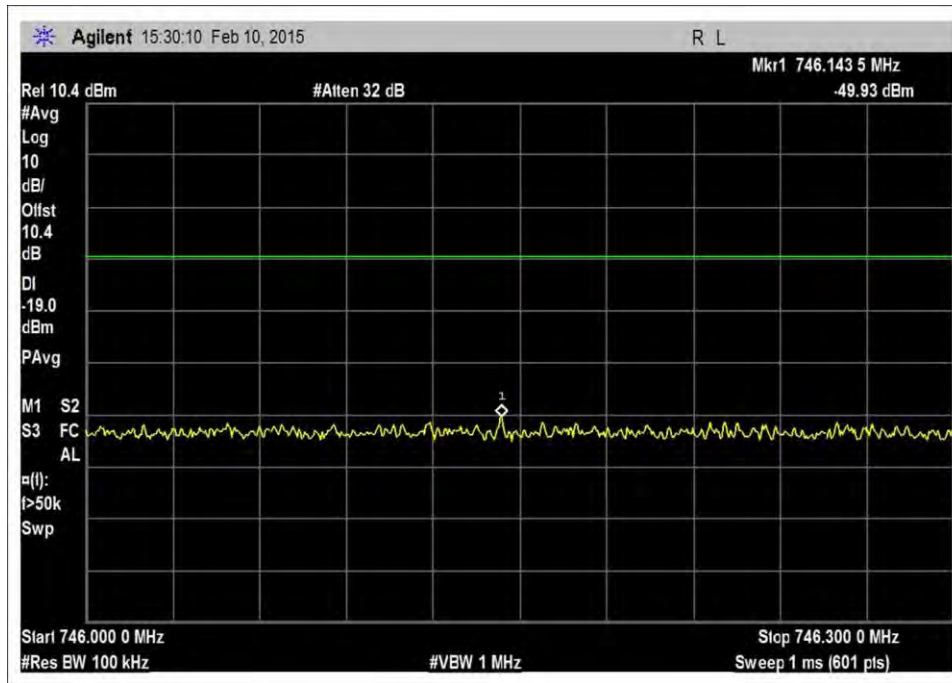
7.5_OBE_DL_728-746MHz_CDMA_H_-20dBm
