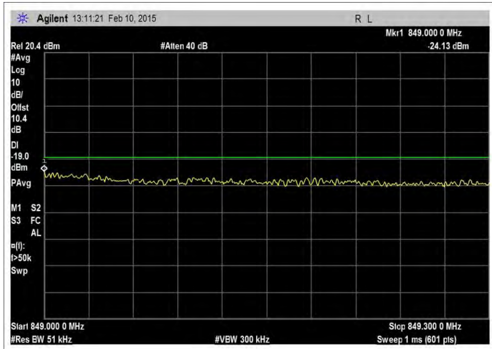
7.5_OBE_UL_824-849MHz_LTE_H_-22dBm
