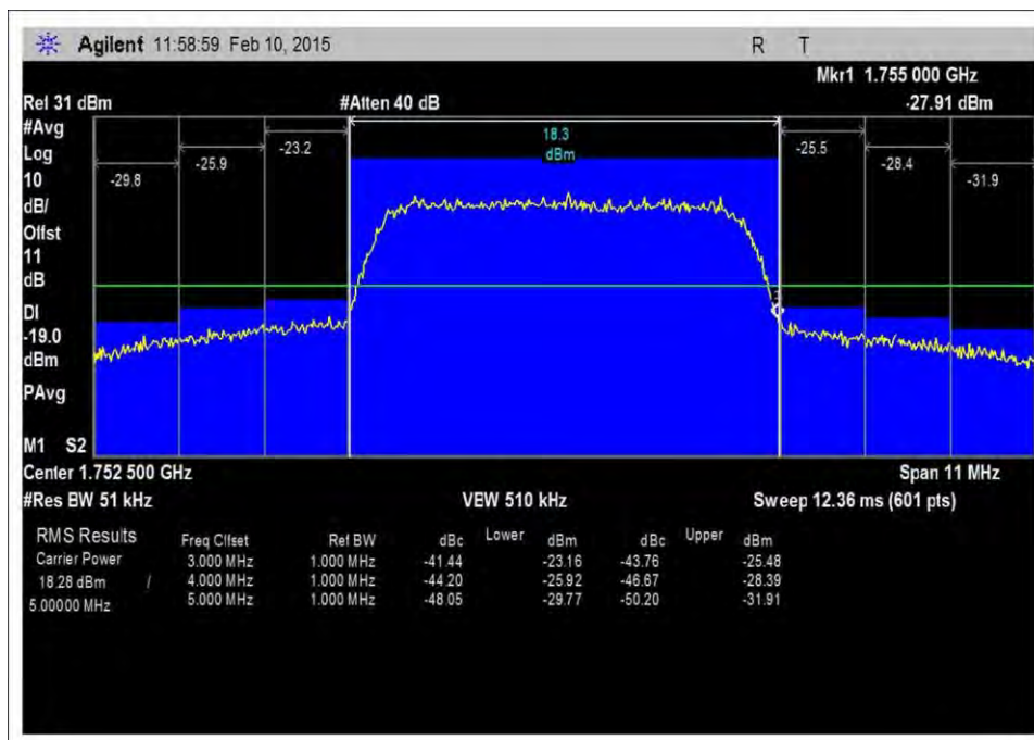
7.5_OBE_UL_1710-1755MHz_LTE_H_-20dBm
