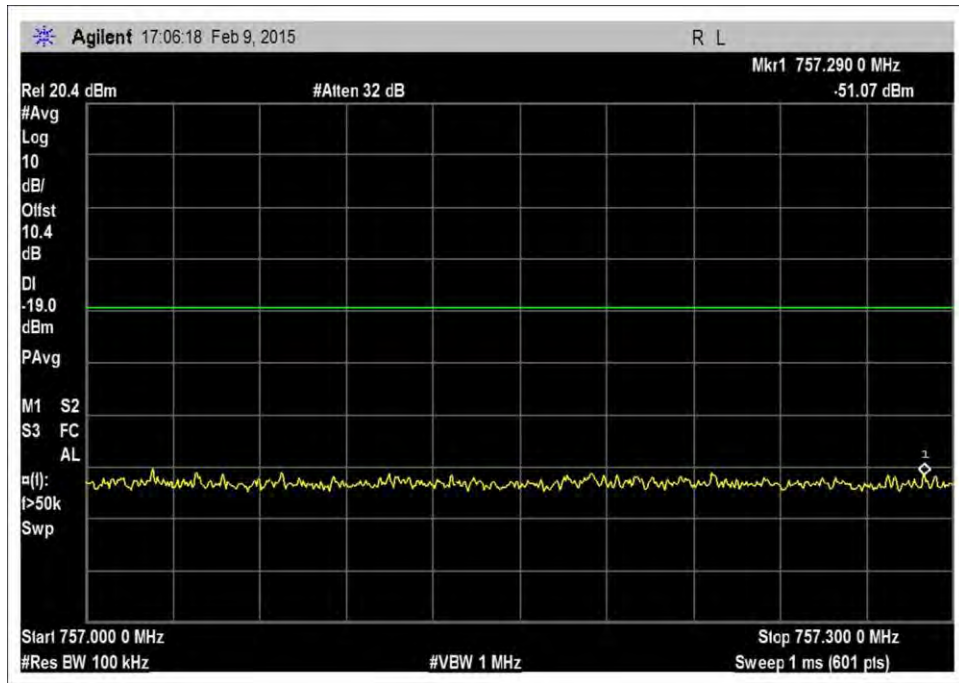
7.5_OBE_DL_746-757MHz_GSM_H_-20dBm
