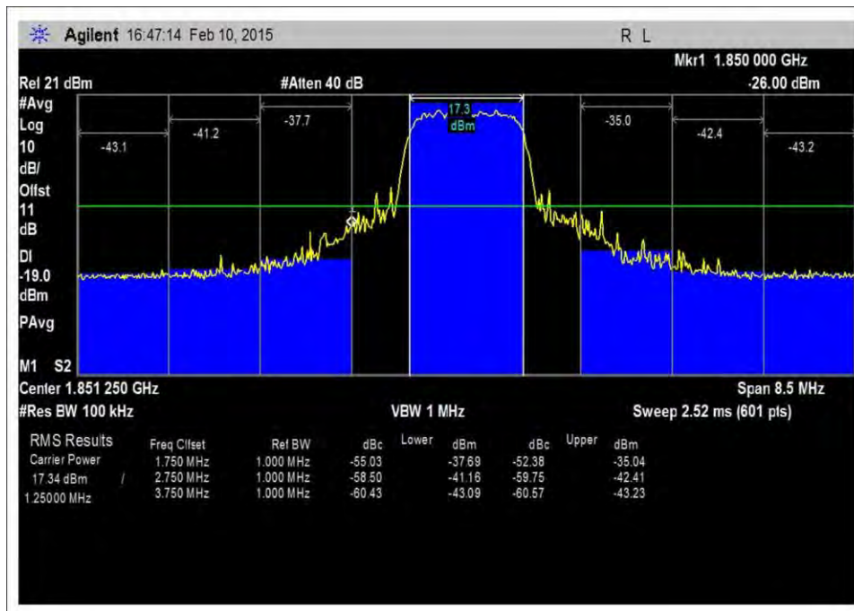
7.5_OBE_UL_1850-1915MHz_CDMA_L_-17dBm
