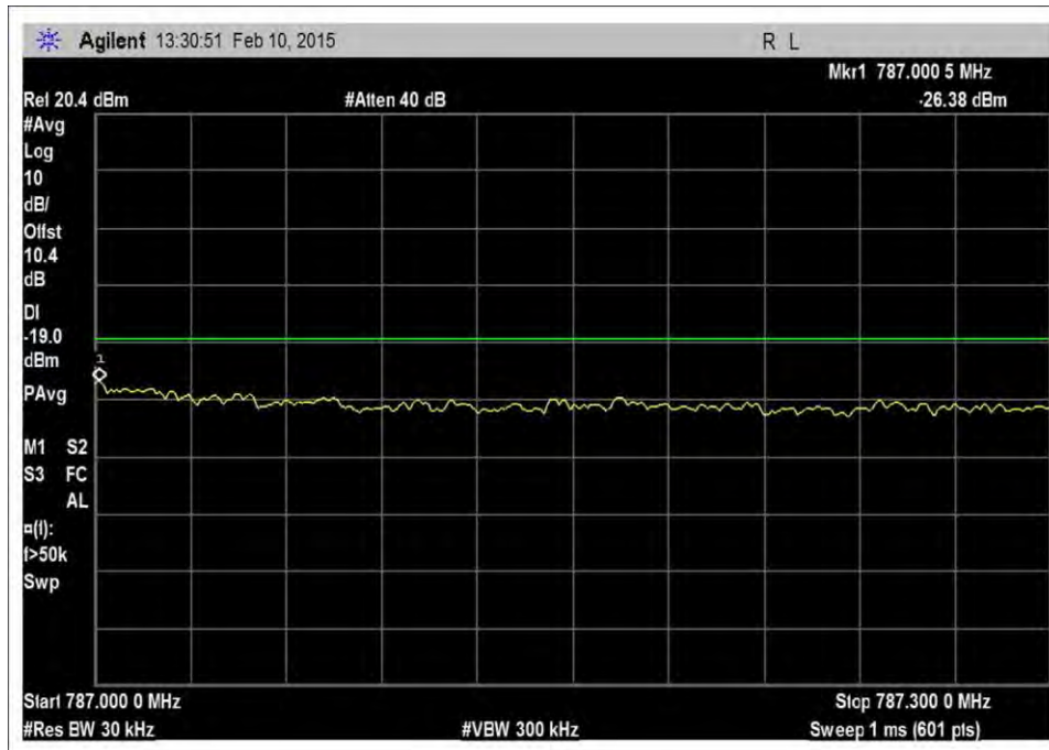
7.5_OBE_UL_776-787MHz_LTE_H_-26dBm
