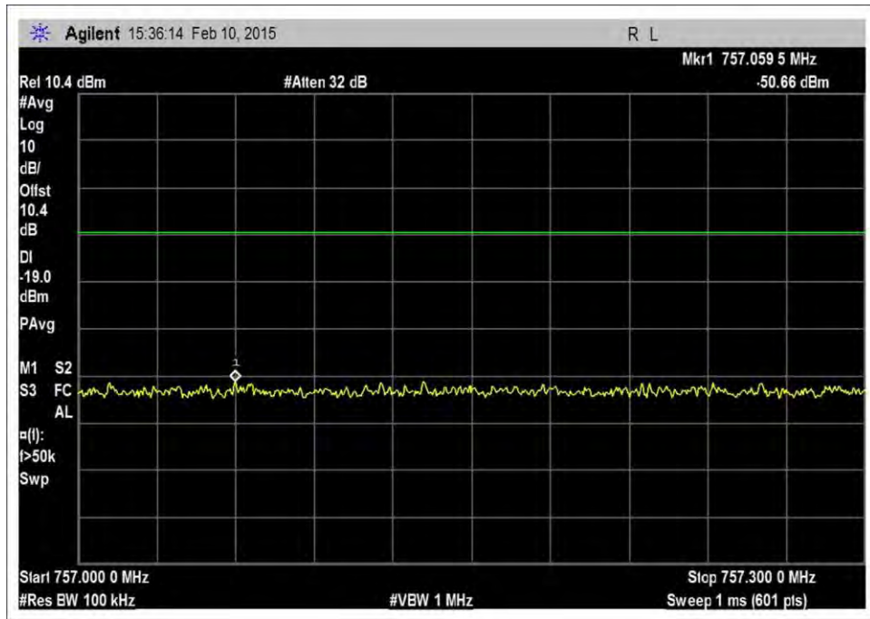
7.5_OBE_DL_746-757MHz_CDMA_H_-56dBm
