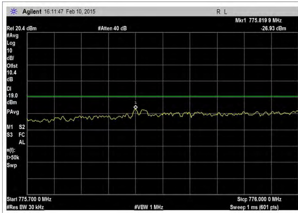
7.5_OBE_UL_776-787MHz_CDMA_L_-20dBm
