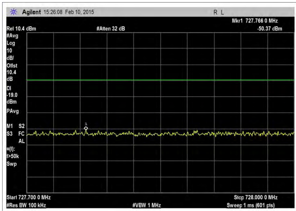
7.5_OBE_DL_728-746MHz_CDMA_L_-20dBm
