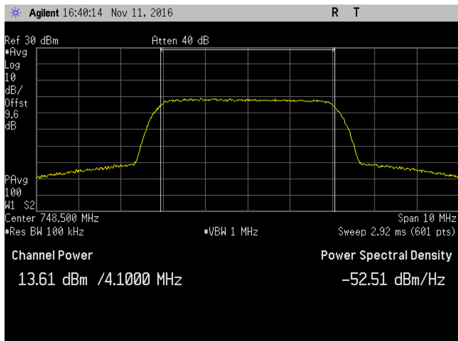
7.2_Power_DL_746-757MHz_AWGN_Max
