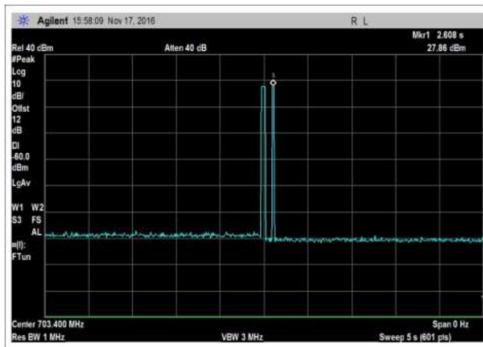
7.11_osc_UL-698-716MHz-Pk
