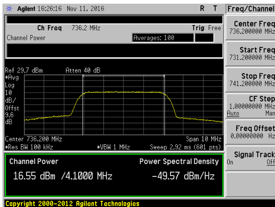
7.2_Power_DL_728-746MHz_AWGN
