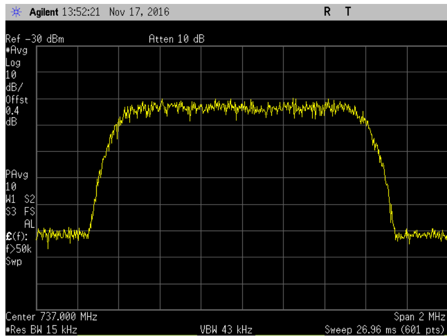
7.10_OBW_DL_728-746MHz_CDMA_In
