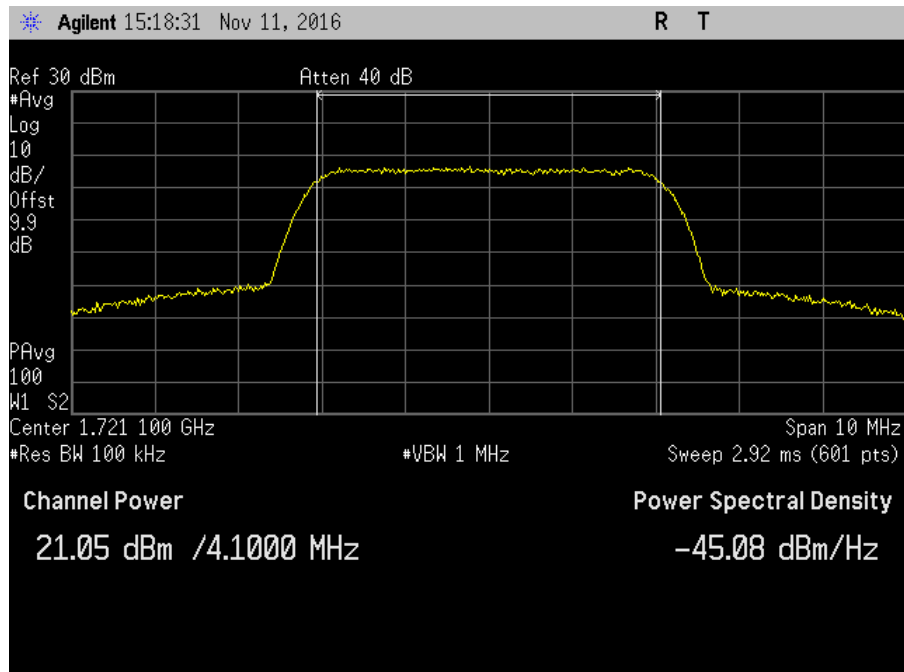
7.2_Power_UL_1710-1755MHz_AWGN_Max
