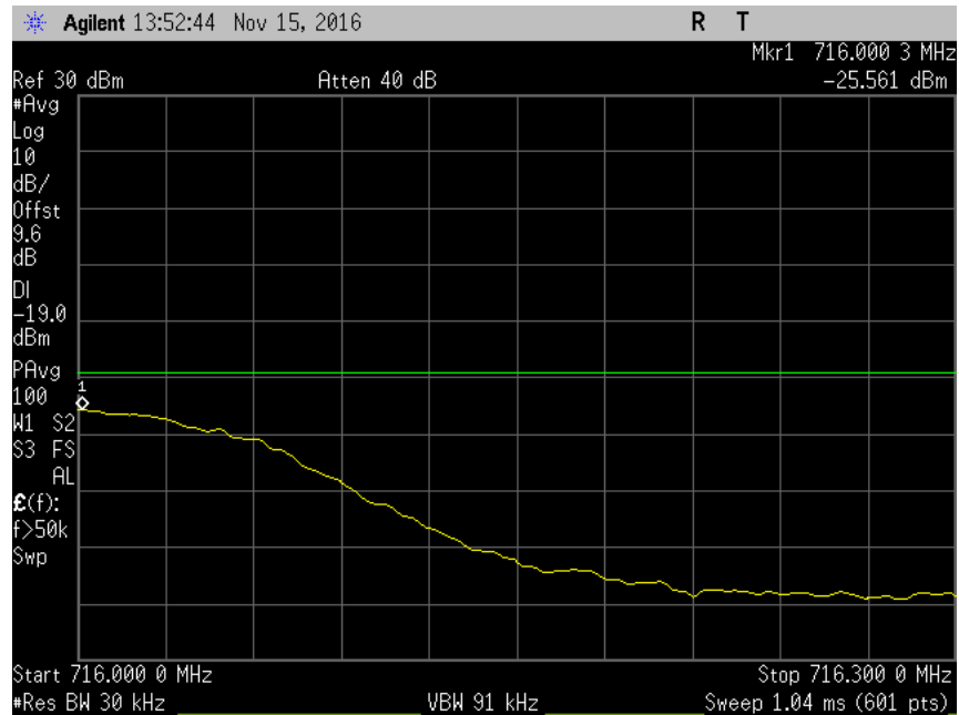
7.5_OBE_UL_698-716MHz_H_PreAGC_GSM
