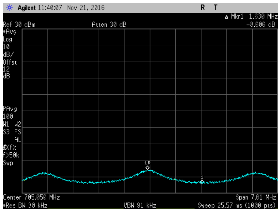
7.11.3_Osc_UL_698-716MHz+5_AWGNR
