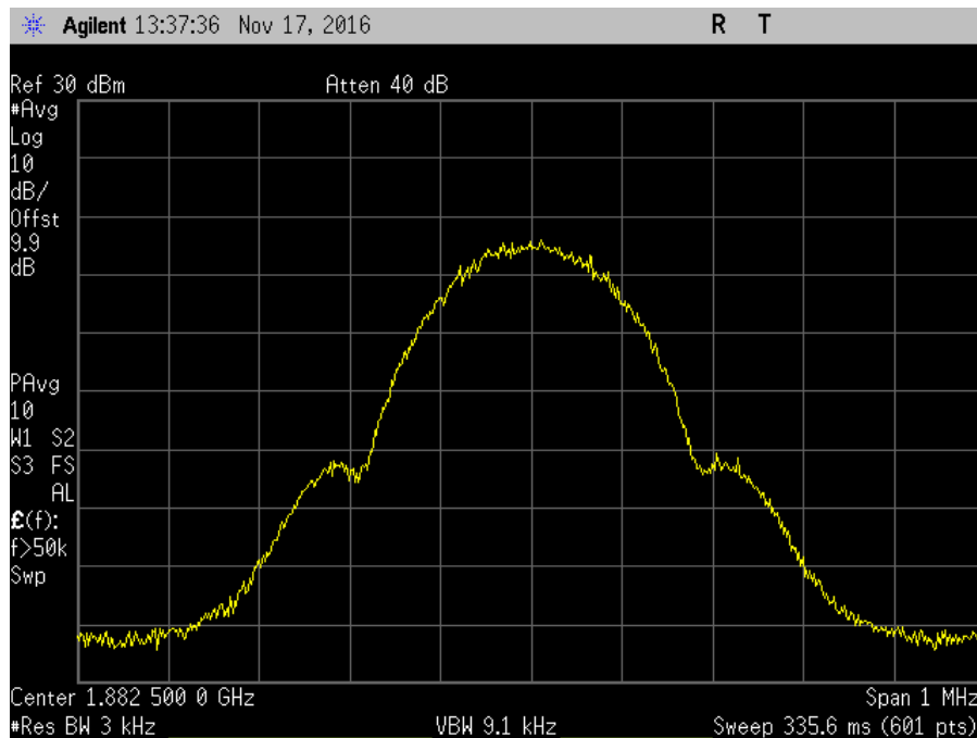
7.10_OBW_UL_1850-1915MHz_GSM_Out
