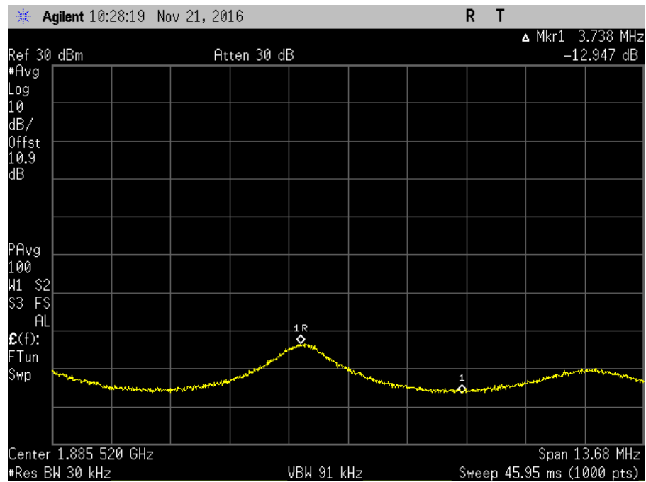
7.11.3_Osc_UL_1850-1915MHz+4_AWGNL
