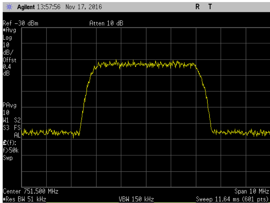
7.10_OBW_DL_746-757MHz_WCDMA_In
