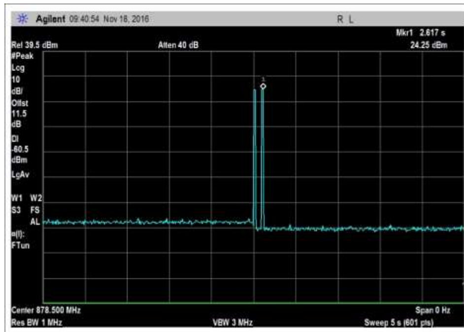
7.11_osc_DL-869-894MHz-Pk
