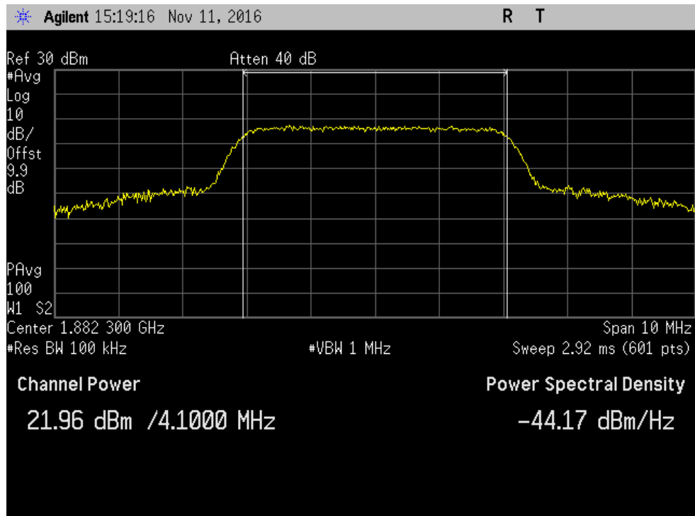
7.2_Power_UL_1850-1915MHz_AWGN_Max
