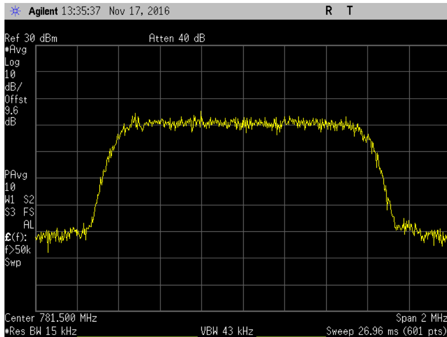
7.10_OBW_UL_776-787MHz_CDMA_Out
