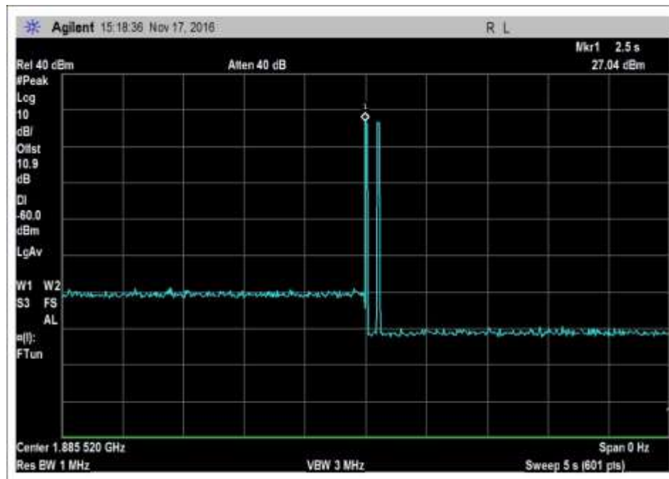
7.11_osc_UL-1850-1915MHz-Pk
