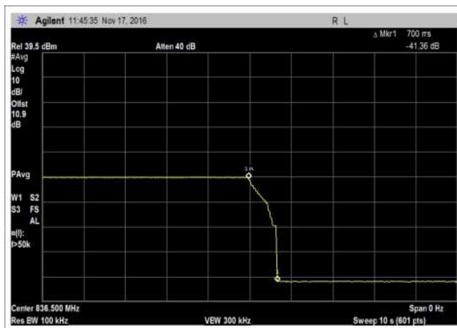
7.9.2_VarULGainTiming_UL_824-849MHz
