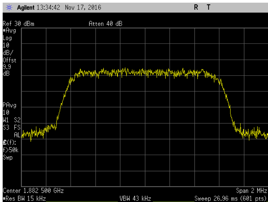
7.10_OBW_UL_1850-1915MHz_CDMA_Out
