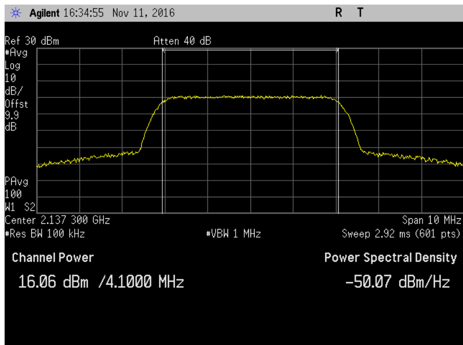
7.2_Power_DL_2110-2155MHz_AWGN_Max
