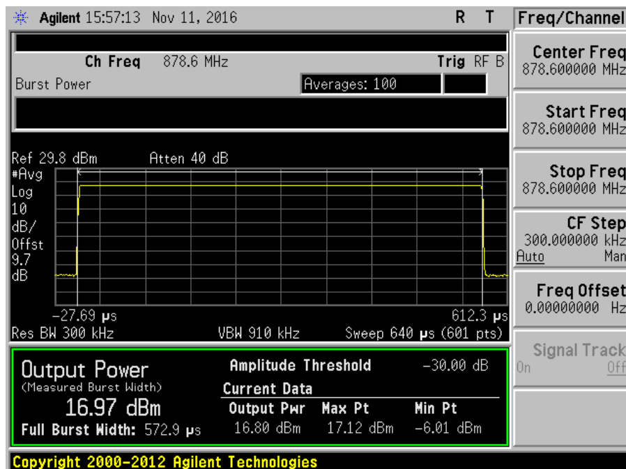
7.2_Power_DL_869-894MHz_GSM_Max
