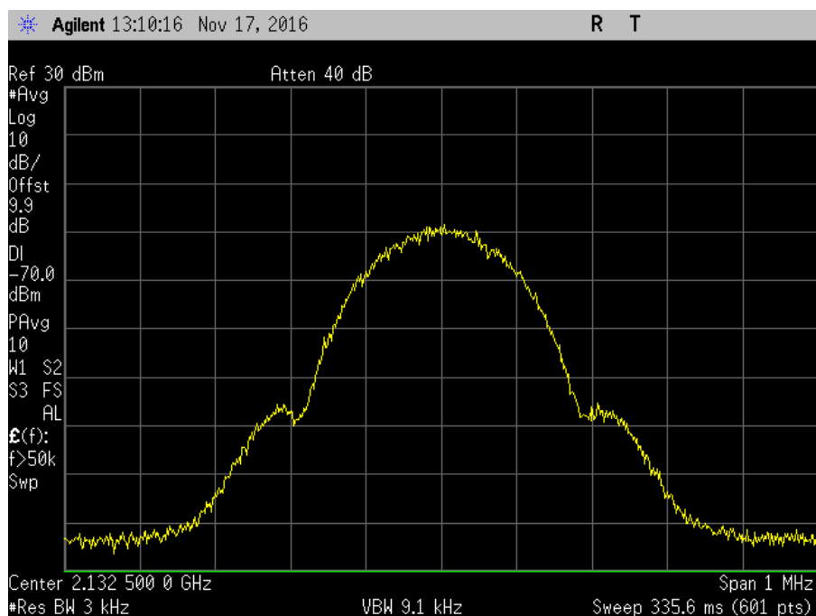
7.10_OBW_DL_2110-2155MHz_GSM_Out
