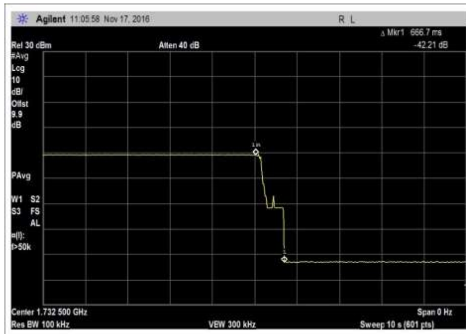
7.9.2_VarULGainTiming_UL_1710-1755MHz
