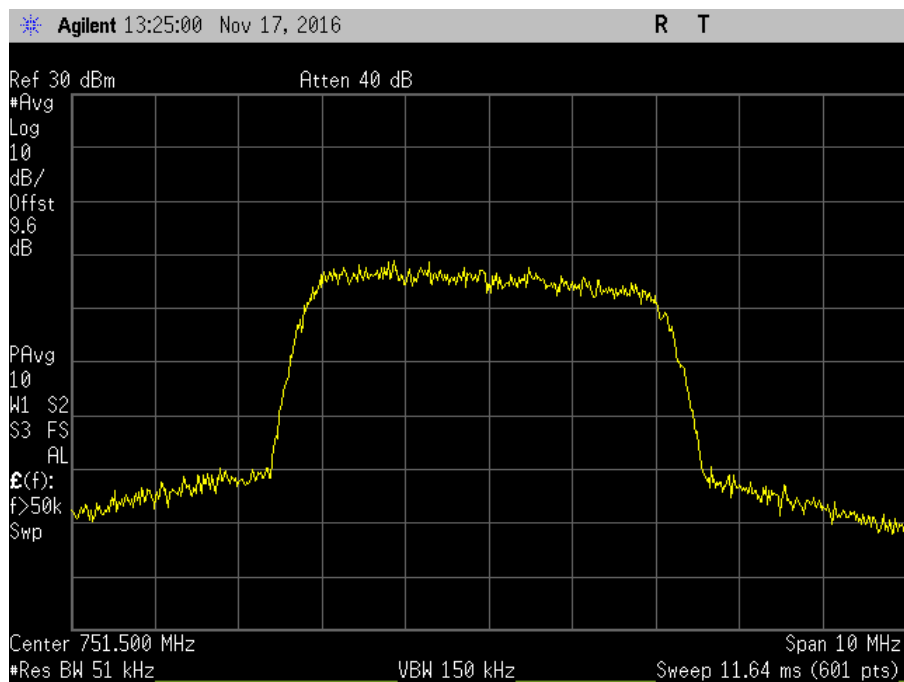
7.10_OBW_DL_746-757MHz_WCDMA_Out
