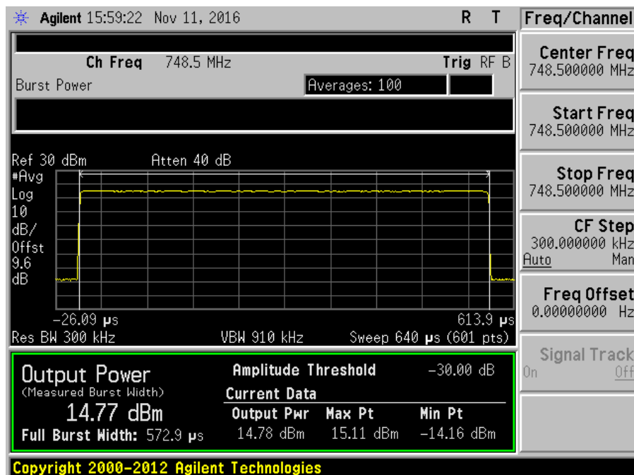
7.2_Power_DL_746-757MHz_GSM_Max
