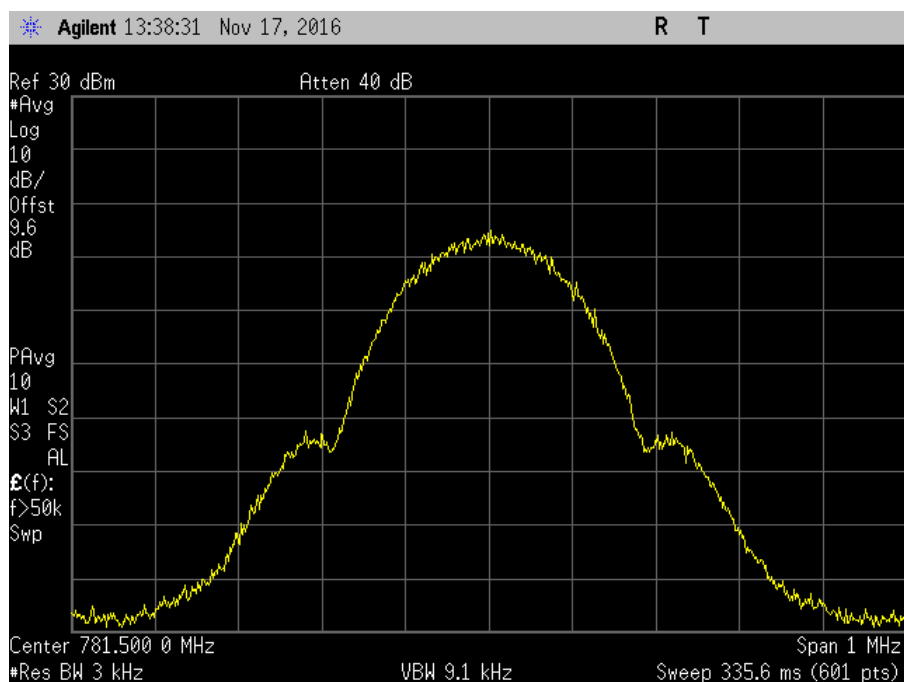
7.10_OBW_UL_776-787MHz_GSM_Out
