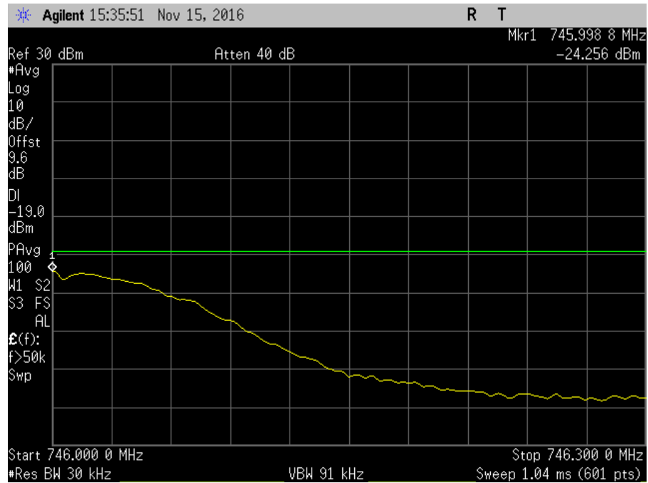
7.5_OBE_DL_728-746MHz_H_PreAGC_GSM
