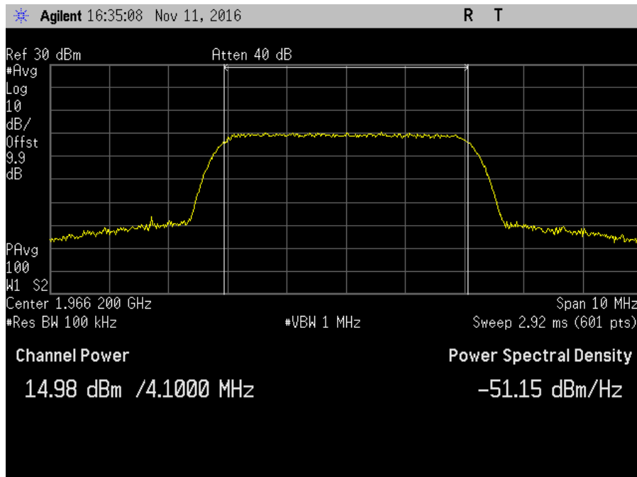
7.2_Power_DL_1930-1995MHz_AWGN_Max
