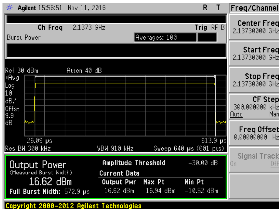
7.2_Power_DL_2110-2155MHz_GSM_Max
