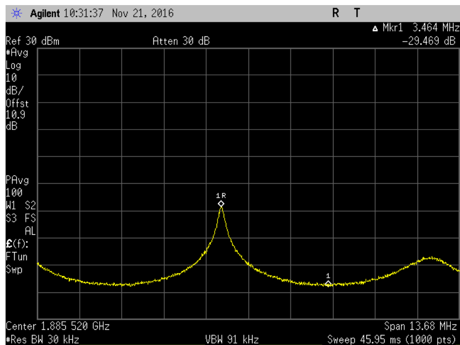
7.11.3_Osc_UL_1850-1915MHz+0_AWGNL
