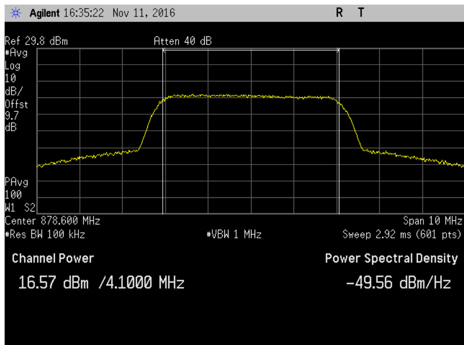
7.2_Power_DL_869-894MHz_AWGN_Max
