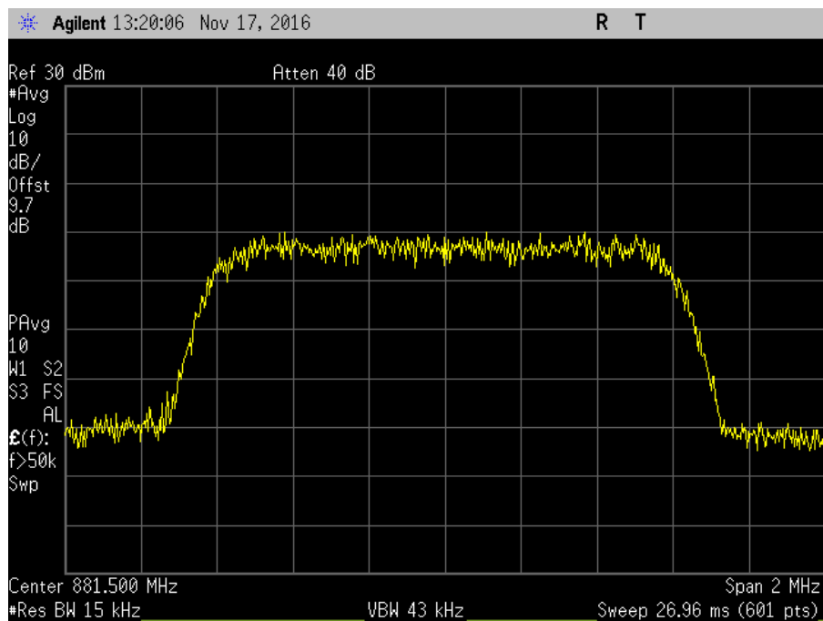
7.10_OBW_DL_869-894MHz_CDMA_Out
