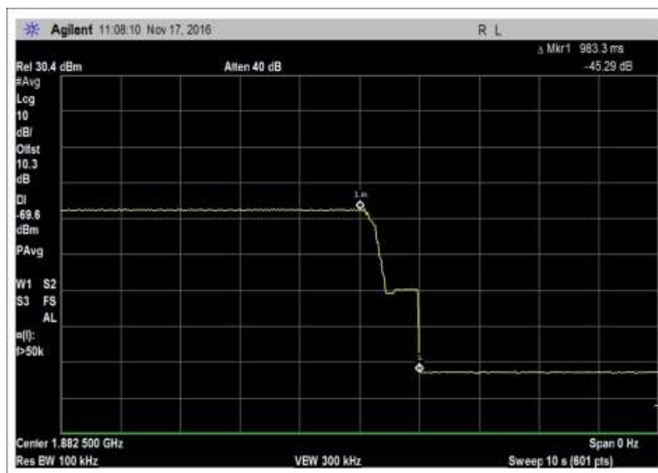
7.9.2_VarULGainTiming_UL_1850-1915MHz
