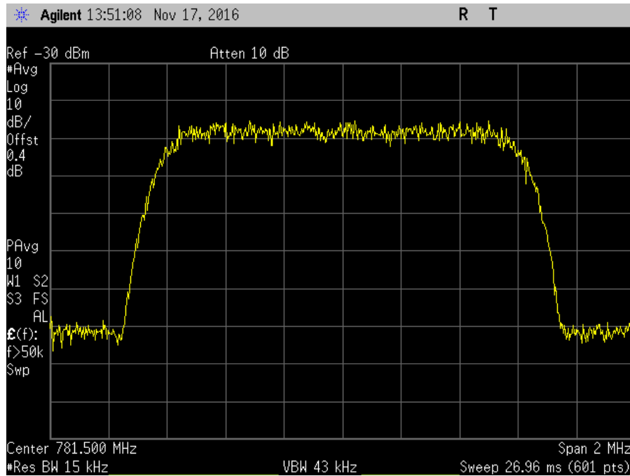
7.10_OBW_UL_776-787MHz_CDMA_In
