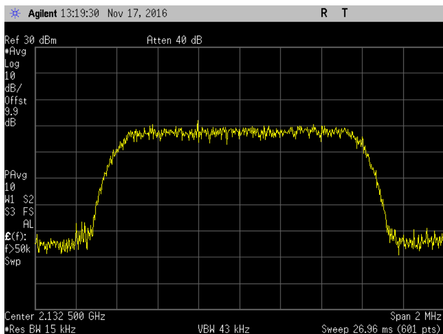
7.10_OBW_DL_2110-2155MHz_CDMA_Out
