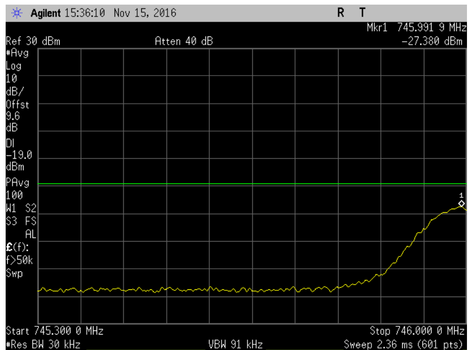
7.5_OBE_DL_746-757MHz_L_PreAGC_GSM
