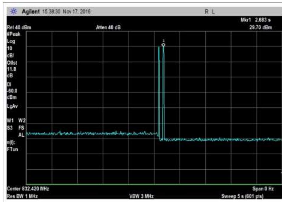
7.11_osc_UL-824-849MHz-Pk
