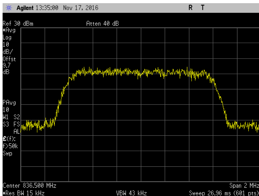
7.10_OBW_UL_824-849MHz_CDMA_Out
