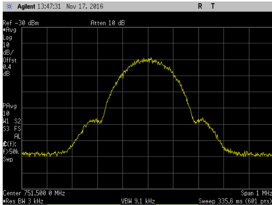
7.10_OBW_DL_746-757MHz_GSM_In
