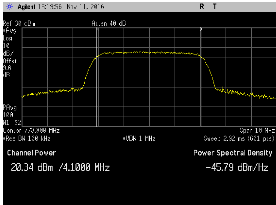
7.2_Power_UL_776-787MHz_AWGN_Max
