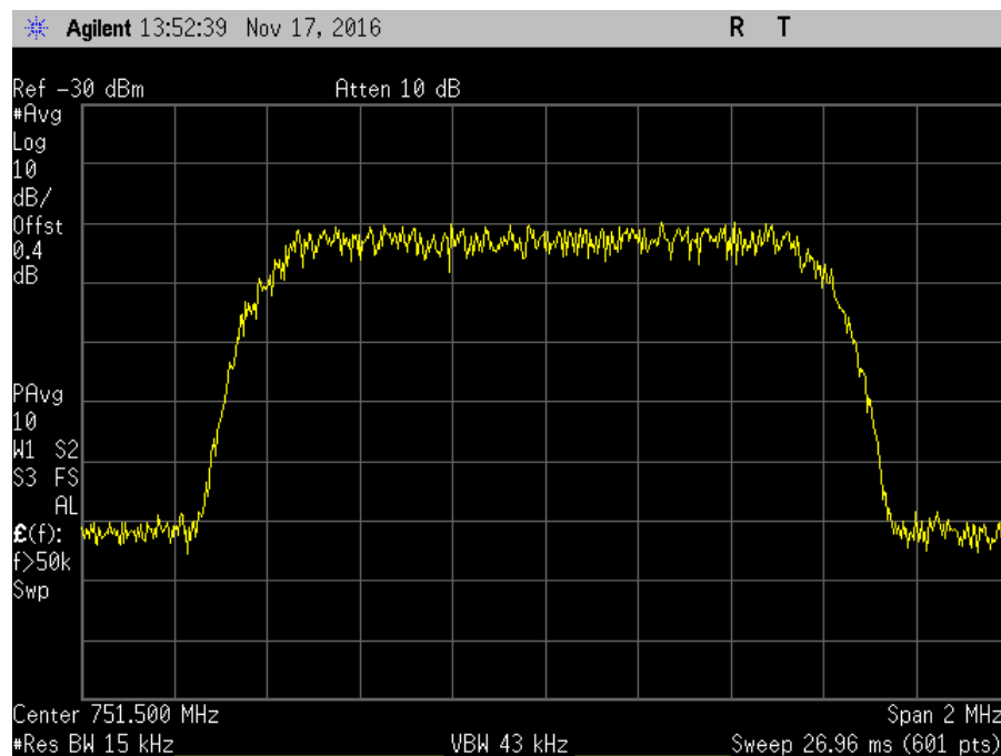
7.10_OBW_DL_746-757MHz_CDMA_In
