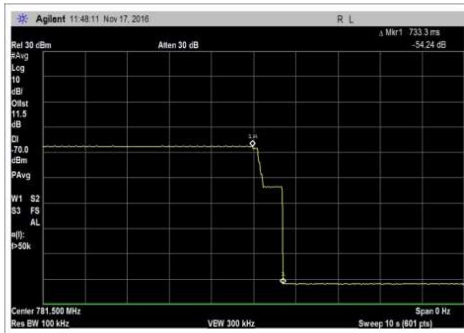
7.9.2_VarULGainTiming_UL_776-787MHz
