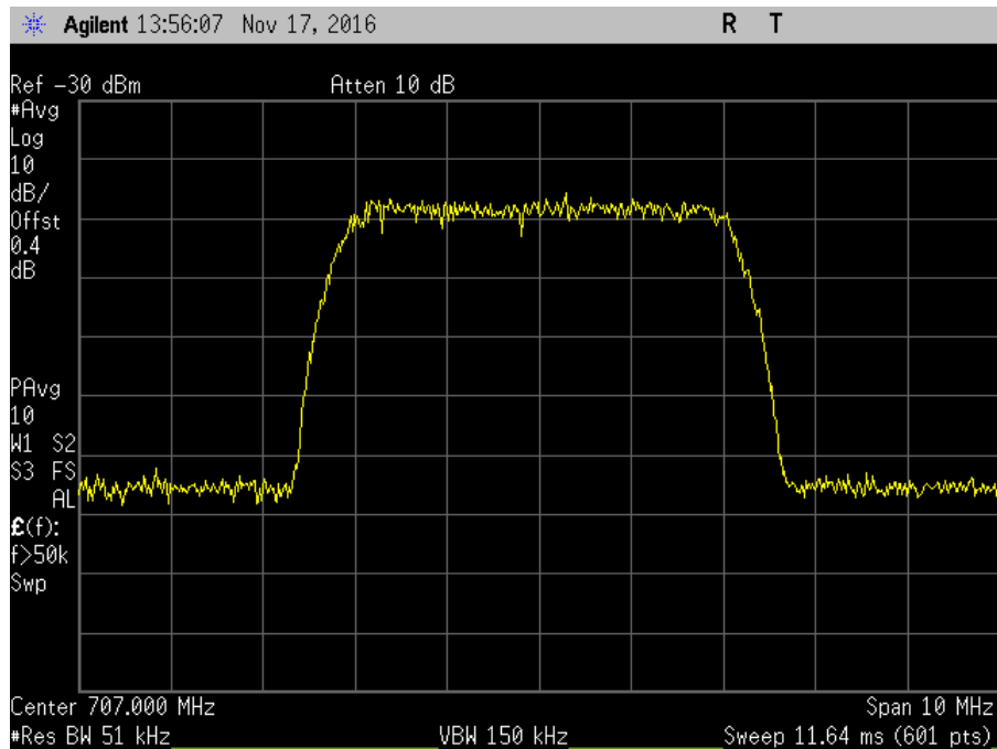
7.10_OBW_UL_698-716MHz_WCDMA_In
