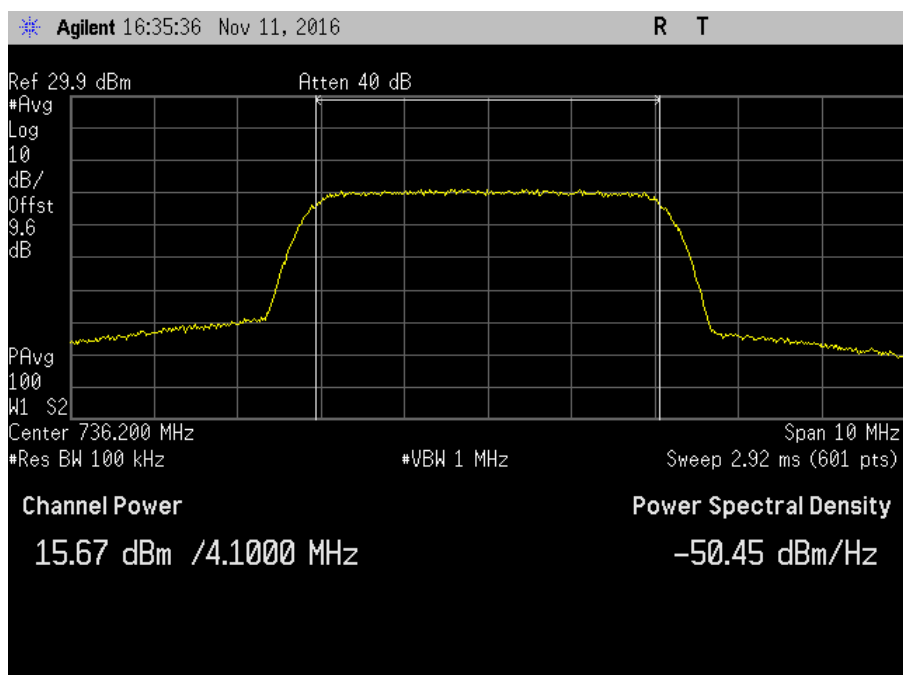
7.2_Power_DL_728-746MHz_AWGN_Max
