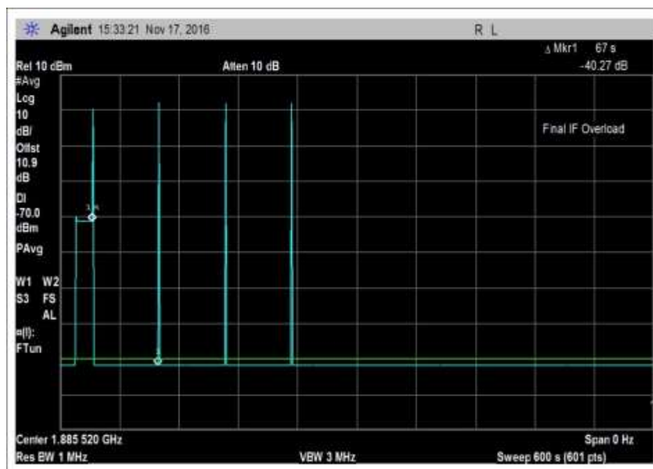
7.11_osc_UL-1850-1915MHz_600sec
