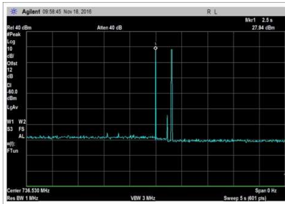
7.11_osc_DL-728-746MHz-Pk
