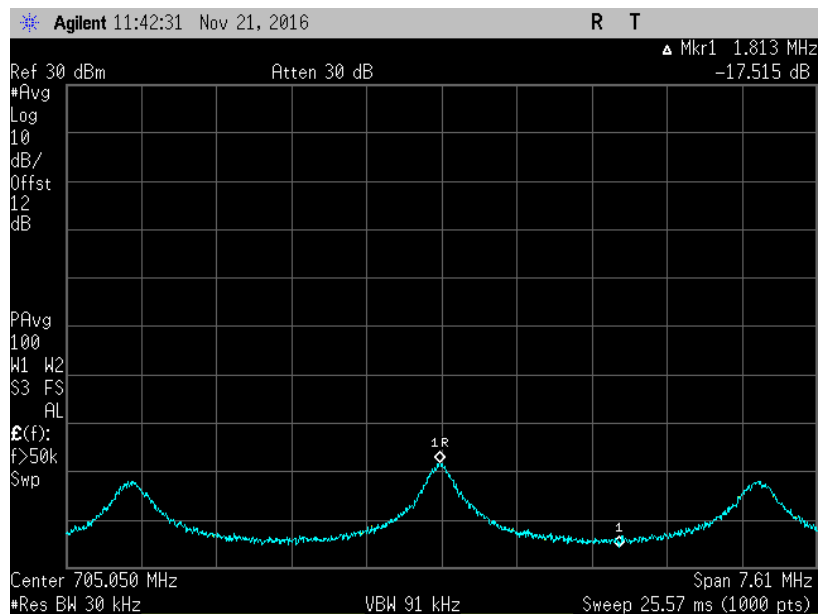
7.11.3_Osc_UL_698-716MHz+1_AWGNR
