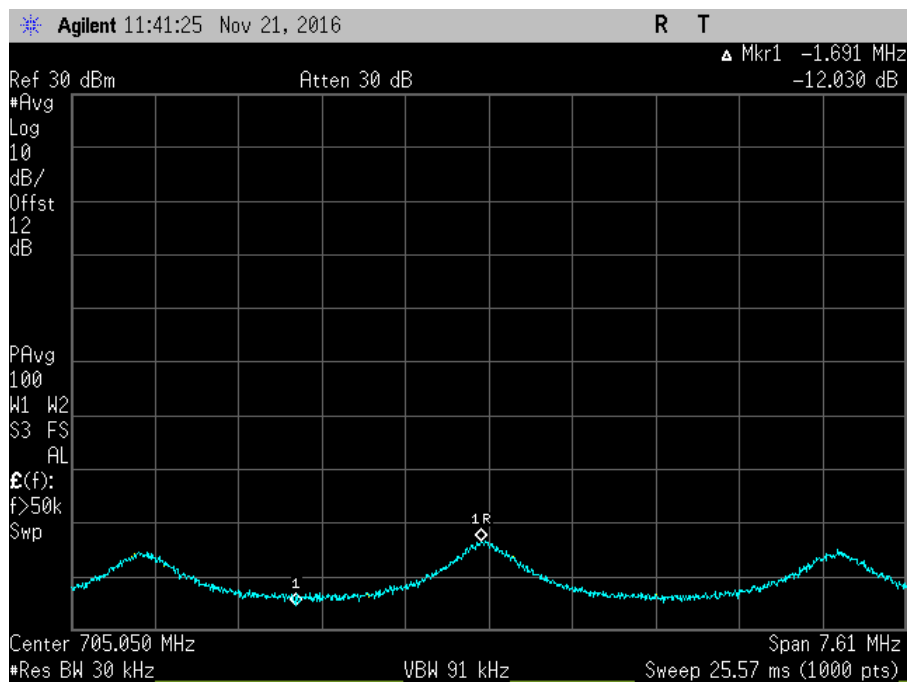
7.11.3_Osc_UL_698-716MHz+3_AWGNR
