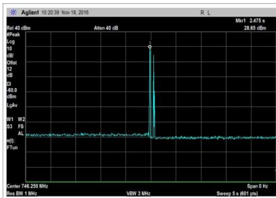
7.11_osc_DL-746-757MHz-Pk
