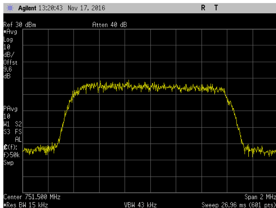
7.10_OBW_DL_746-757MHz_CDMA_Out
