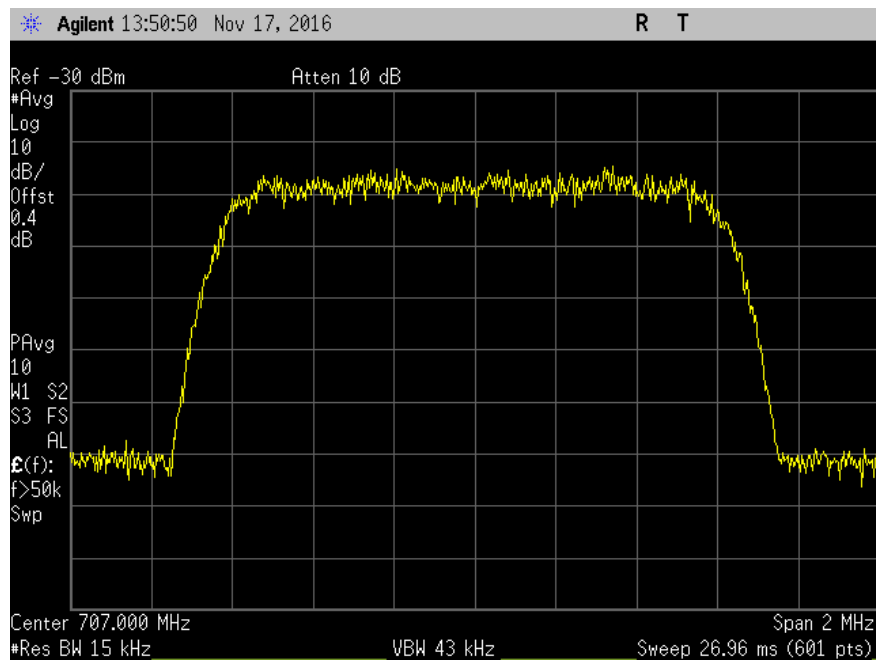
7.10_OBW_UL_698-716MHz_CDMA_In
