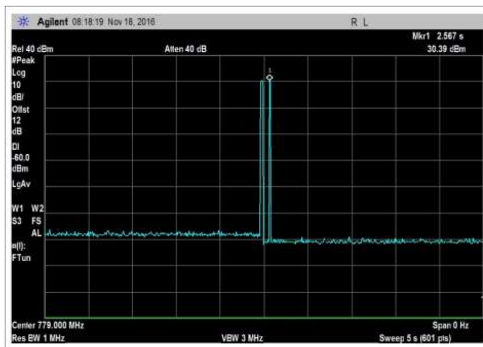
7.11_osc_UL-776-787MHz-Pk
