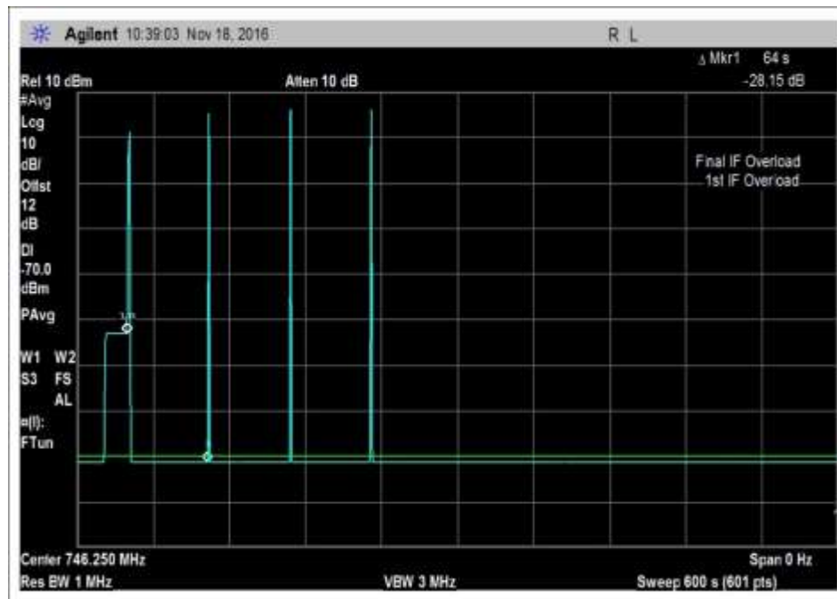
7.11_osc_DL-746-757MHz-600
