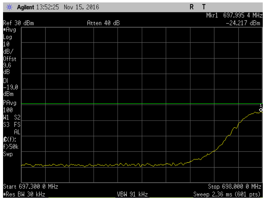
7.5_OBE_UL_698-716MHz_L_PreAGC_GSM
