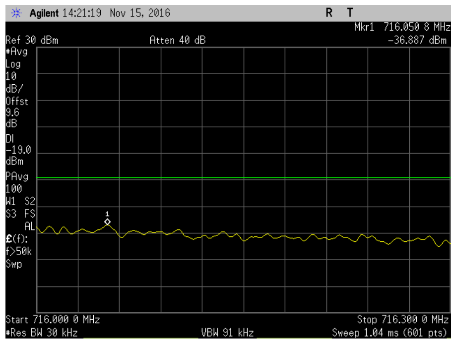
7.5_OBE_UL_698-716MHz_H_PreAGC_CDMA
