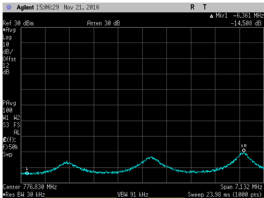
7.11.3_Osc_UL_776-787MHz+1_AWGNR
