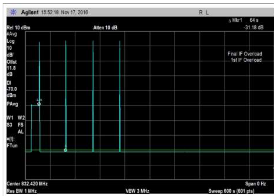
7.11_osc_UL-824-849MHz-600sec
