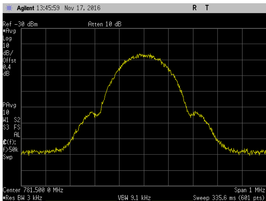
7.10_OBW_UL_776-787MHz_GSM_In
