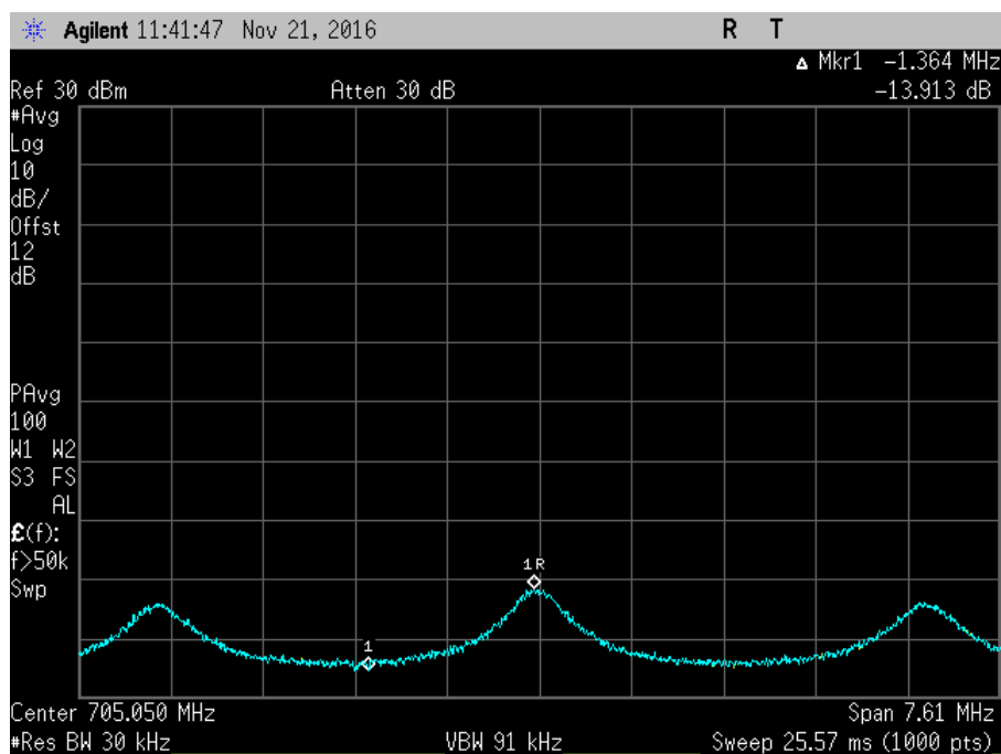
7.11.3_Osc_UL_698-716MHz+2_AWGNR
