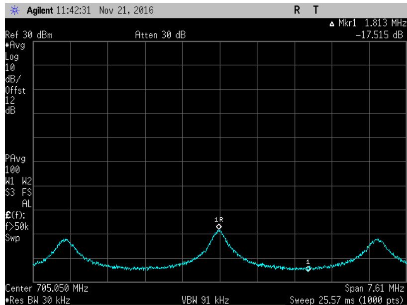
7.11.3_Osc_UL_698-716MHz+1_AWGNR
