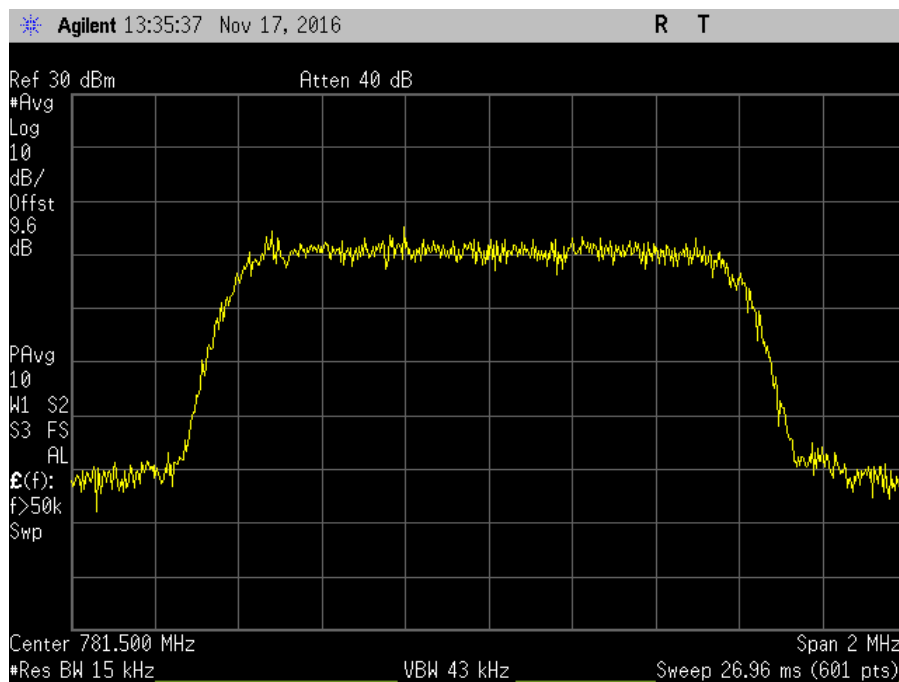
7.10_OBW_UL_776-787MHz_CDMA_Out
