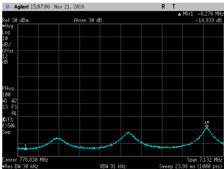
7.11.3_Osc_UL_776-787MHz+0_AWGNR
