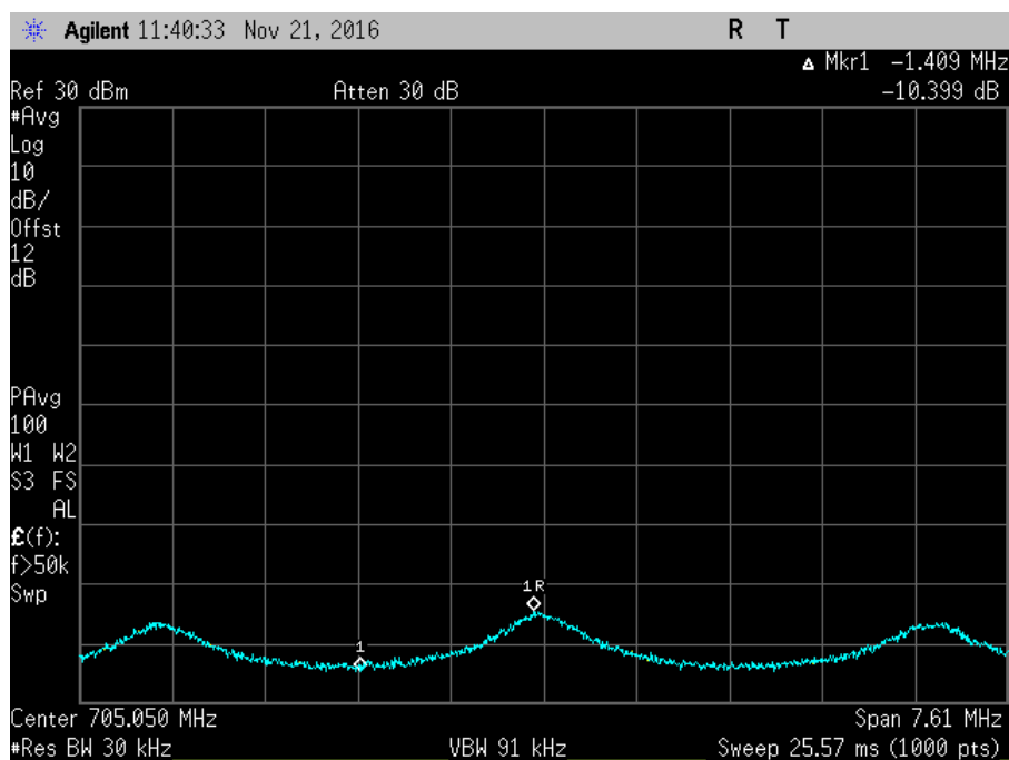
7.11.3_Osc_UL_698-716MHz+4_AWGNR
