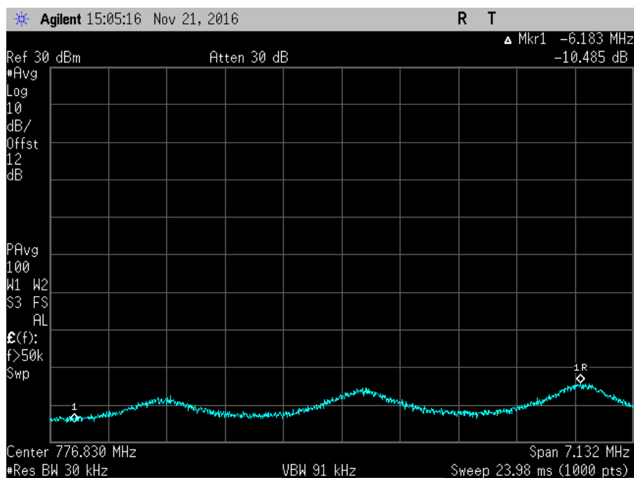
7.11.3_Osc_UL_776-787MHz+4_AWGNR
