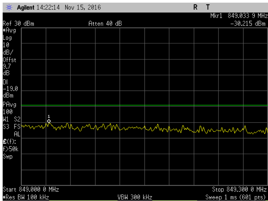
7.5_OBE_UL_824-849MHz_H_PreAGC_CDMA
