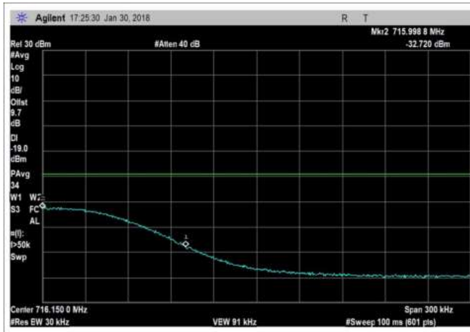
UL_698-716MHz_GSM_H_rbw=30kHz
