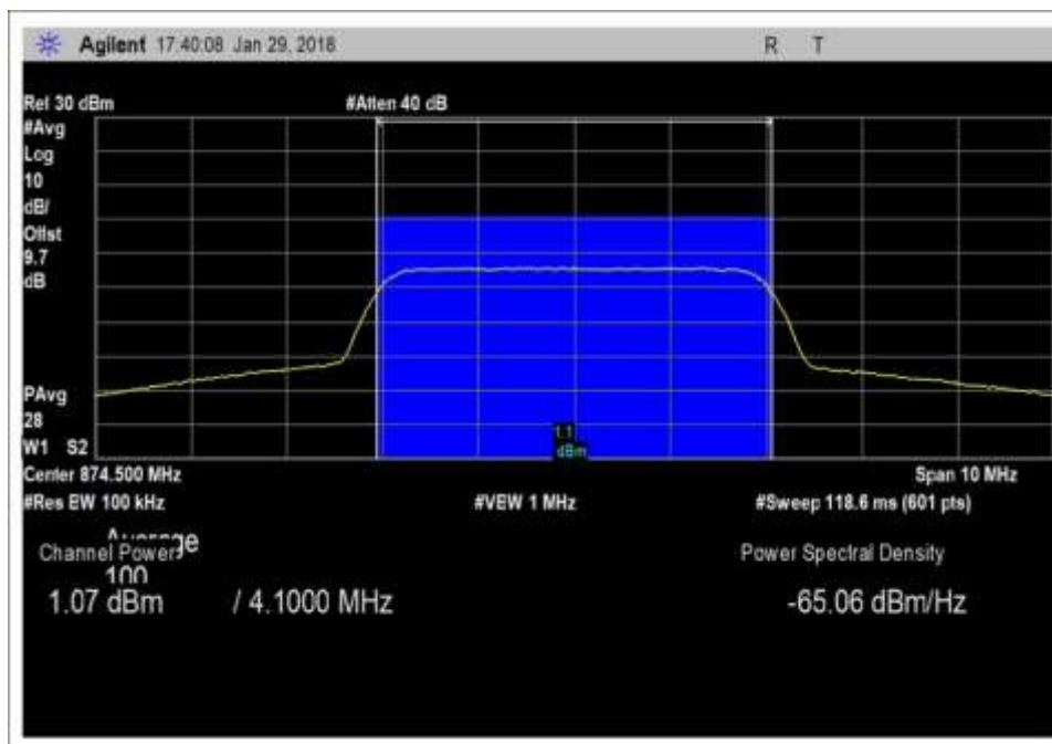
DL_869-894MHz_AWGN_max
