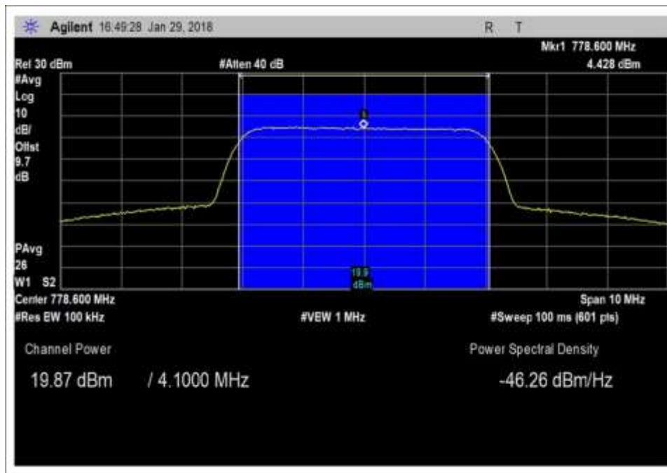
UL_776-787MHz_AWGN
