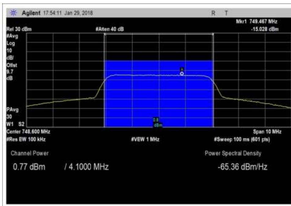
DL_746-757MHz_AWGN_max.
