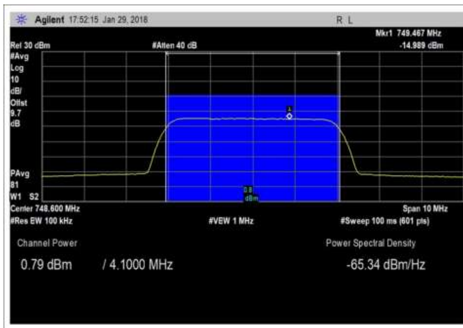
DL_746-757MHz_AWGN
