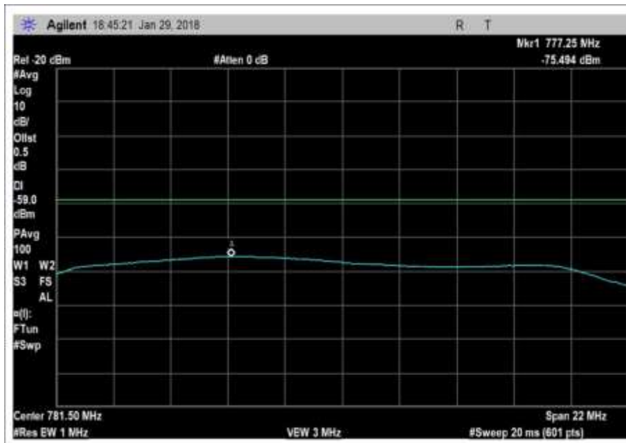
UL_776-787MHz_b
