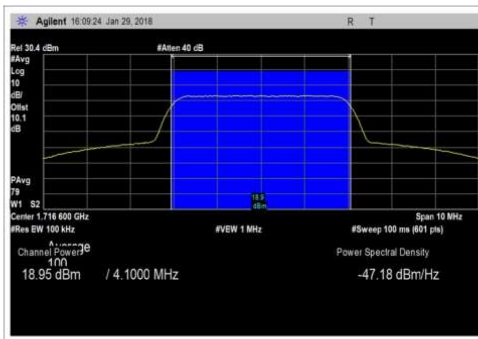
UL_1710-1755MHz_AWGN_max
