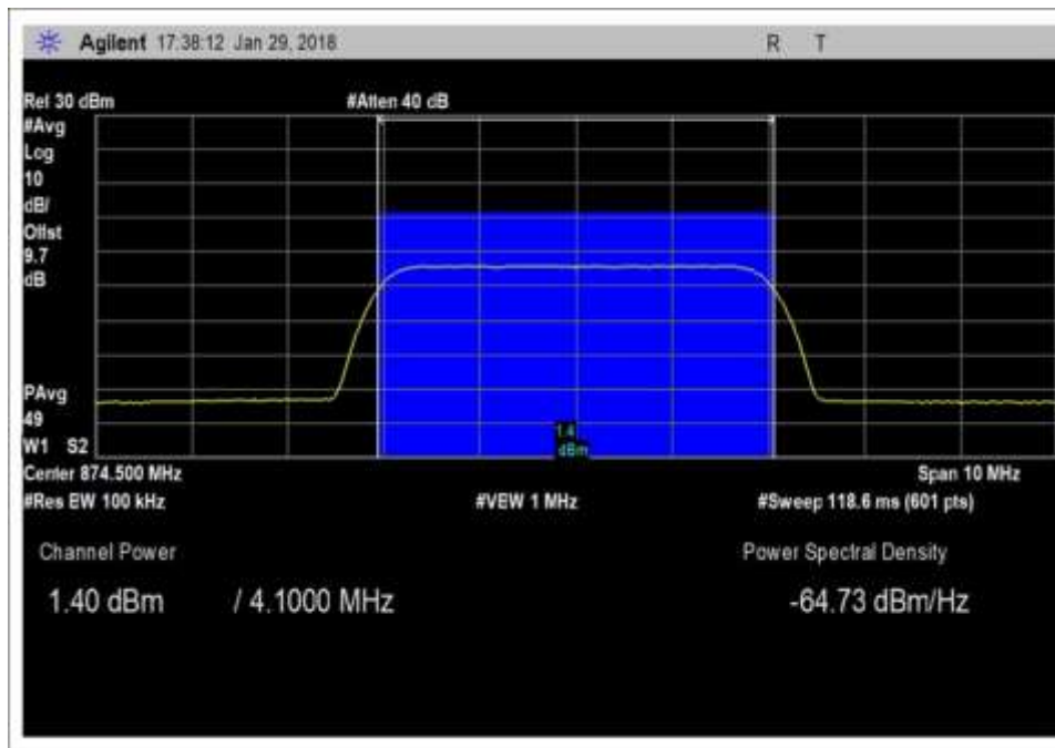
DL_869-894MHz_AWGN
