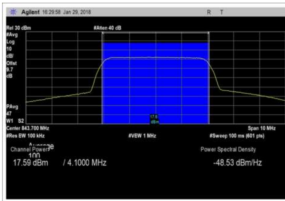
UL_824-894MHz_AWGN_max
