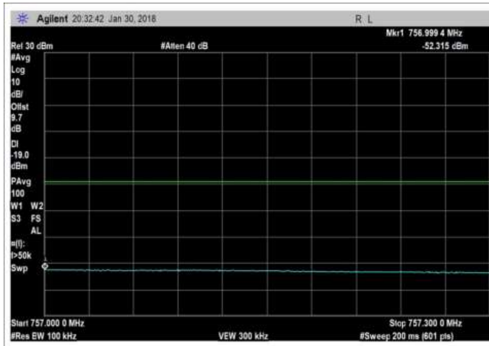
DL_746-757MHz_CDMA_H
