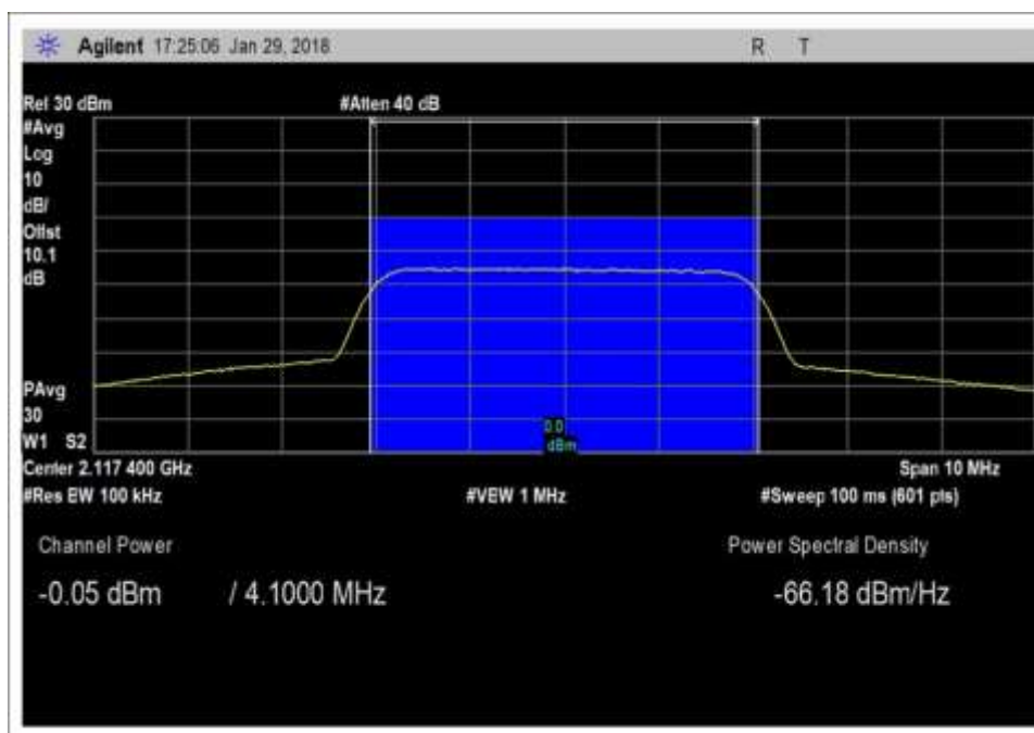
DL_2110-2155MHz_AWGN_max
