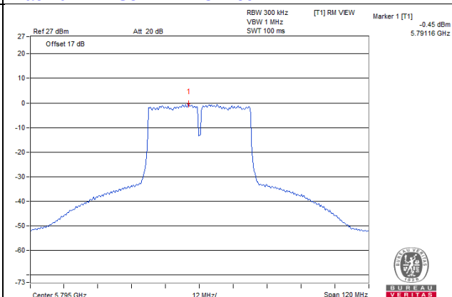
11ac 40MHz 1S3T TxBF CH159
