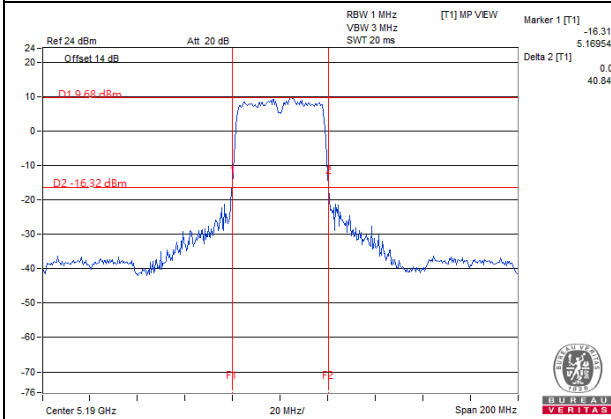
11ac 40MHz 1S3T CDD CH38 Ant2
