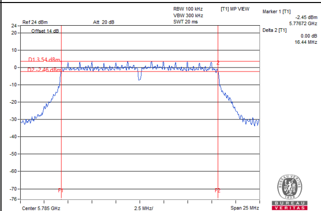
11a 1S3T CDD CH157 Ant2
