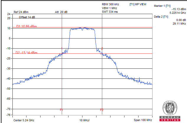
11ac 20MHz 1S3T TxBF CH48 Ant2
