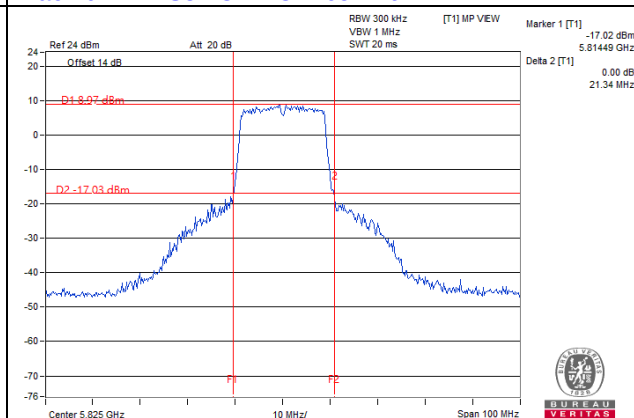
11ac 20MHz 1S3T CDD CH165 Ant2
