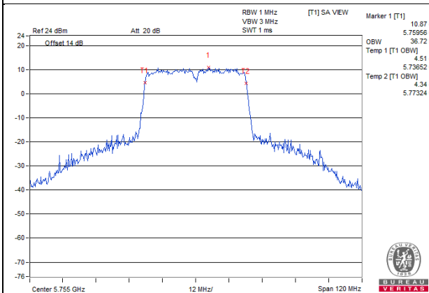
11ac 40MHz 2S3T TxBF CH151 Ant3
