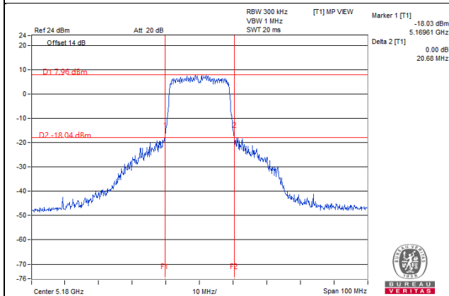
11ac 20MHz 2S3T TxBF CH36 Ant3
