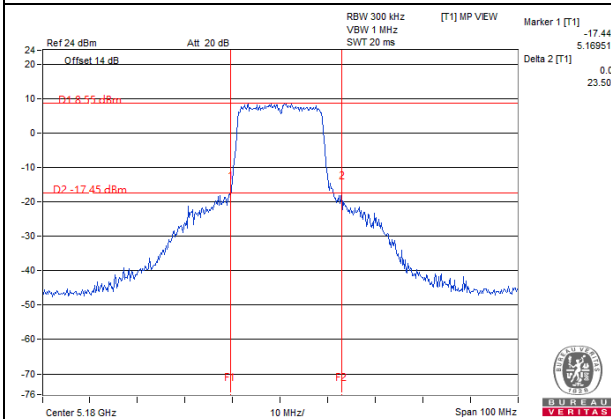
11ac 20MHz 1S3T CDD CH36 Ant2
