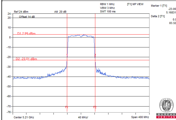
11ac 80MHz 2S3T TxBF CH42 Ant3
