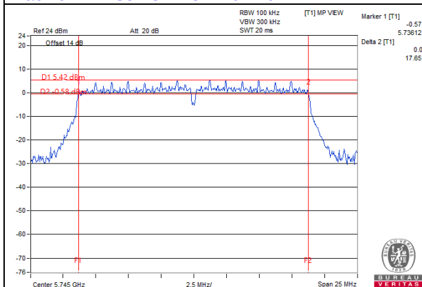
11ac 20MHz 1S3T CDD CH149 Ant2
