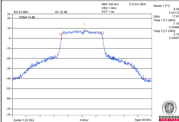
11ac 20MHz 1S3T TxBF CH48 Ant3
