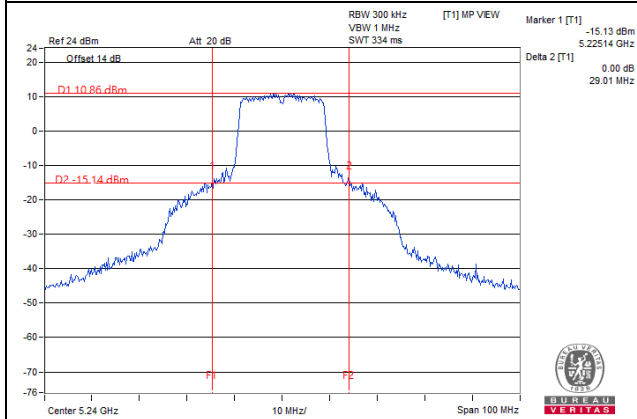
11ac 20MHz 1S3T CDD CH48 Ant2
