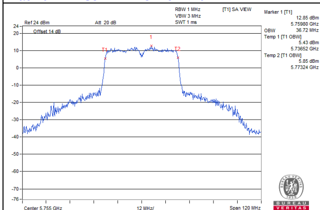
11ac 40MHz 1S3T TxBF CH151 Ant2
