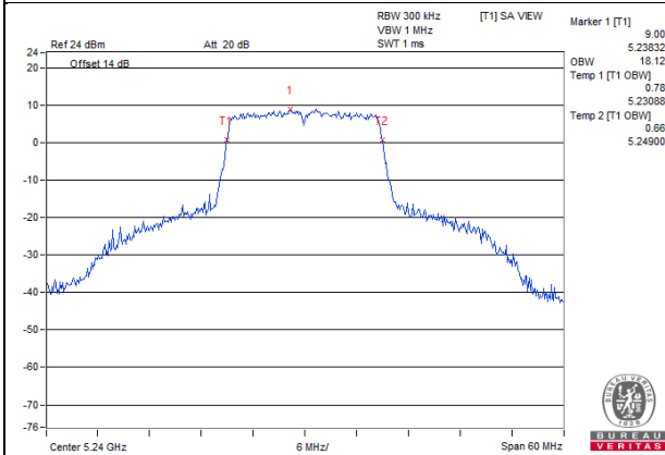
11ac 20MHz 1S3T TxBF CH48 Ant3
