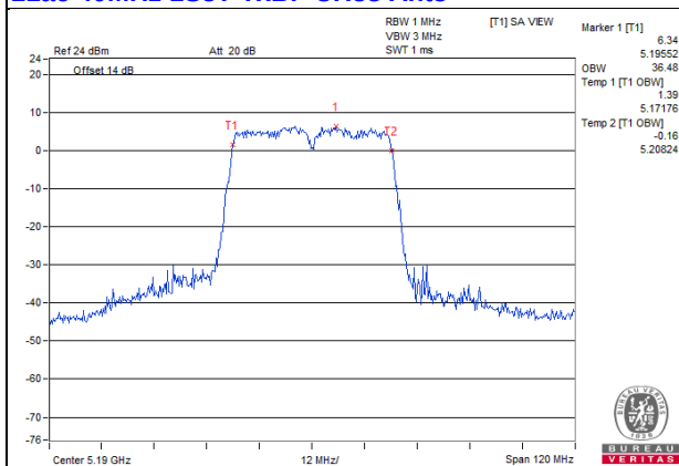
11ac 40MHz 1S3T TxBF CH38 Ant3
