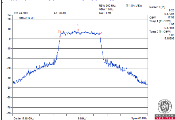
11ac 20MHz 2S3T TxBF CH36 Ant3
