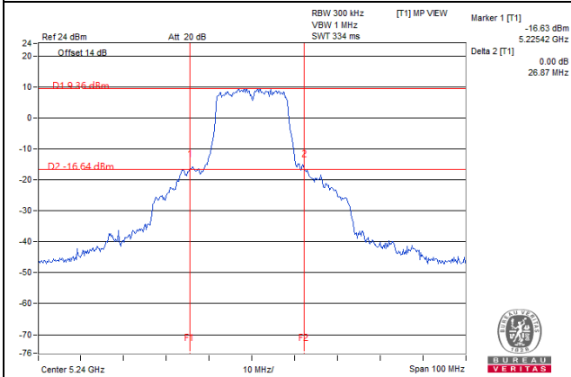
11a 1S3T CDD CH48 Ant2
