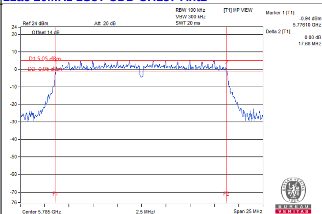
11ac 20MHz 1S3T CDD CH157 Ant3
