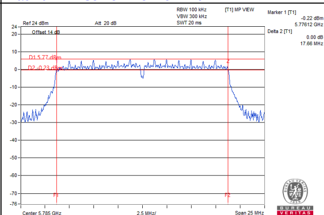
11ac 20MHz 1S3T CDD CH157 Ant2
