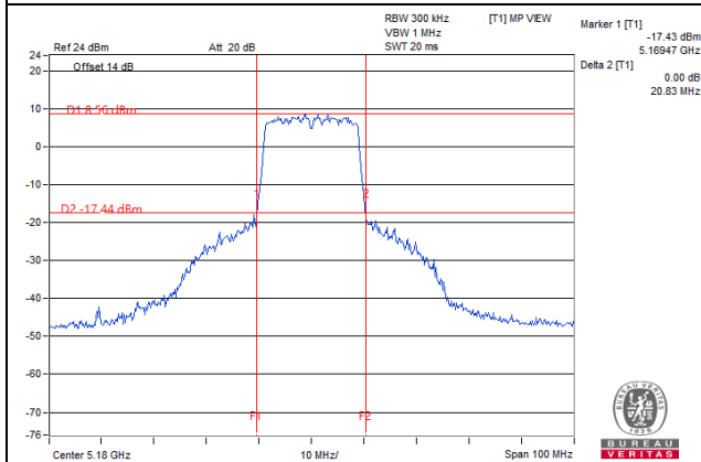
11ac 20MHz 2S3T TxBF CH36 Ant2
