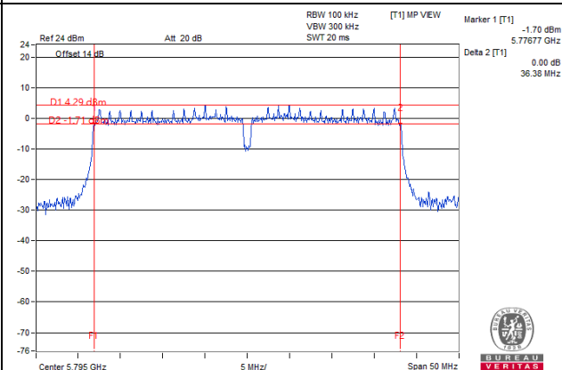
11ac 40MHz 1S3T CDD CH159 Ant2
