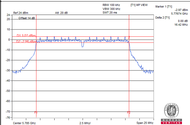
11a 1S3T CDD CH157 Ant3
