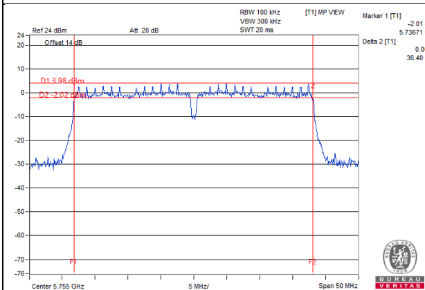
11ac 40MHz 1S3T CDD CH151 Ant3
