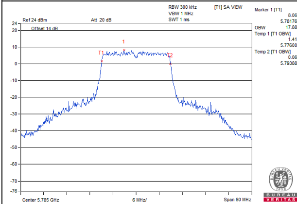
11ac 20MHz 1S3T TxBF CH157 Ant2
