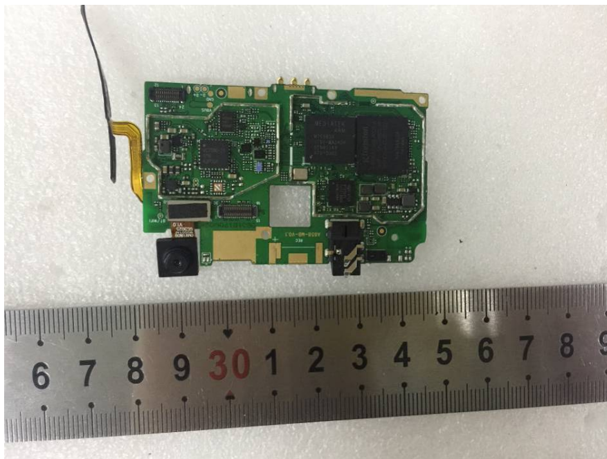
EUT – Main Board 1 Rear Shielding off View
