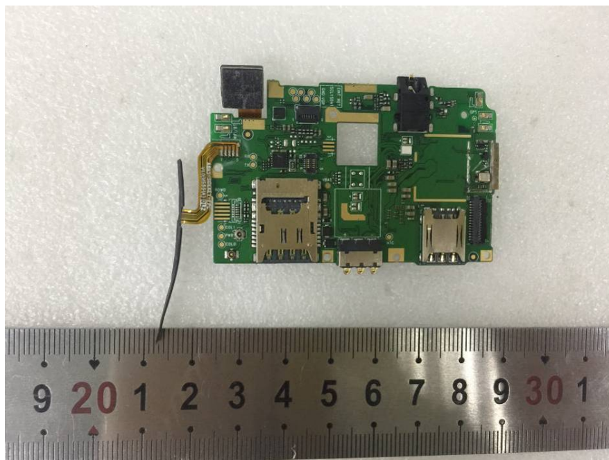
EUT – Main Board 1 Front Shielding off View
