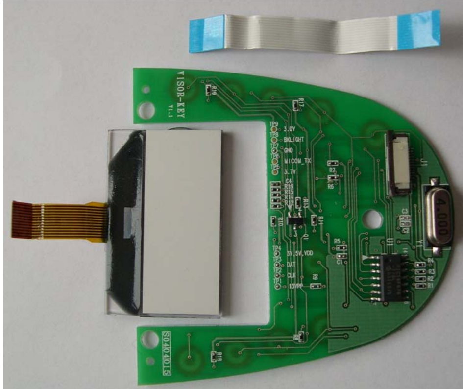
<Photograph 4: Front View - Keyboard and LCD unit>
