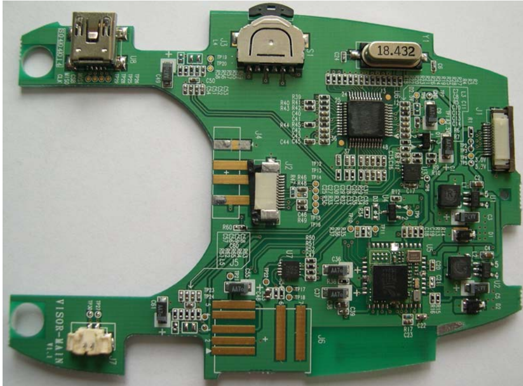
<Photograph 2: Front View - Main board>
