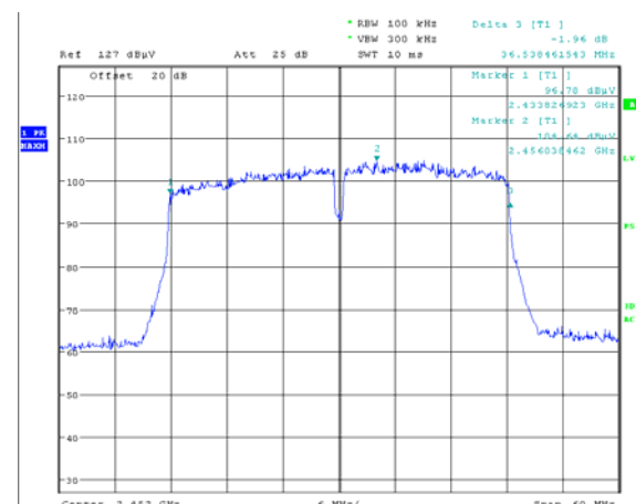
802.11 n (HT40)2452MHz
