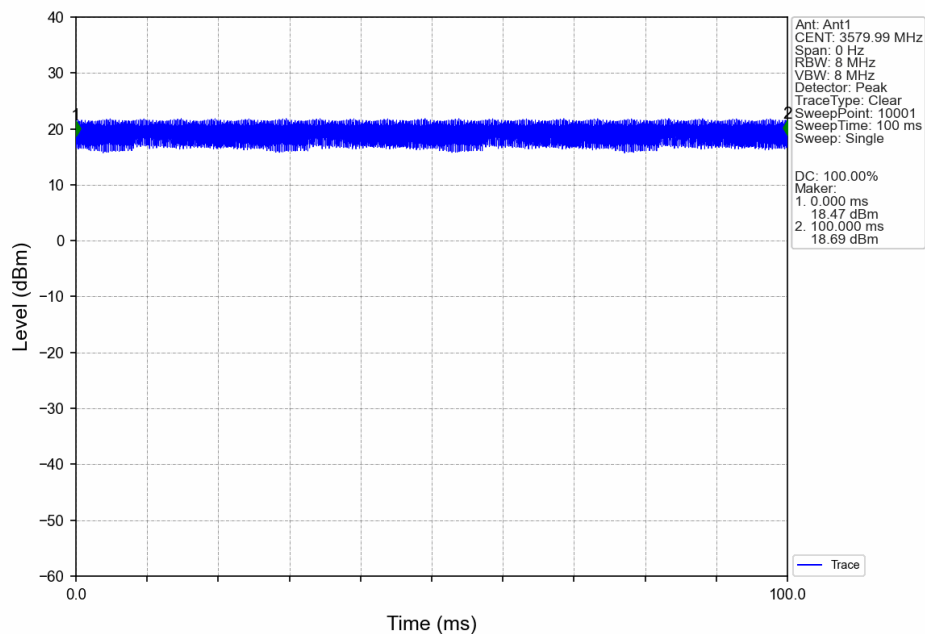
n78d_BS Type 1-C_30_Single_NTNV_CC1:60MHz_NR-FR1-TM3.1a_CC1:3579.99MHz_Ant1
