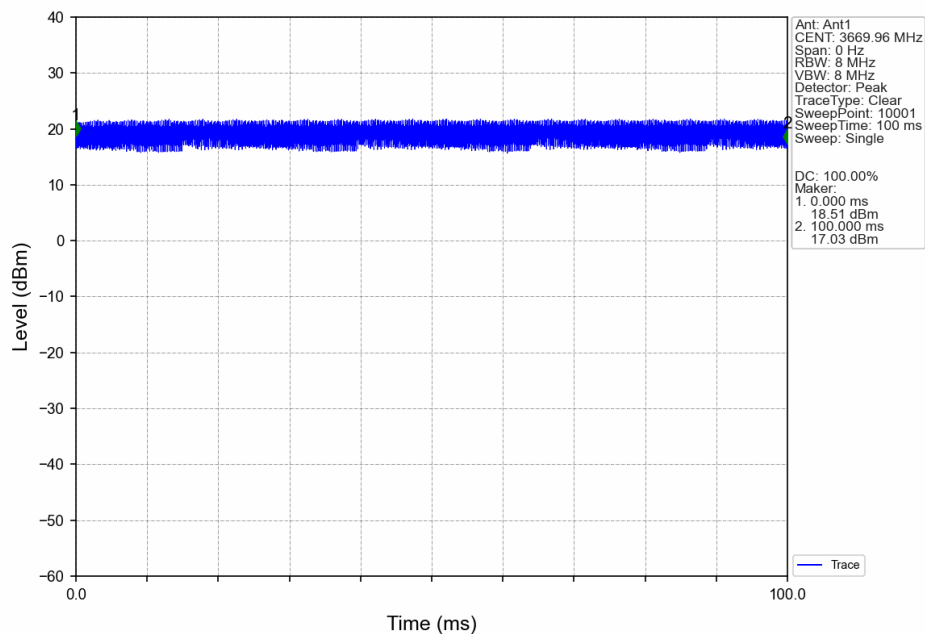
n78d_BS Type 1-C_30_Single_NTNV_CC1:60MHz_NR-FR1-TM3.1a_CC1:3669.96MHz_Ant1
