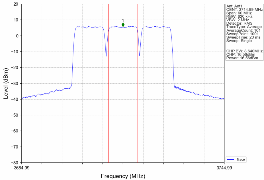
n77a_BS Type 1-C_30_Continuous_NTNV_CC1:10 CC2:10 CC3:10MHz_NR-FR1-TM3.1a_CC1:3705 CC2:3714.99 CC3:3724.98MHz Ant1
