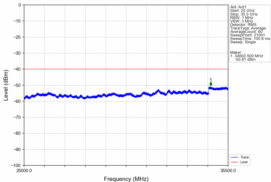
n77d_BS Type 1-C_30_Single_NTNV_CC1:40MHz_NR-FR1-TM3.1a_CC1:3529.98MHz_Ant1
