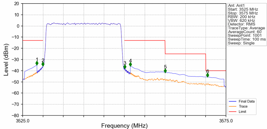
n77d_BS Type 1-C_30_Single_NTNV_CC1:20MHz_NR-FR1-TM3.1a_CC1:3540MHz_Ant1
