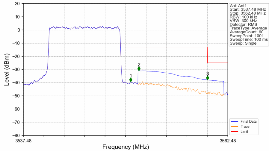
n77d_BS Type 1-C_30_Single_NTNV_CC1:10MHz_NR-FR1-TM3.1a_CC1:3544.98MHz_Ant1
