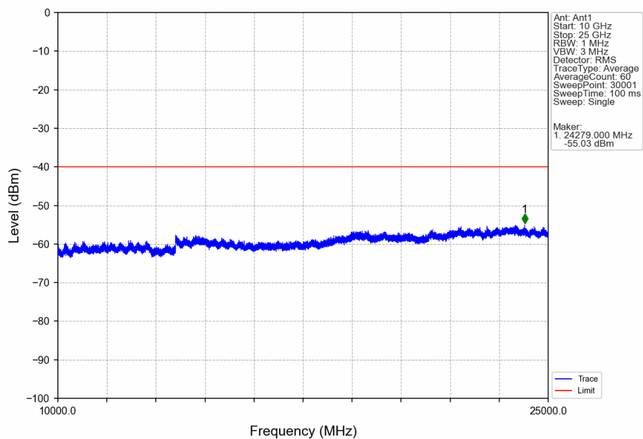
n77d_BS Type 1-C_30_Single_NTNV_CC1:40MHz_NR-FR1-TM3.1a_CC1:3499.98MHz_Ant1
