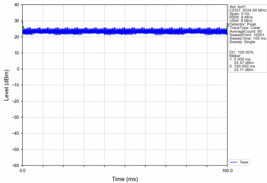
n77d_BS Type 1-C_30_Single_NTNV_CC1:30MHz_NR-FR1-TM3.1a_CC1:3534.99MHz_Ant1
