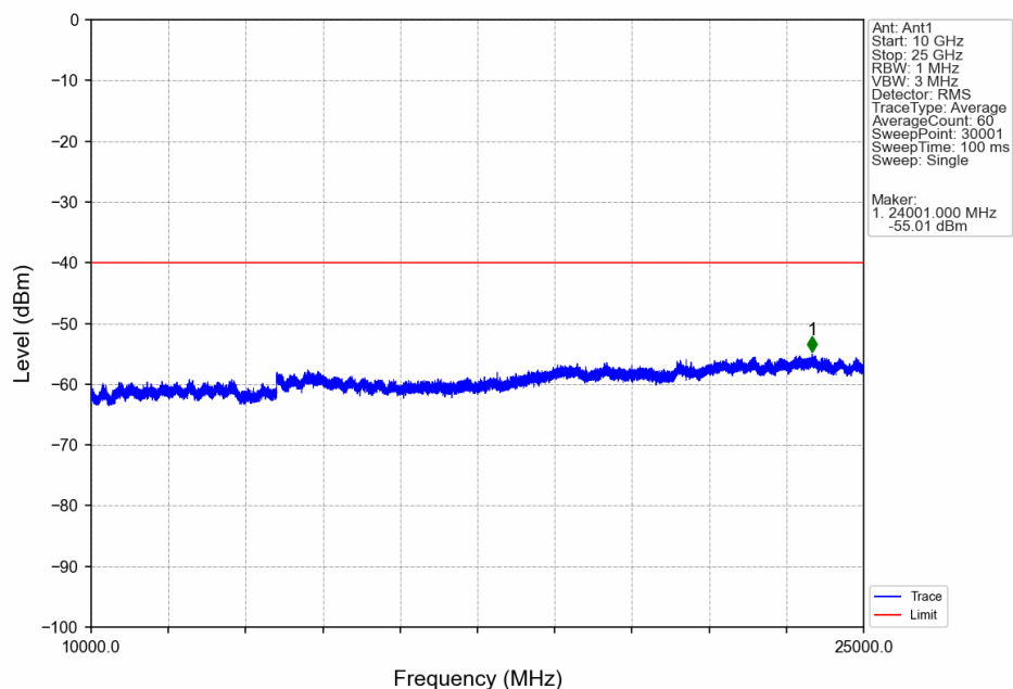
n77d_BS Type 1-C_30_Single_NTNV_CC1:40MHz_NR-FR1-TM3.1a_CC1:3529.98MHz_Ant1
