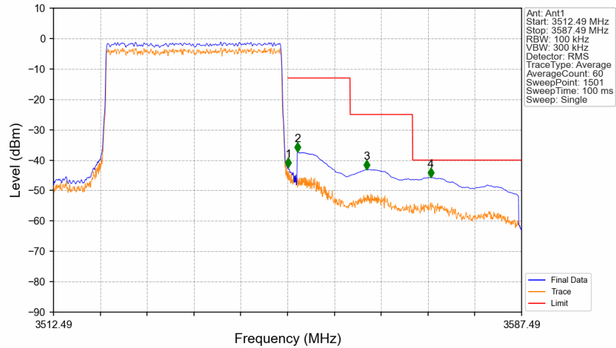
n77d_BS Type 1-C_30_Single_NTNV_CC1:30MHz_NR-FR1-TM3.1a_CC1:3534.99MHz_Ant1
