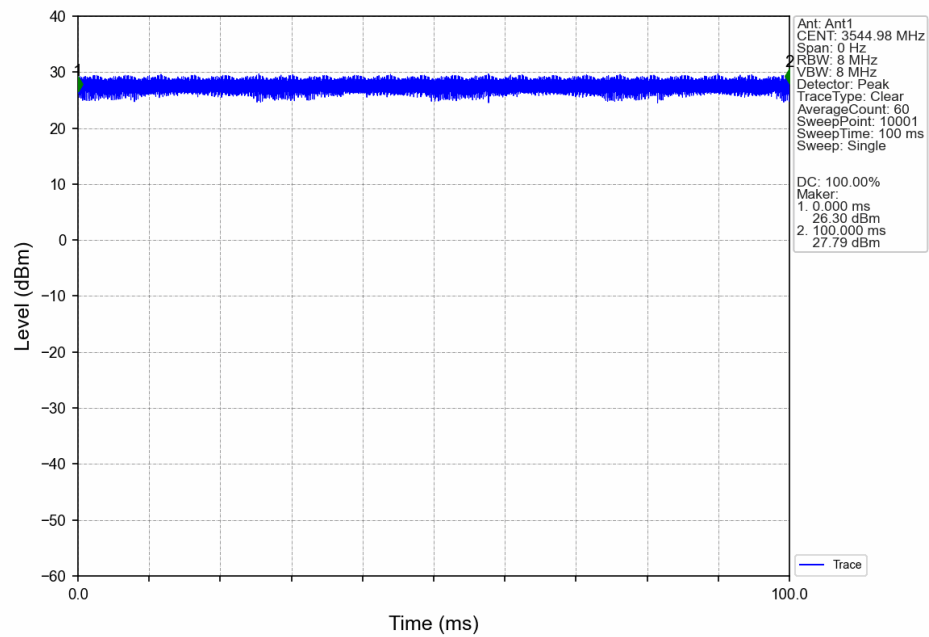
n77d_BS Type 1-C_30_Single_NTNV_CC1:10MHz_NR-FR1-TM3.1a_CC1:3544.98MHz_Ant1
