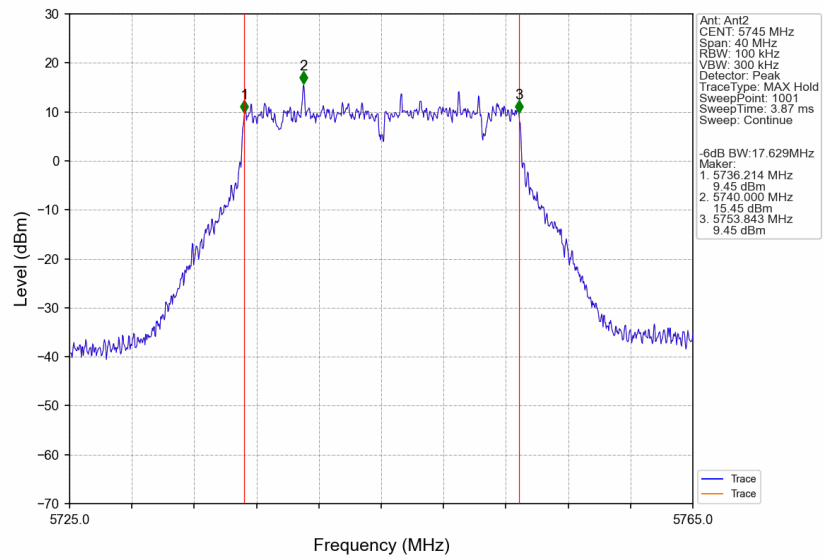
802.11ac(VHT20)_LCH_5745MHz_Ant2_NTNV
