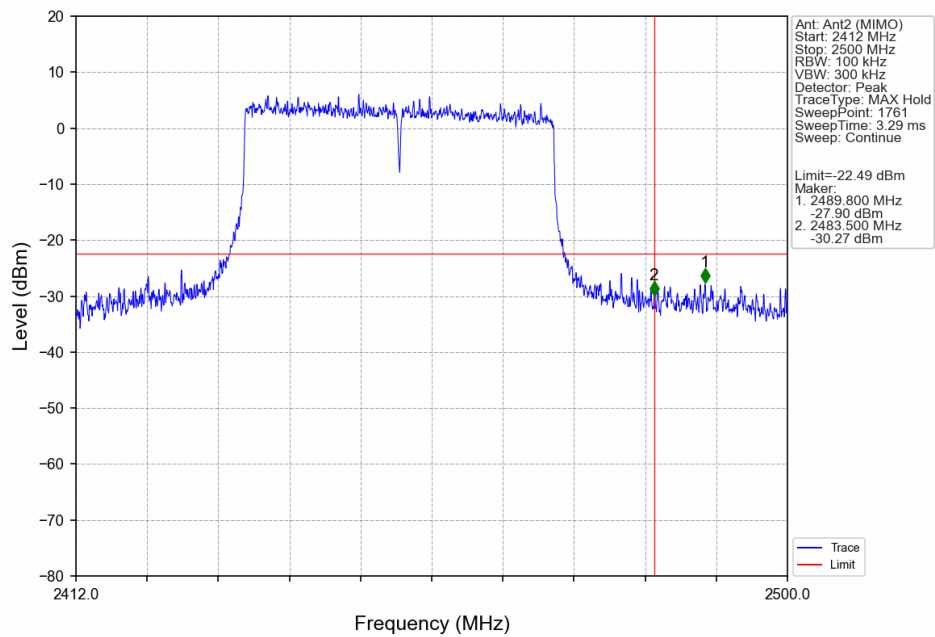
802.11ax(HEW40)_HCH_2452MHz_SU_/_Ant2 (MIMO)_NTNV
