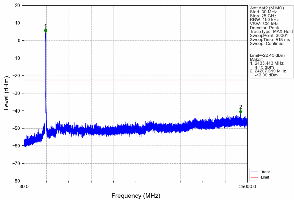
802.11ax(HEW40)_HCH_2452MHz_SU_/_Ant2 (MIMO)_NTNV
