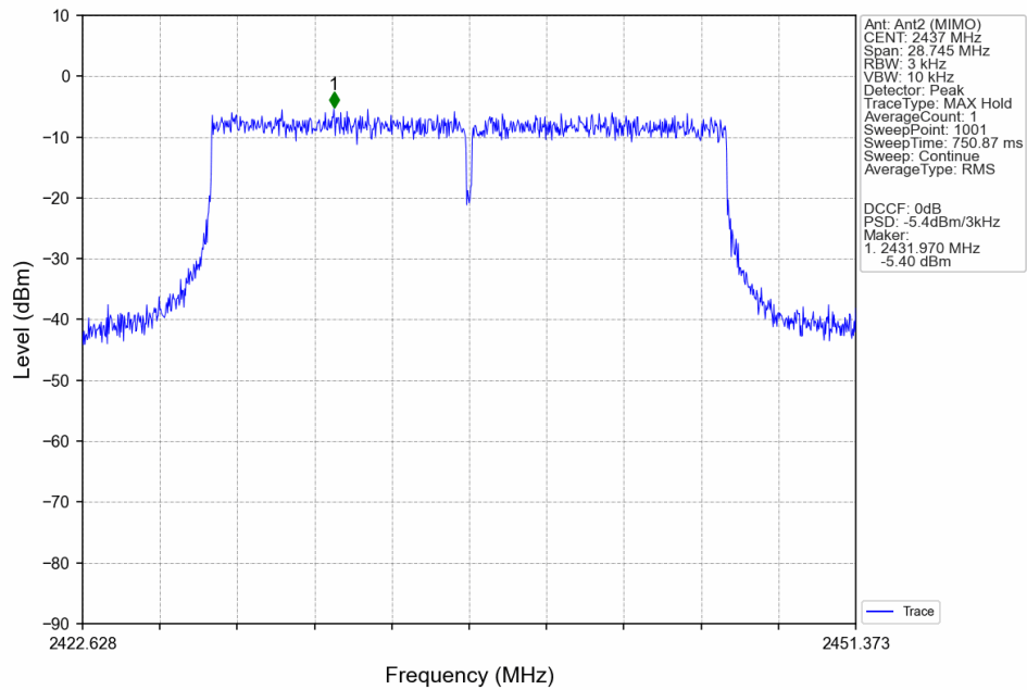
802.11ax(HEW20)_MCH_2437MHz_SU_/_MIMO_NTN
