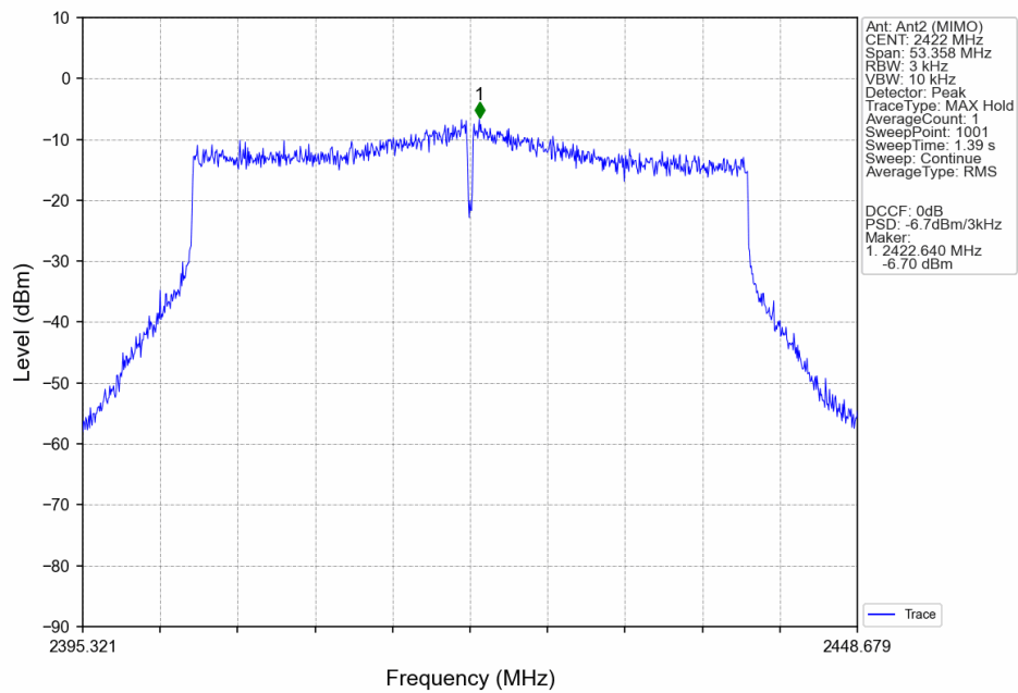
802.11be(EHT40)_LCH_2422MHz_SU_/_MIMO_NTN
