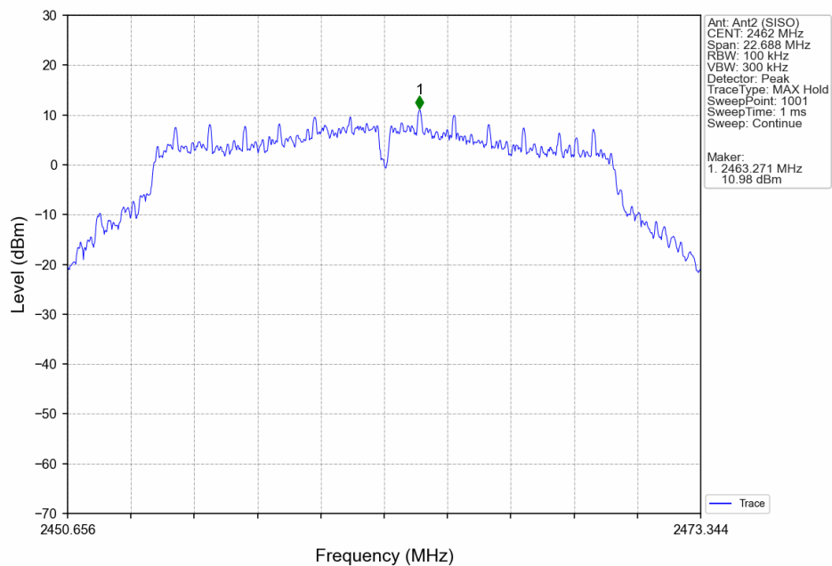
802.11g_HCH_2462MHz_Ant2 (SISO)_NTN
