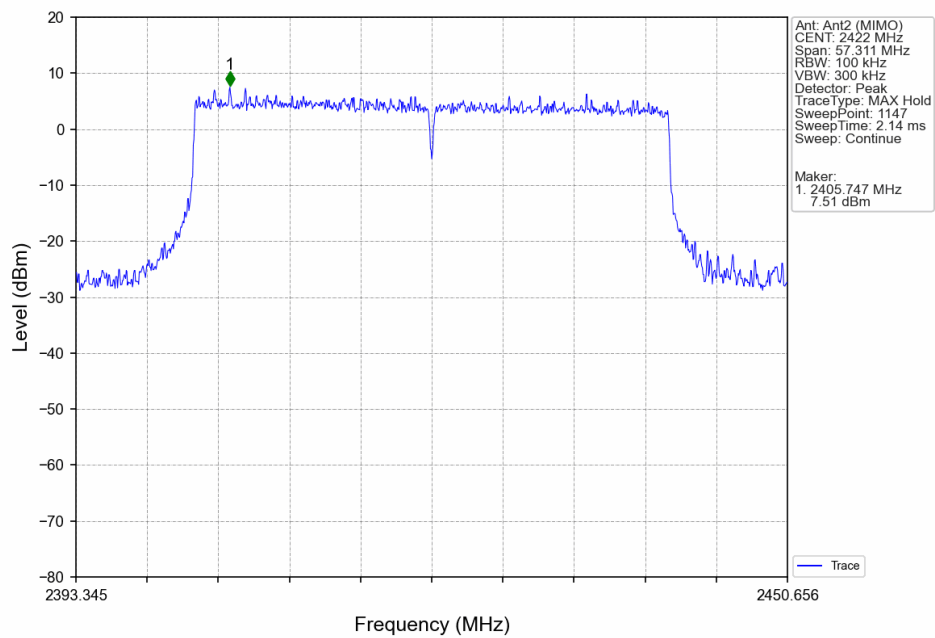
802.11ax(HEW40)_LCH_2422MHz_SU_/_Ant2 (MIMO)_NTNV
