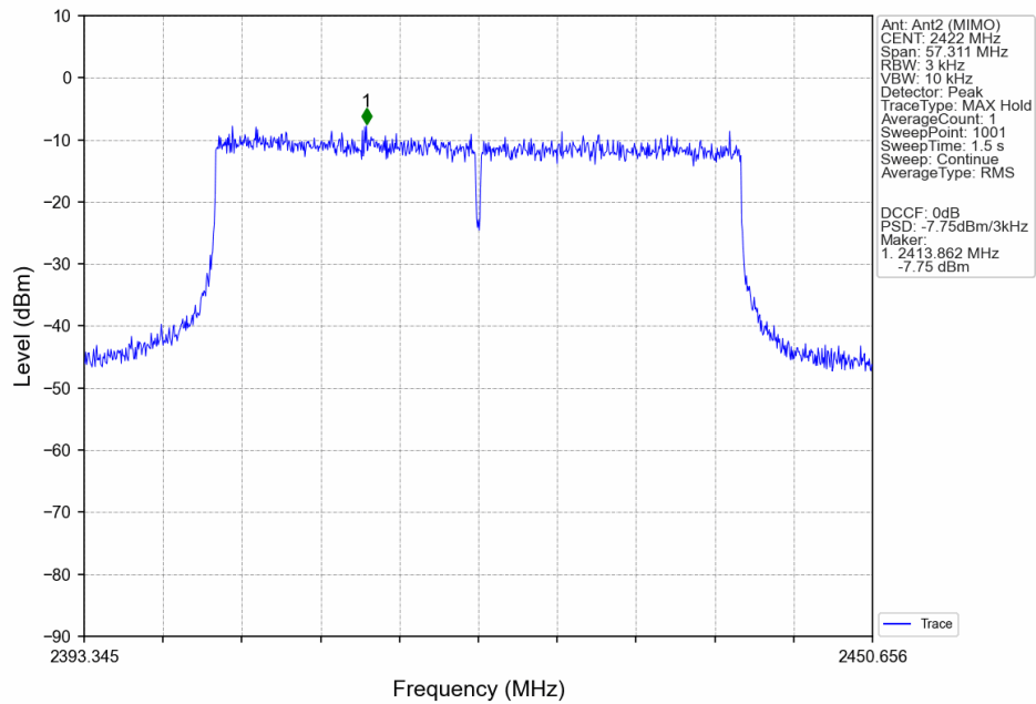
802.11ax(HEW40)_LCH_2422MHz_SU_/_MIMO_NTN
