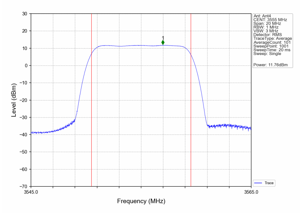
n78d_BS Type 1-C_30_Single_NTNV_CC1:10MHz_NR-FR1-TM3.1a_CC1:3555MHz_Ant4
