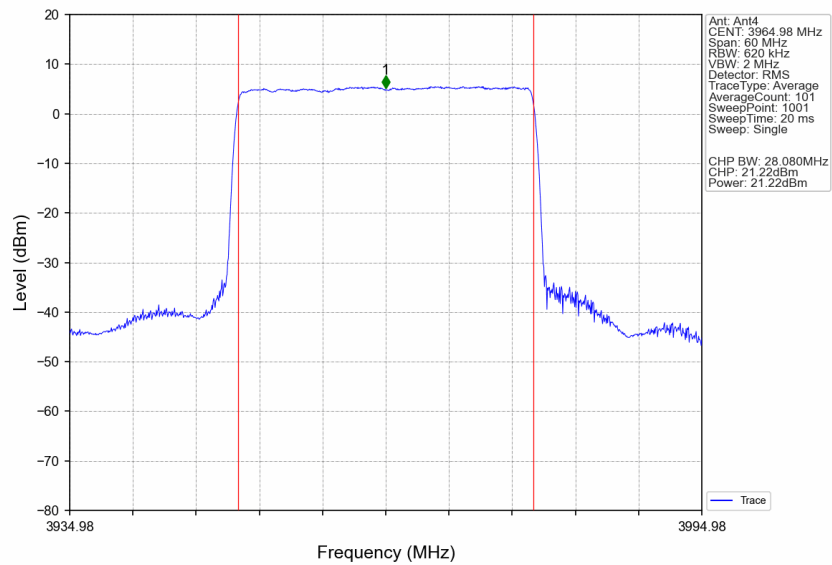
n77h_BS Type 1-C_30_Single_NTNV_CC1:30MHz_NR-FR1-TM3.1a_CC1:3964.98MHz_Ant4
