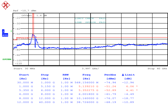
Figure 8.4-9: Conducted peak spurious emissions within restricted bands at low channel, cho, PMP with Antenna configuration 2
