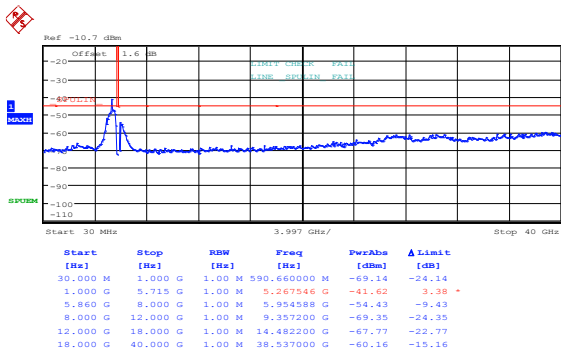
Figure 8.4-17: Conducted peak spurious emissions outside restricted bands at low channel, cho, PMP with Antenna configuration 1
