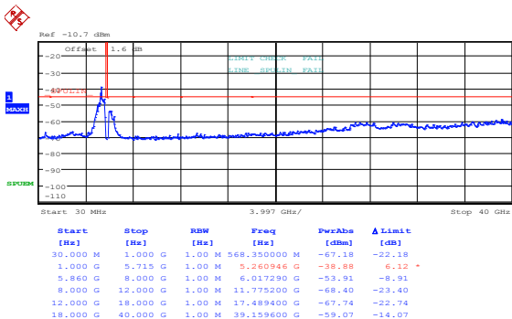
Figure 8.4-13: Conducted peak spurious emissions outside restricted bands at low channel, cho, PTP
