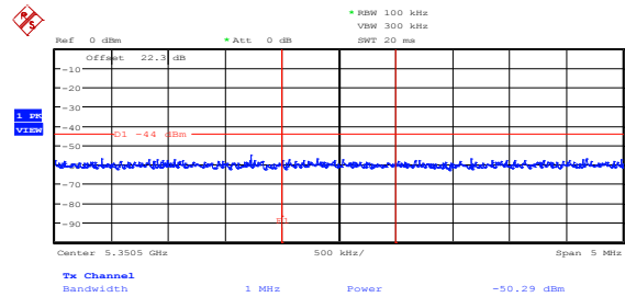
Figure 8.4-12: Upper band edge emission, ch1
