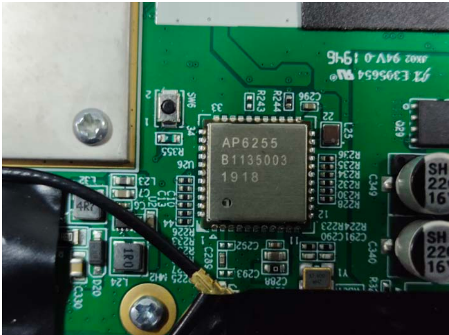
EUT – 2.4G/5G Wi-Fi & Bluetooth Module View
