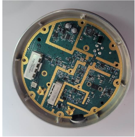
Yahsat T-TAC Maritime Antenna Step 2 – Mounting of PCBA
