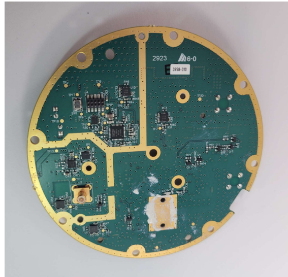
Yahsat T-TAC Maritime Antenna PCBA BottomView
