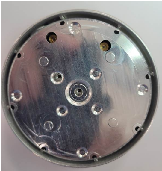
Yahsat T-TAC Maritime Antenna Step 3 – Mounting of Inner Shield
