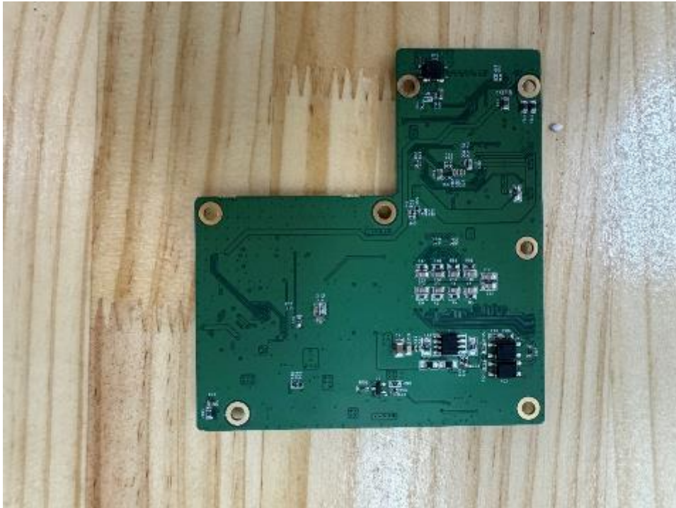
Rear View of Power Board_EXPD 4343N1, EXPD 3643N1
