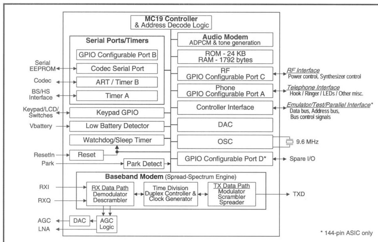
DA579 ASIC Block Diagram
