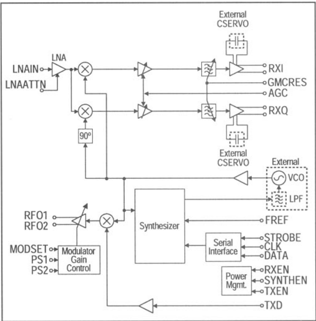
DA579 RF Block Diagram
