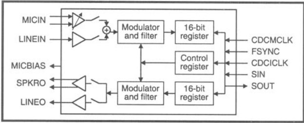
DA579 CODEC Block Diagram
