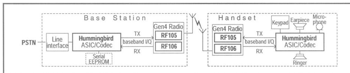
DA579 Spread Spectrum Telephone System Architecture
