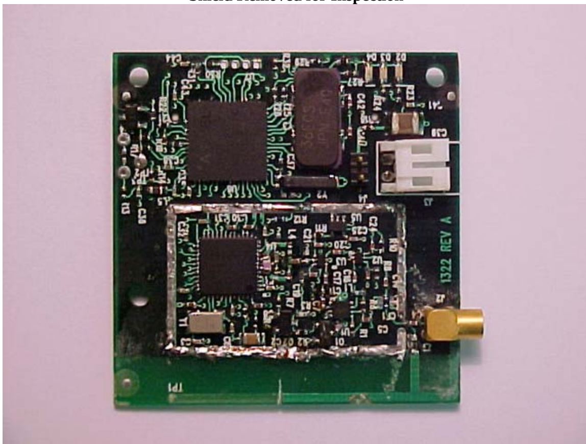
Photo One – Internal Shield Removed for Inspection
