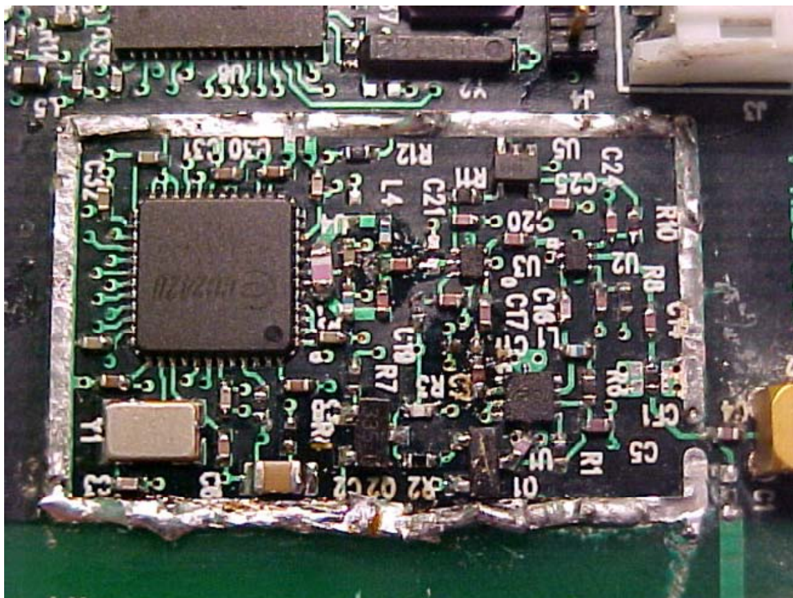
Photo Two – Internal RF Section Close-Up
