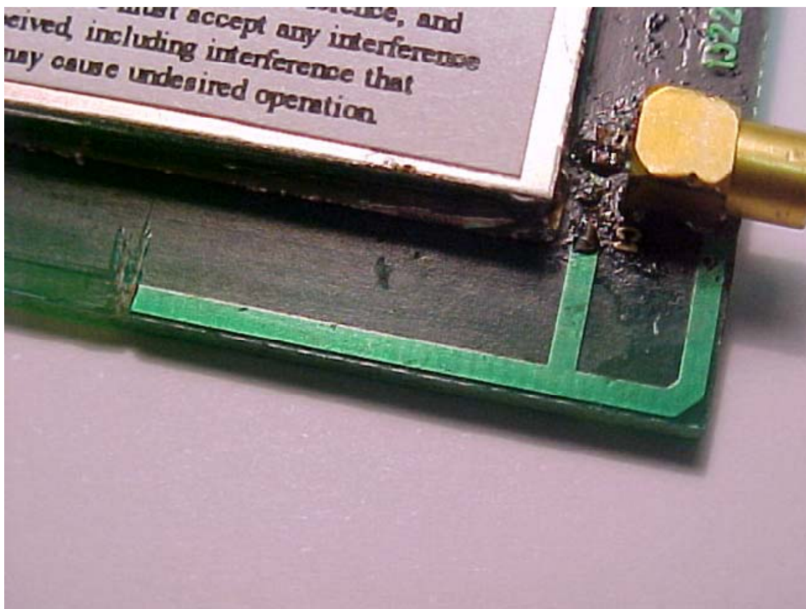
Photo Four – Internal PCB Antenna Close-Up
