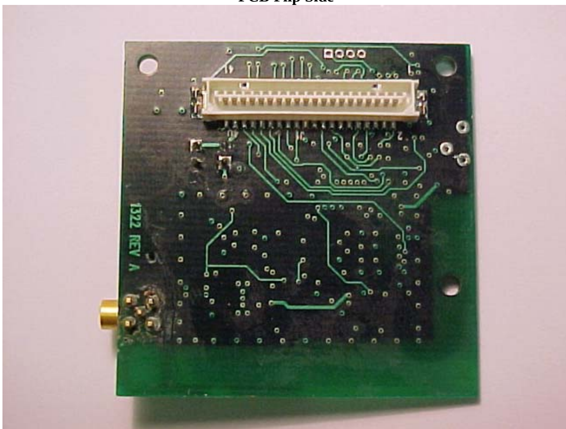
Photo Three – Internal PCB Flip Side
