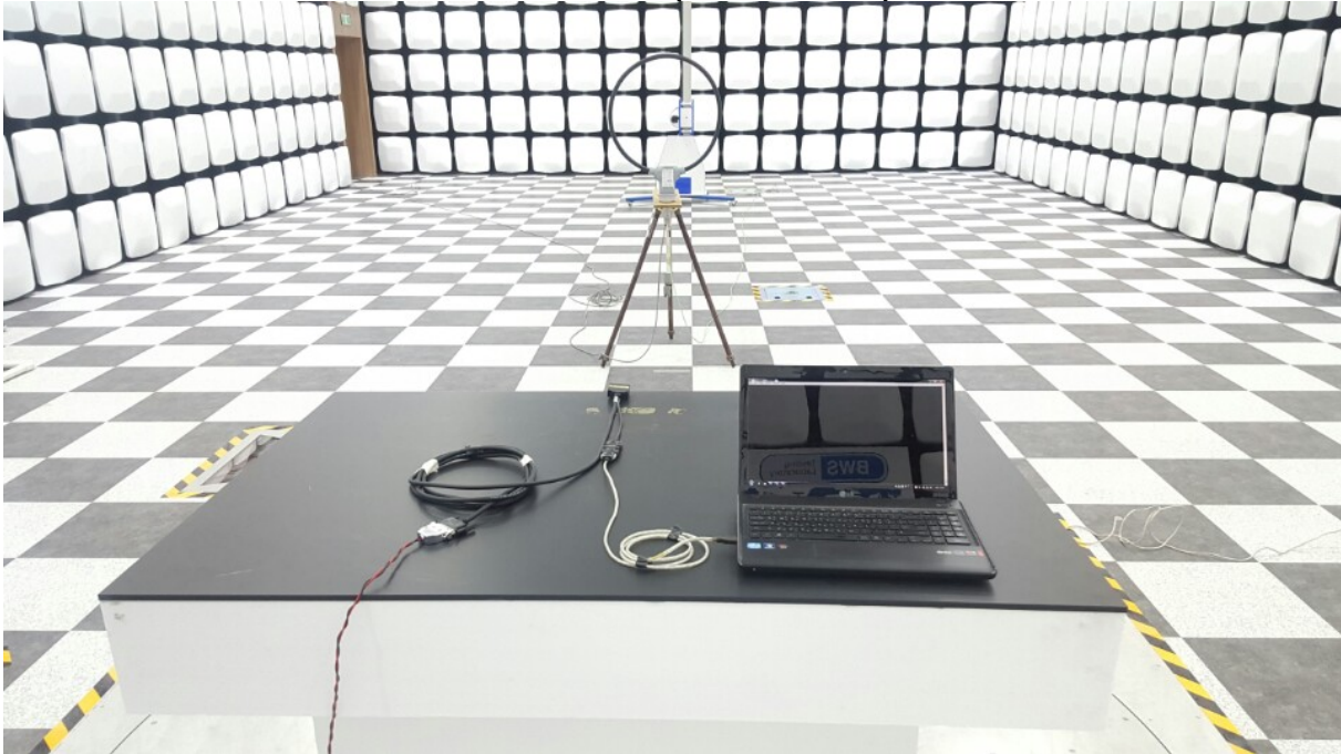
Radiated Test(0.009-30MHz)
