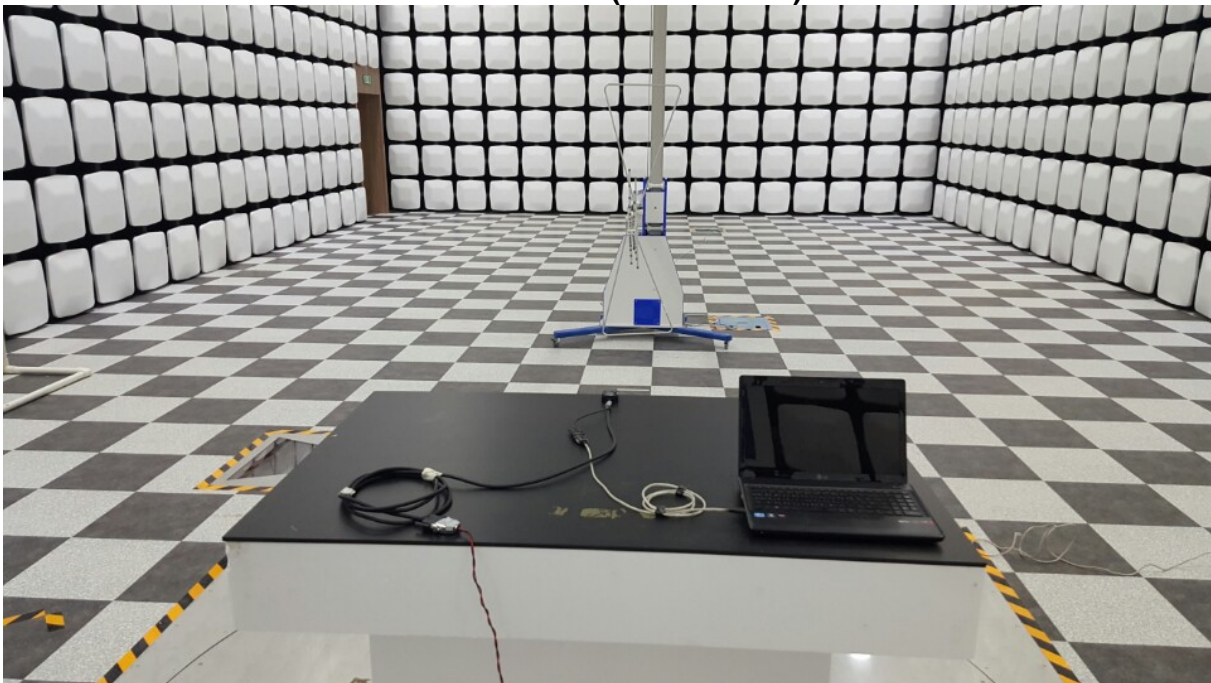
Radiated Test(30-1000MHz)
