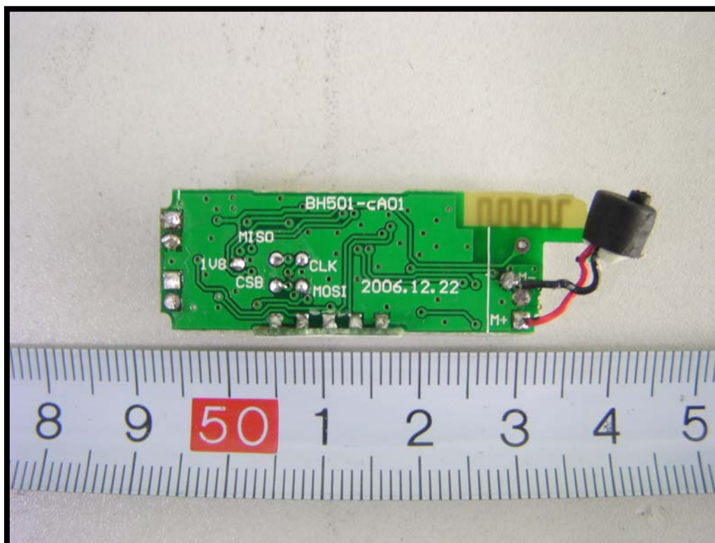
Battery View
