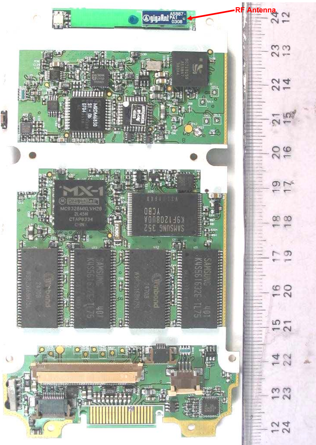
EUT PCB Top View
