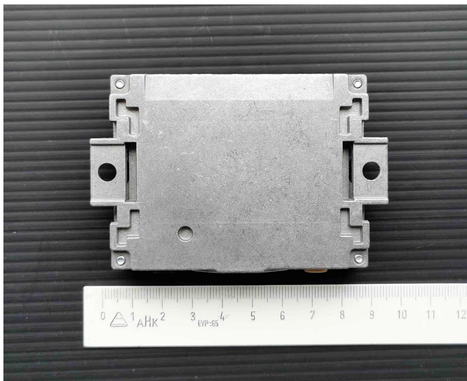
Bottom View (HVIN: 17400213, 17400214)
