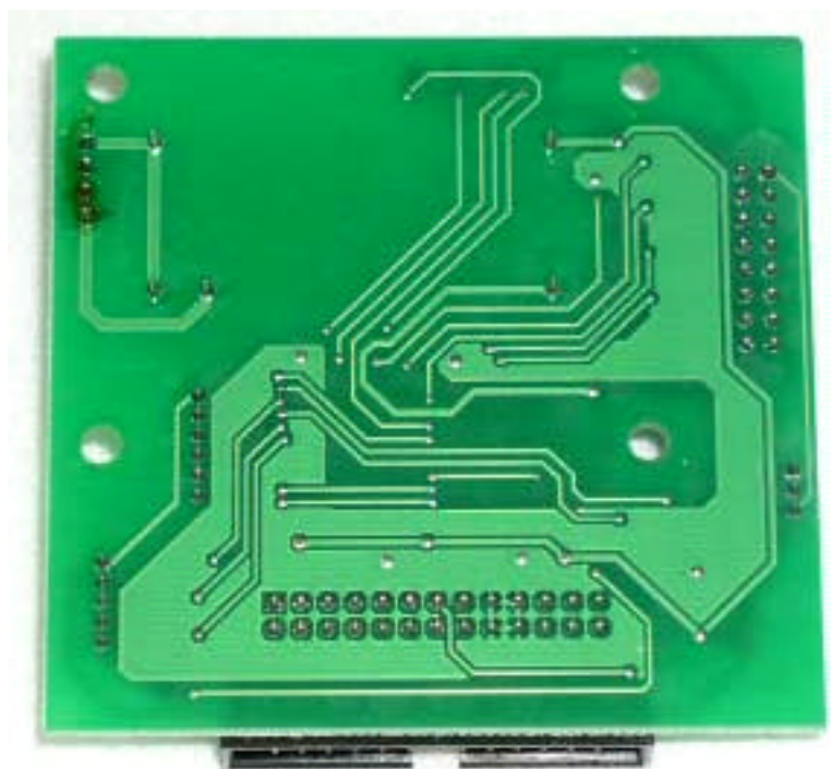
Component side view of Card Reader board
