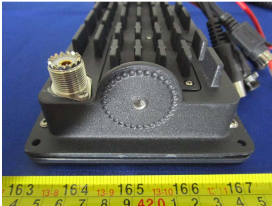
EUT – HM380S Side View
