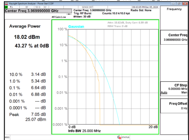
Band77-Part27_20MHz_DFT_s_OFDM_SCS30kHz_256QAM_RB50_0_CH664666
