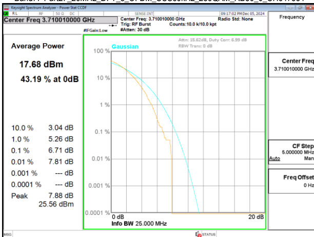
Band77-Part27_20MHz_DFT_s_OFDM_SCS30kHz_256QAM_RB50_0_CH647334
