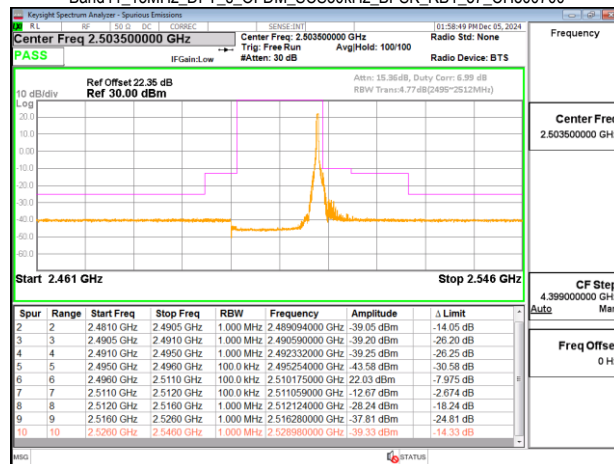
Band41_15MHz_DFT_s_OFDM_SCS30kHz_BPSK_RB36_0_CH500700
