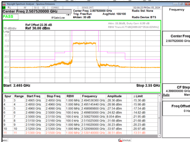
Band41_15MHz_DFT_s_OFDM_SCS30kHz_BPSK_RB36_0_CH501504
