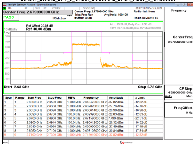
Band41 20MHz DFT_s_OFDM_SCS30kHz BPSK RB50_0_CH535998
