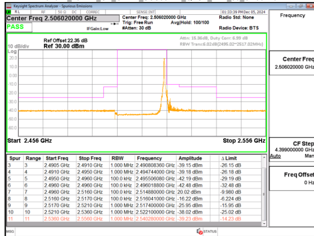
Band41 20MHz CP_OFDM_SCS30kHz QPSK RB51_0_CH501204
