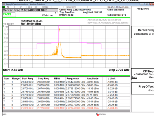
Band41_15MHz_DFT_s_OFDM_SCS30kHz_BPSK_RB1_37_CH536496
