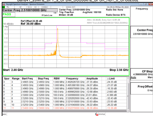
Band41_20MHz_DFT_s_OFDM_SCS30kHz_BPSK_RB1_50_CH502002
