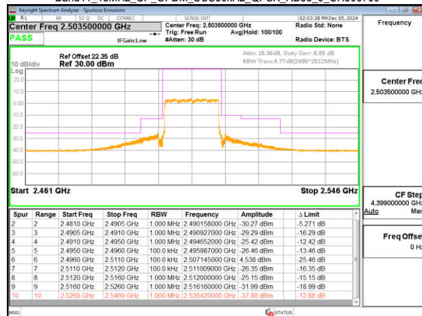
Band41_15MHz_CP_OFDM_SCS30kHz_QPSK_RB36_0_CH500700
