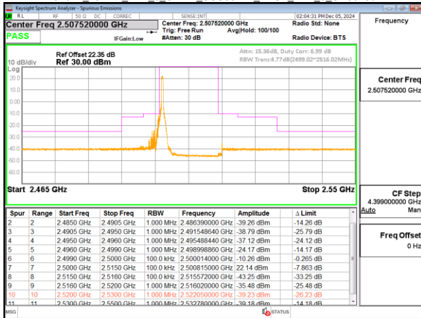
Band41_15MHz_DFT_s_OFDM_SCS30kHz_BPSK_RB1_37_CH501504
