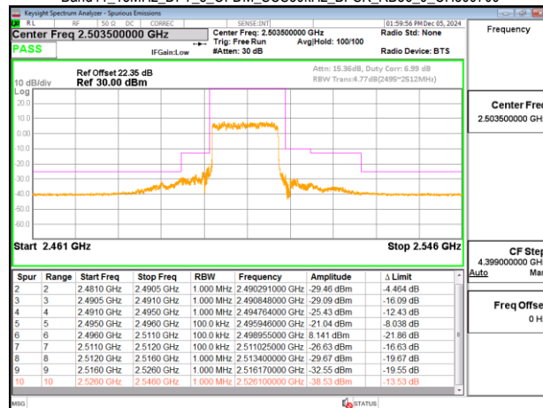
Band41_15MHz_DFT_s_OFDM_SCS30kHz_BPSK_RB36_0_CH500700
