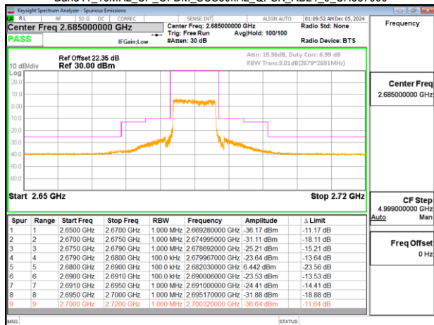
Band41_10MHz_CP_OFDM_SCS30kHz_QPSK_RB24_0_CH537000
