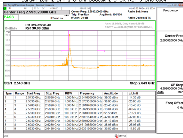
Band41_20MHz_DFT_s_OFDM_SCS30kHz_BPSK_RB1_50_CH518604
