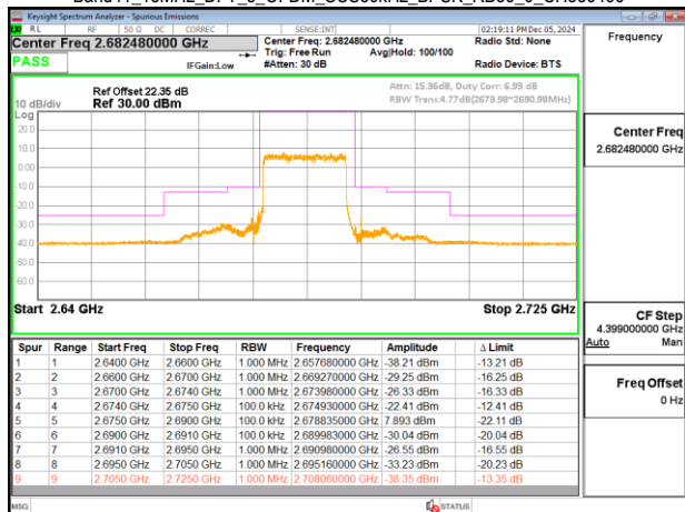
Band41_15MHz_DFT_s_OFDM_SCS30kHz_BPSK_RB36_0_CH536496
