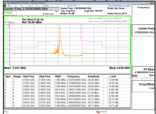
Band41_15MHz_DFT_s_OFDM_SCS30kHz_BPSK_RB1_37_CH518604
