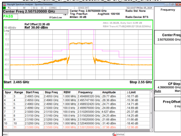
Band41_15MHz_CP_OFDM_SCS30kHz_QPSK_RB38_0_CH501504
