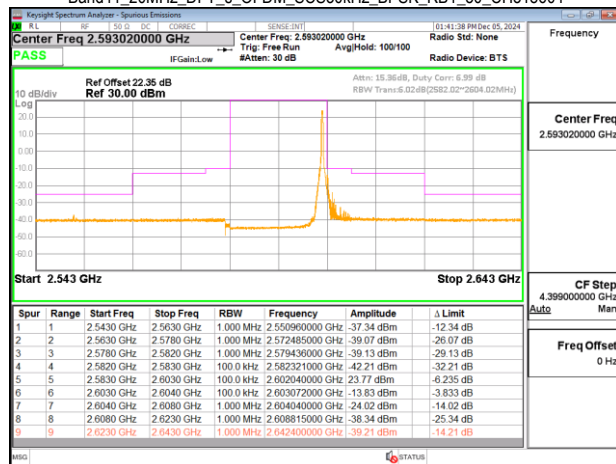
Band41_20MHz_DFT_s_OFDM_SCS30kHz_BPSK_RB50_0_CH518604
