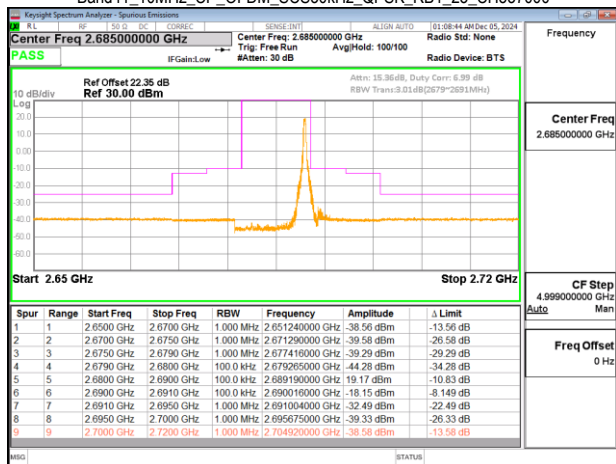
Band41_10MHz_CP_OFDM_SCS30kHz_QPSK_RB24_0_CH537000
