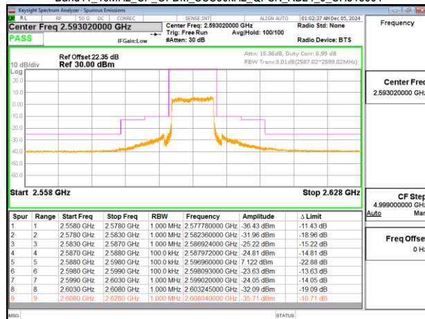
Band41_10MHz_CP_OFDM_SCS30kHz_QPSK_RB24_0_CH518604
