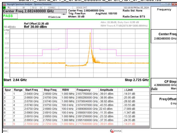
Band41_15MHz_DFT_s_OFDM_SCS30kHz_BPSK_RB36_0_CH536496
