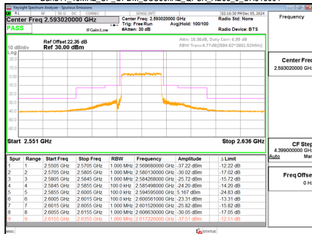
Band41_15MHz_CP_OFDM_SCS30kHz_QPSK_RB38_0_CH518604
