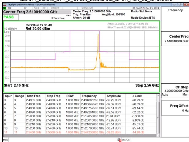
Band41_20MHz_DFT_s_OFDM_SCS30kHz_BPSK_RB50_0_CH502002
