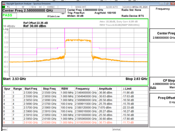
Band38_20MHz_CP_OFDM_SCS30kHz_QPSK_RB51_0_CH516000
