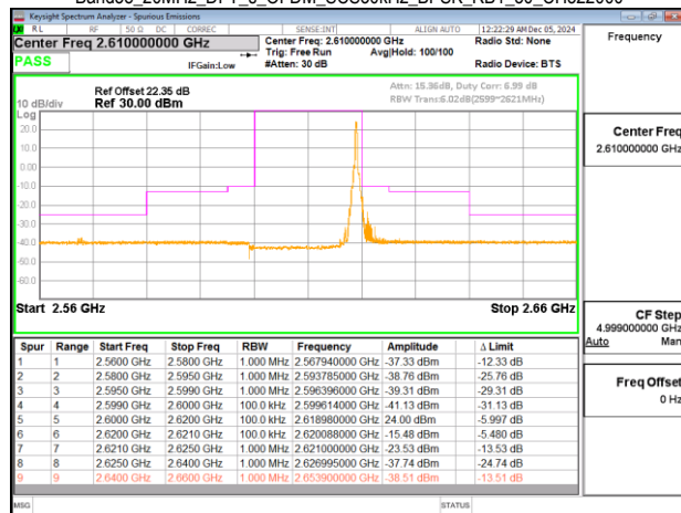
Band38_20MHz_DFT_s_OFDM_SCS30kHz_BPSK_RB50_0_CH522000
