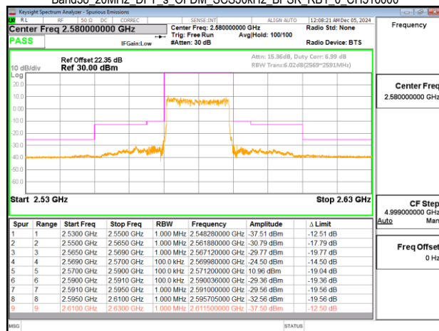
Band38_20MHz_DFT_s_OFDM_SCS30kHz_BPSK_RB1_50_CH516000
