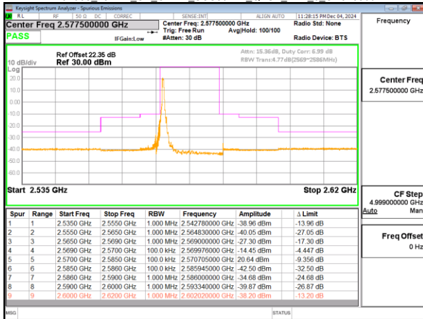
Band38_15MHz_CP_OFDM_SCS30kHz_QPSK_RB1_37_CH515500
