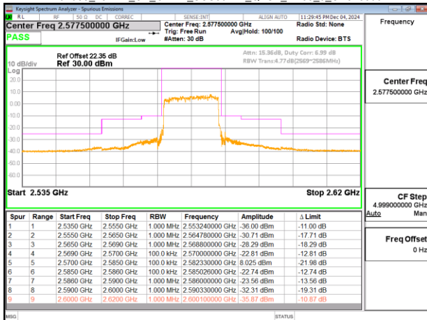
Band38_15MHz_CP_OFDM_SCS30kHz_QPSK_RB38_0_CH515500
