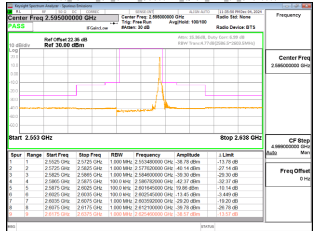
Band38_15MHz_CP_OFDM_SCS30kHz_QPSK_RB38_0_CH519000
