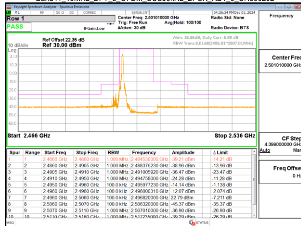
Band41_10MHz_DFT_s_OFDM_SCS30kHz_BPSK_RB1_23_CH500202
