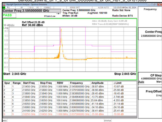
Band38_20MHz_DFT_s_OFDM_SCS30kHz_BPSK_RB1_50_CH519000
