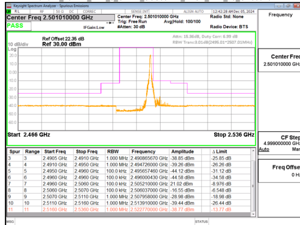
Band41_10MHz_DFT_s_OFDM_SCS30kHz_BPSK_RB24_0_CH500202
