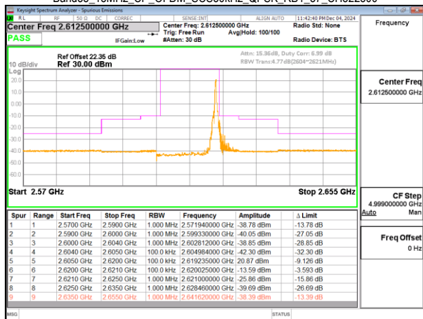
Band38_15MHz_CP_OFDM_SCS30kHz_QPSK_RB38_0_CH522500
