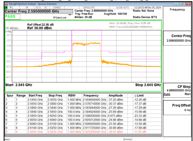
Band38_20MHz_CP_OFDM_SCS30kHz_QPSK_RB51_0_CH519000
