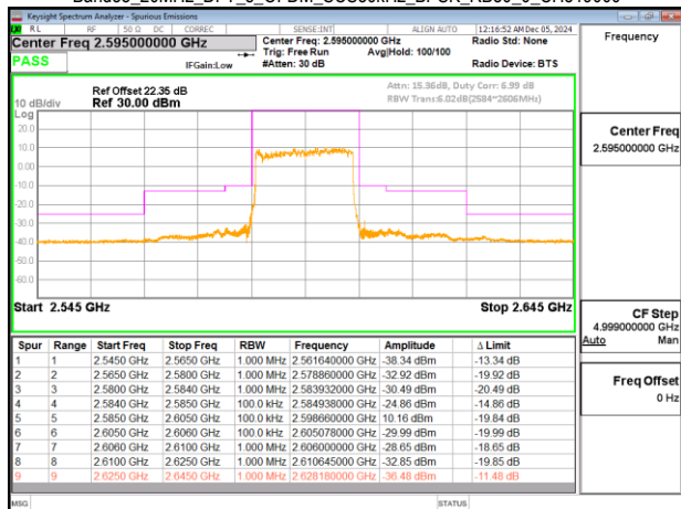
Band38_20MHz_DFT_s_OFDM_SCS30kHz_BPSK_RB50_0_CH519000
