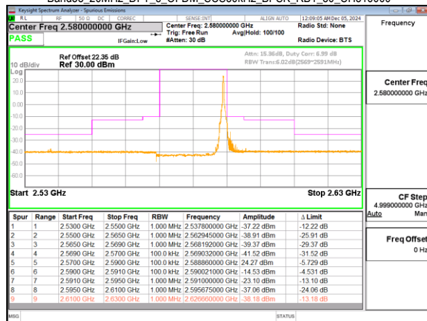
Band38_20MHz_DFT_s_OFDM_SCS30kHz_BPSK_RB50_0_CH516000
