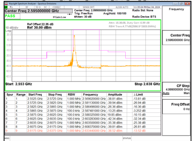
Band38_15MHz_CP_OFDM_SCS30kHz_QPSK_RB1_37_CH519000
