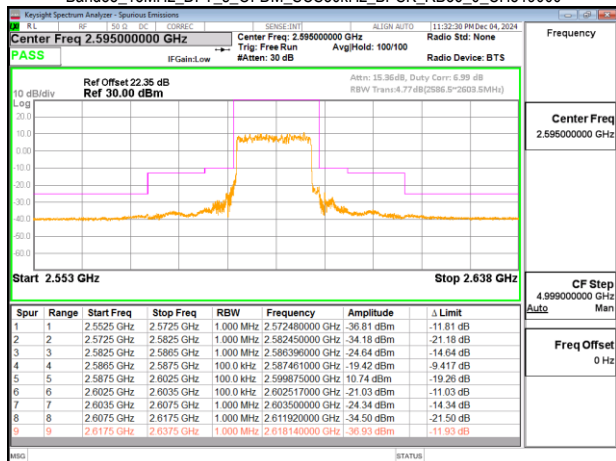
Band38_15MHz_DFT_s_OFDM_SCS30kHz_BPSK_RB36_0_CH519000
