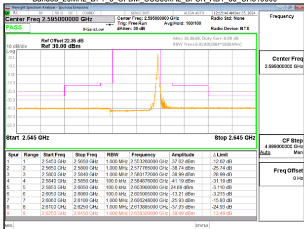
Band38_20MHz_DFT_s_OFDM_SCS30kHz_BPSK_RB50_0_CH519000
