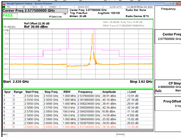
Band38_15MHz_CP_OFDM_SCS30kHz_QPSK_RB38_0_CH515500
