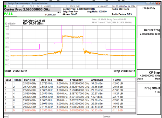
Band38_15MHz_CP_OFDM_SCS30kHz_QPSK_RB38_0_CH519000
