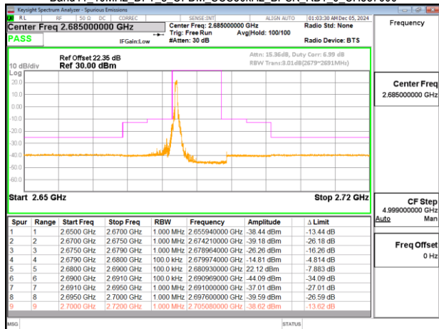
Band41_10MHz_DFT_s_OFDM_SCS30kHz_BPSK_RB1_23_CH537000
