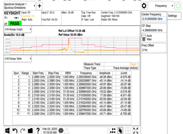
Band30_5MHz_DFT_s_OFDM_SCS15kHz_BPSK_RB1_24_CH462500
