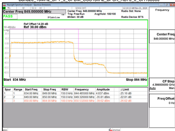
Band26_15MHz_DFT_s_OFDM_SCS15kHz_BPSK_RB75_0_CH168300
