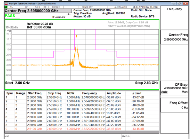
Band38_10MHz_CP_OFDM_SCS30kHz_QPSK_RB1_23_CH519000
