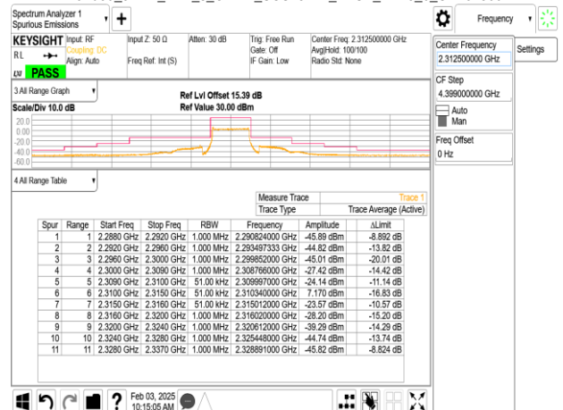
Band30_5MHz_DFT_s_OFDM_SCS15kHz_BPSK_RB25_0_CH462500
