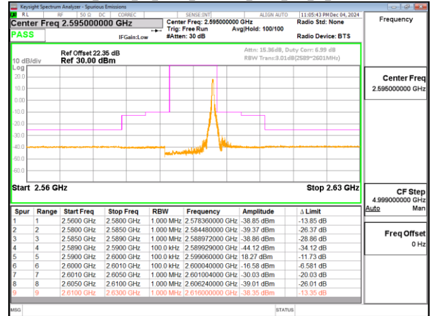
Band38_10MHz_CP_OFDM_SCS30kHz_QPSK_RB24_0_CH519000
