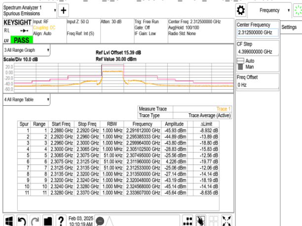
Band30_5MHz_DFT_s_OFDM_SCS15kHz_BPSK_RB25_0_CH462000
