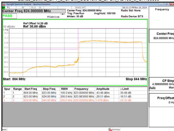
Band5_20MHz_DFT_s_OFDM_SCS15kHz_BPSK_RB100_0_CH166800
