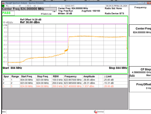
Band5_20MHz_CP_OFDM_SCS15kHz_QPSK_RB1_0_CH166800
