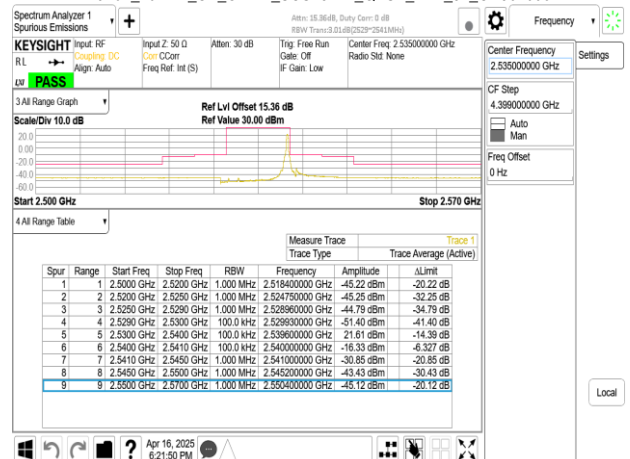
Band7_10MHz_CP_OFDM_SCS15kHz_QPSK_RB1_51_CH507000
