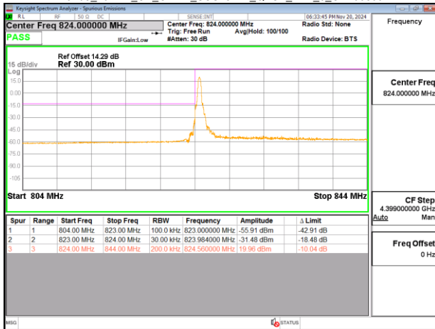
Band5_20MHz_CP_OFDM_SCS15kHz_QPSK_RB106_0_CH167800
