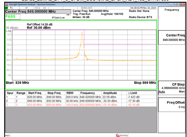
Band5_20MHz_DFT_s_OFDM_SCS15kHz_BPSK_RB1_105_CH167800
