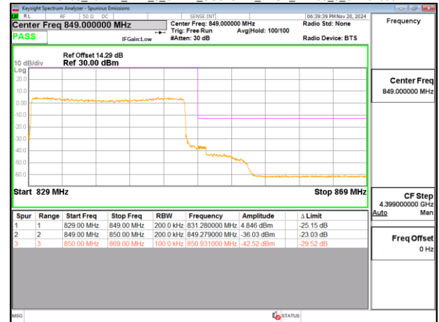
Band5_20MHz_DFT_s_OFDM_SCS15kHz_BPSK_RB1_105_CH167800
