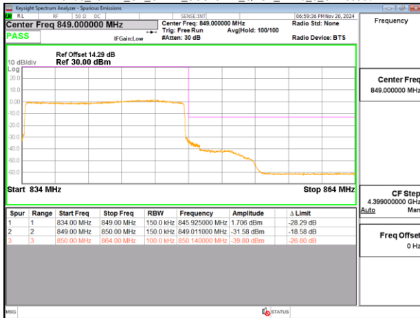
Band5_20MHz_DFT_s_OFDM_SCS15kHz_BPSK_RB100_0_CH166800
