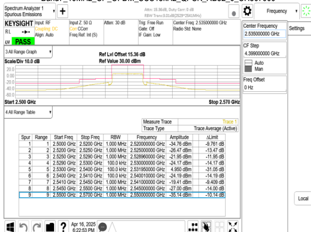
Band7_10MHz_CP_OFDM_SCS15kHz_QPSK_RB1_0.CH513000
