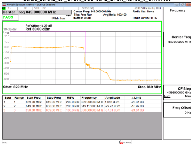
Band5_20MHz_CP_OFDM_SCS15kHz_QPSK_RB106_0_CH167800
