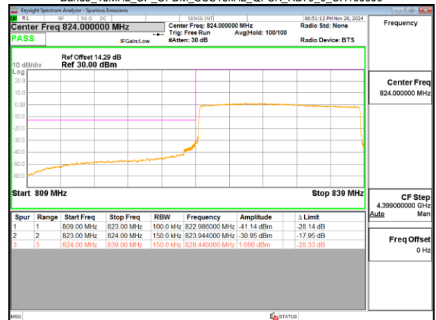
Band5_15MHz_CP_OFDM_SCS15kHz_QPSK_RB79_0_CH166300
