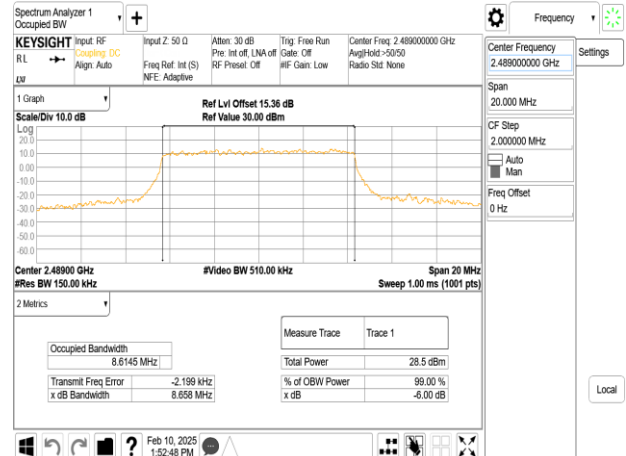
Band53_10MHz_DFT_s_OFDM_SCS30kHz_64QAM_RB24_0_CH497800
