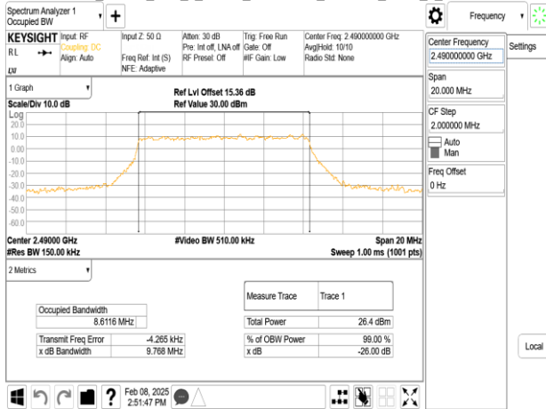
Band53_10MHz_DFT_s_OFDM_SCS30kHz_256QAM_RB24_0_CH498000
