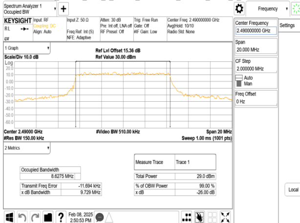
Band53_10MHz_DFT_s_OFDM_SCS30kHz_16QAM_RB24_0_CH498000
