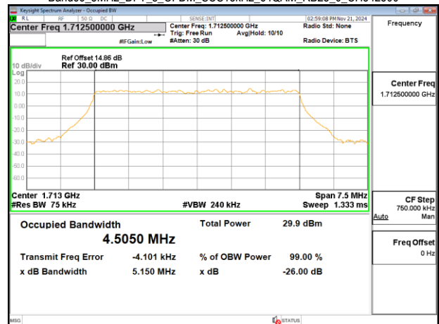
Band66_5MHz_DFT_s_OFDM_SCS15kHz_64QAM_RB25_0_CH342500
