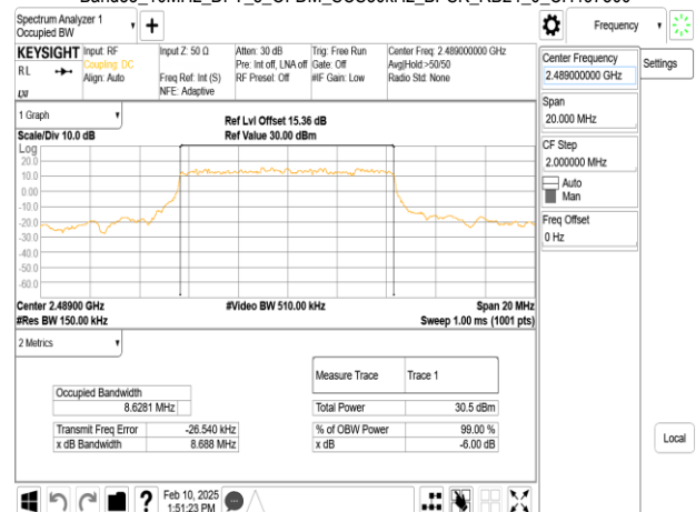
Band53_10MHz_DFT_s_OFDM_SCS30kHz_BPSK_RB24_0_CH497800
