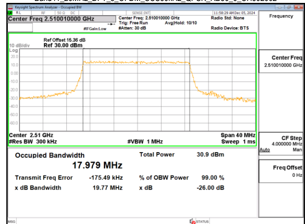
Band41_20MHz_DFT_s_OFDM_SCS30kHz_QPSK_RB50_0_CH502002
