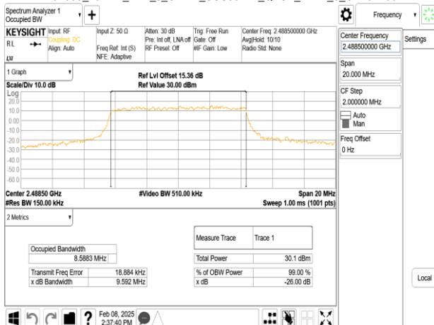
Band53_10MHz_DFT_s_OFDM_SCS30kHz_QPSK_RB24_0_CH497700
