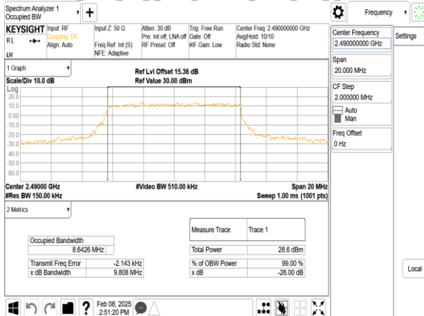
Band53_10MHz_DFT_s_OFDM_SCS30kHz_64QAM_RB24_0_CH498000
