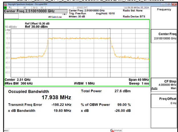
Band41_20MHz_DFT_s_OFDM_SCS30kHz_256QAM_RB50_0_CH502002
