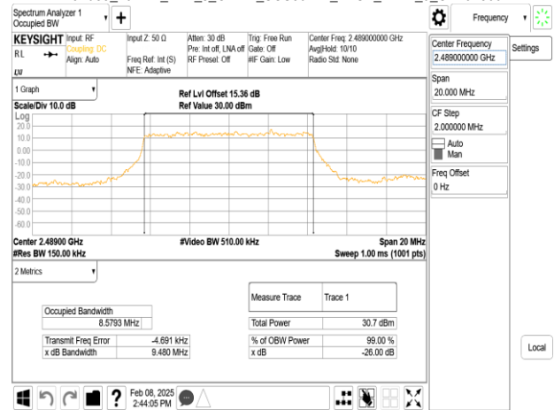
Band53_10MHz_DFT_s_OFDM_SCS30kHz_BPSK_RB24_0_CH497800
