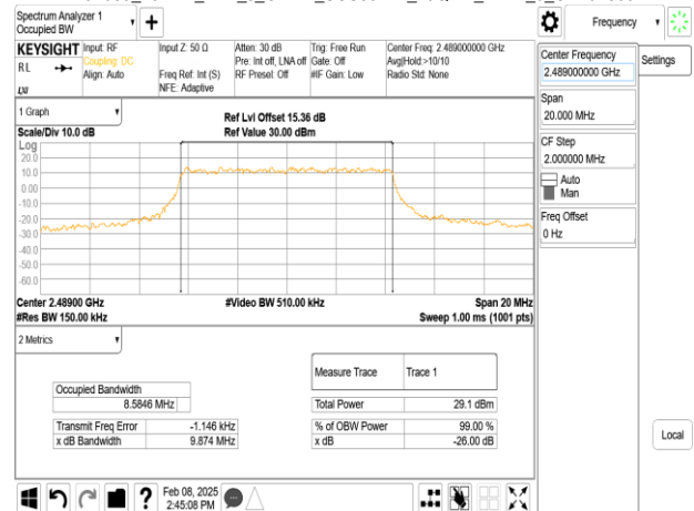
Band53_10MHz_DFT_s_OFDM_SCS30kHz_16QAM_RB24_0_CH497800
