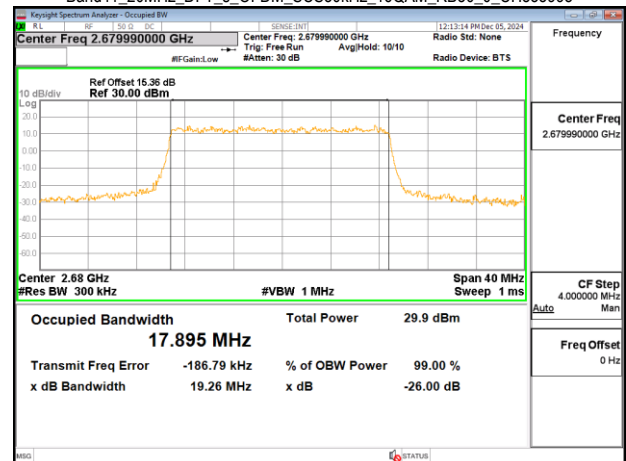
Band41_20MHz_DFT_s_OFDM_SCS30kHz_16QAM_RB50_0_CH535998
