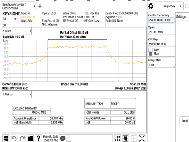
Band53_10MHz_DFT_s_OFDM_SCS30kHz_BPSK_RB24_0_CH498000
