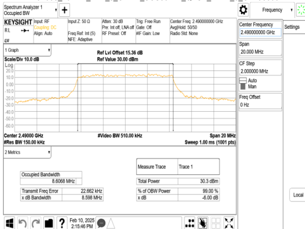
Band53_10MHz_DFT_s_OFDM_SCS30kHz_16QAM_RB24_0_CH497700
