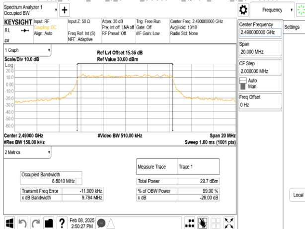
Band53_10MHz_DFT_s_OFDM_SCS30kHz_QPSK_RB24_0_CH498000
