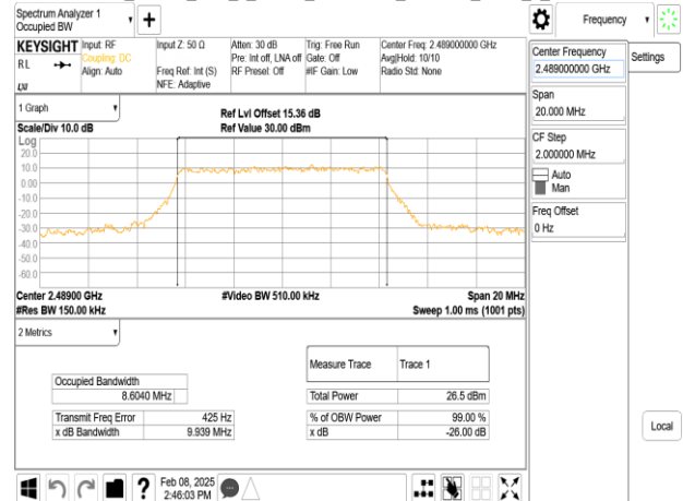
Band53_10MHz_DFT_s_OFDM_SCS30kHz_256QAM_RB24_0_CH497800
