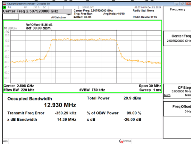
Band41_15MHz_DFT_s_OFDM_SCS30kHz_16QAM_RB36_0_CH518604
