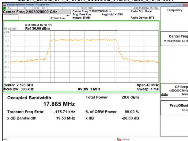
Band41_20MHz_DFT_s_OFDM_SCS30kHz_64QAM_RB50_0_CH518604
