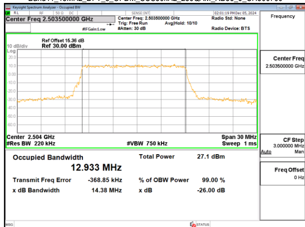
Band41_15MHz_DFT_s_OFDM_SCS30kHz_256QAM_RB36_0_CH500700
