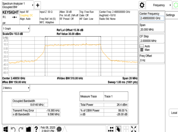
Band53_10MHz_DFT_s_OFDM_SCS30kHz_256QAM_RB24_0_CH497700
