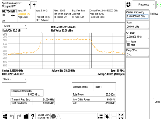
Band53_10MHz_DFT_s_OFDM_SCS30kHz_64QAM_RB24_0_CH497700
