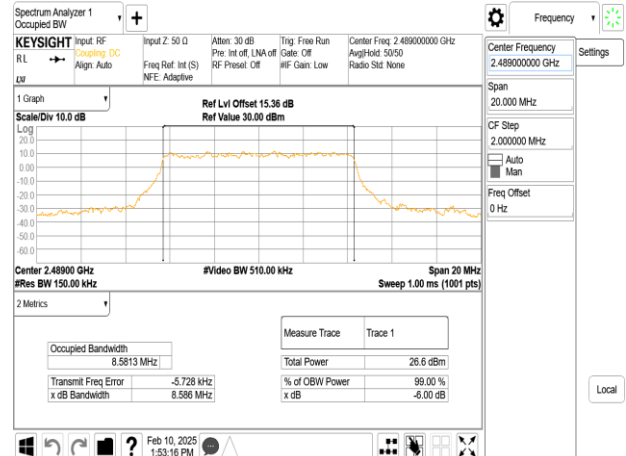
Band53_10MHz_DFT_s_OFDM_SCS30kHz_256QAM_RB24_0_CH497800
