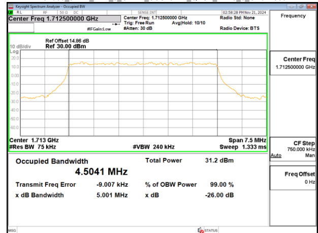
Band66_5MHz_DFT_s_OFDM_SCS15kHz_QPSK_RB25_0_CH342500
