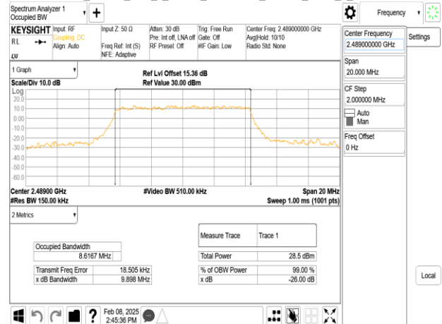
Band53_10MHz_DFT_s_OFDM_SCS30kHz_64QAM_RB24_0_CH497800
