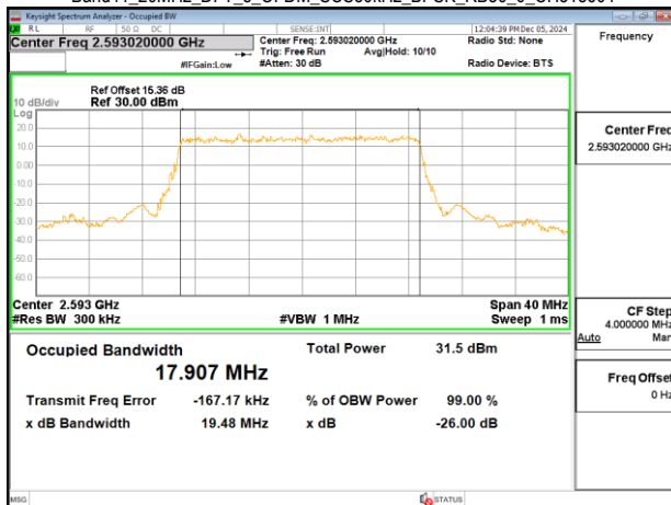
Band41_20MHz_DFT_s_OFDM_SCS30kHz_BPSK_RB50_0_CH518604
