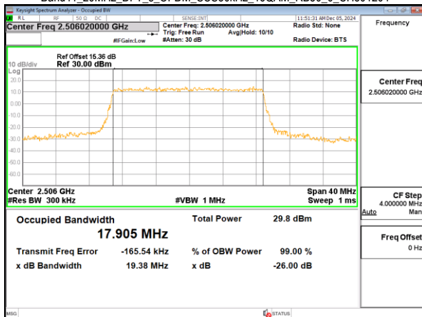
Band41_20MHz_DFT_s_OFDM_SCS30kHz_16QAM_RB50_0_CH501204
