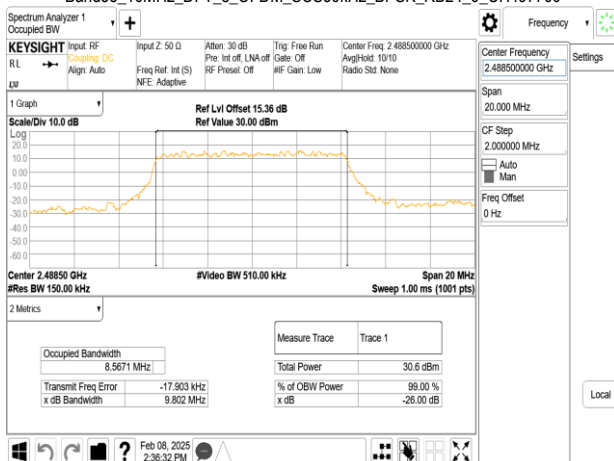
Band53_10MHz_DFT_s_OFDM_SCS30kHz_BPSK_RB24_0_CH497700
