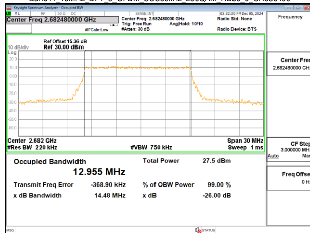
Band41_15MHz_DFT_s_OFDM_SCS30kHz_256QAM_RB36_0_CH536496
