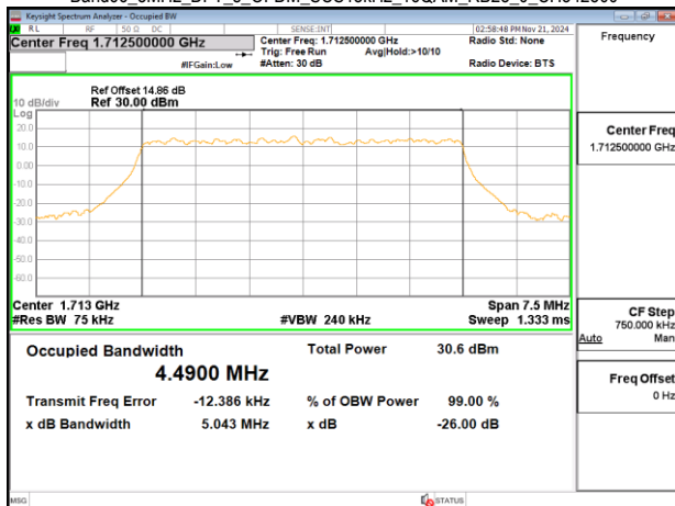
Band66_5MHz_DFT_s_OFDM_SCS15kHz_16QAM_RB25_0_CH342500
