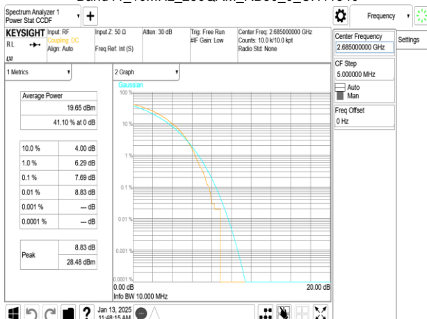
Band41_10MHz_256QAM_RB50_0_CH41540
