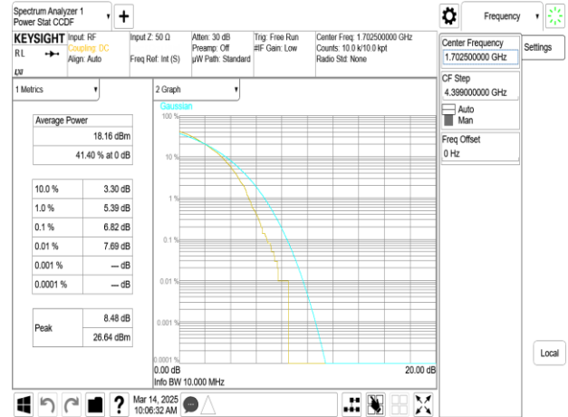
Band70_10MHz_256QAM_RB50_0_CH133072
