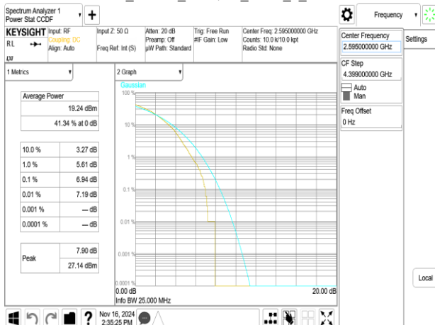
Band38_15MHz_256QAM_RB75_0_CH38000
