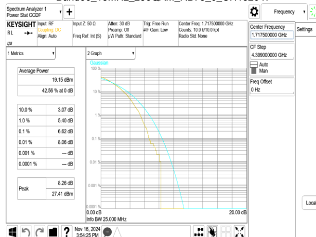
Band66_15MHz_256QAM_RB75_0_CH132047
