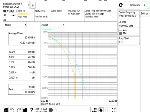
Band41_10MHz_256QAM_RB50_0_CH39700
