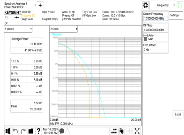
Band70_15MHz_256QAM_RB75_0_CH133047
