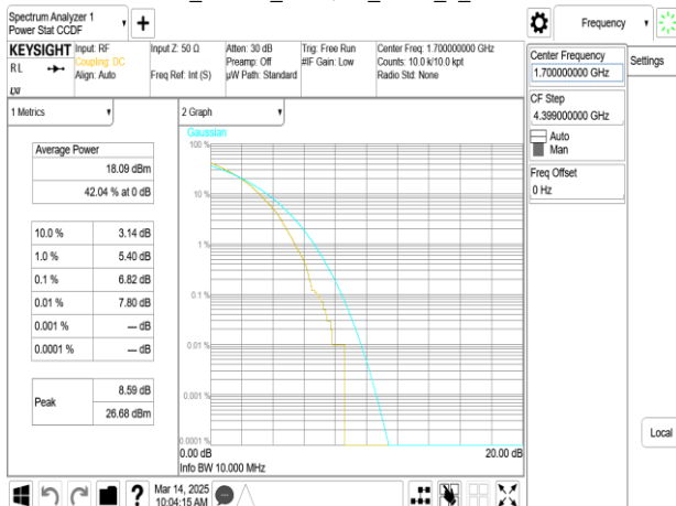
Band70_10MHz_256QAM_RB50_0_CH133022
