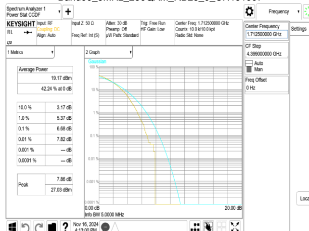
Band66_5MHz_256QAM_RB25_0_CH131997
