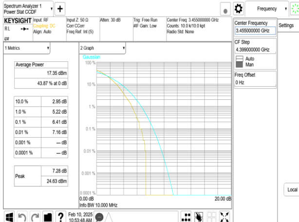
Band42-Part27_10MHz_256QAM_RB50_0_CH42140
