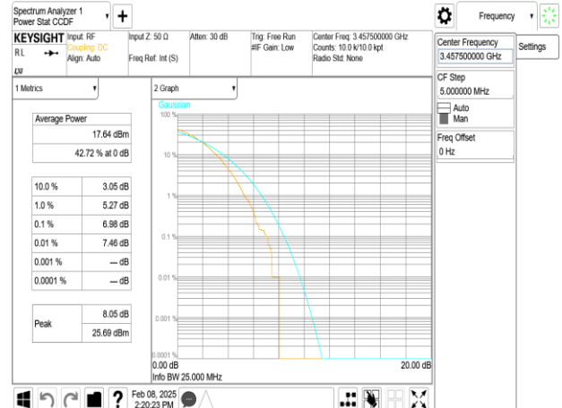
Band42-Part27_15MHz_256QAM_RB75_0_CH42165
