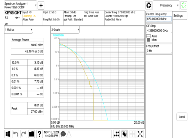
Band71_20MHz_256QAM_RB100_0_CH133297
