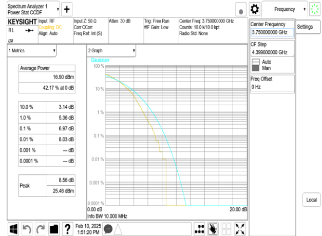
Band43-Part27_10MHz_256QAM_RB50_0_CH45540
