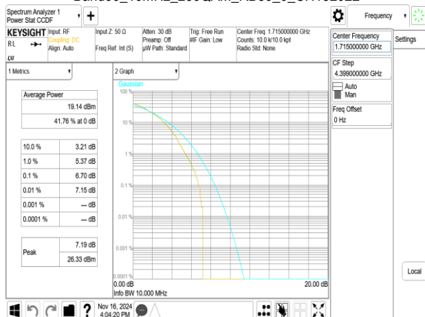
Band66_10MHz_256QAM_RB50_0_CH132022
