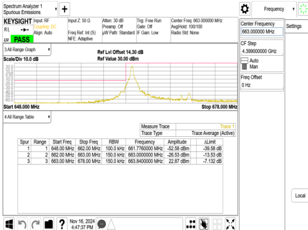
Band71_15MHz_QPSK_RB75_0_CH133197
