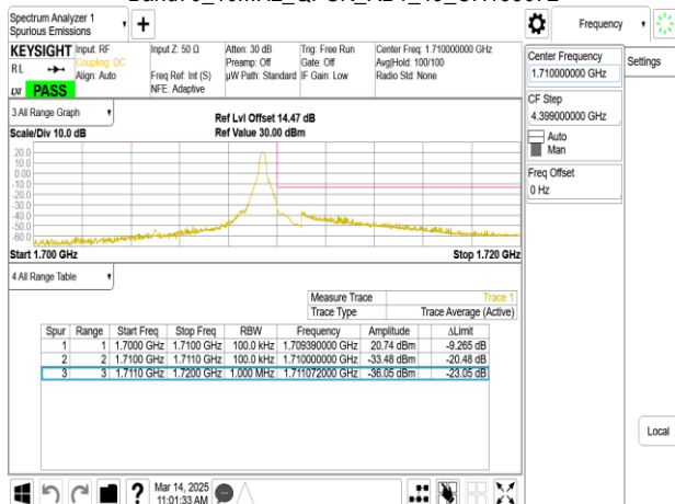
Band70_10MHz_QPSK_RB50_0_CH133072
