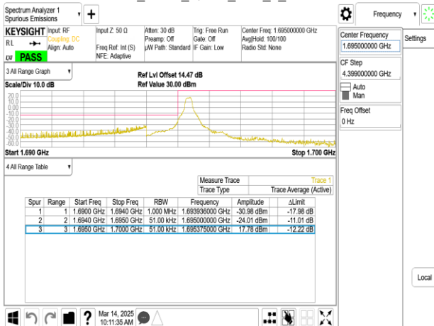
Band70_5MHz_QPSK_RB25_0_CH132997
