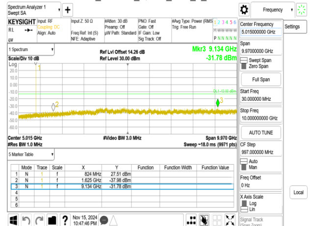
Band5_1.4MHz_QPSK_RB1_0_CH20525
