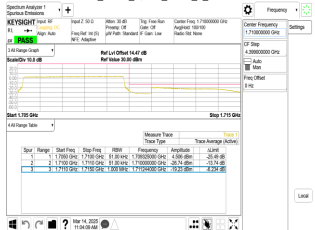
Band70_10MHz_QPSK_RB1_0_CH133022
