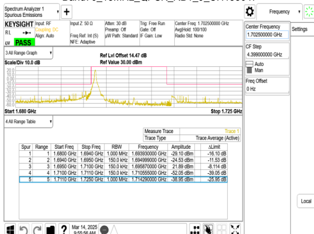
Band70_15MHz_QPSK_RB1_0_CH133047
