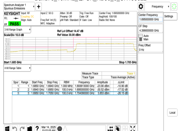
Band70_10MHz_QPSK_RB50_0_CH133022
