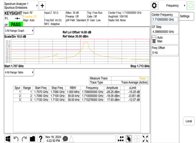
Band66_3MHz_QPSK_RB15_0_CH131987
