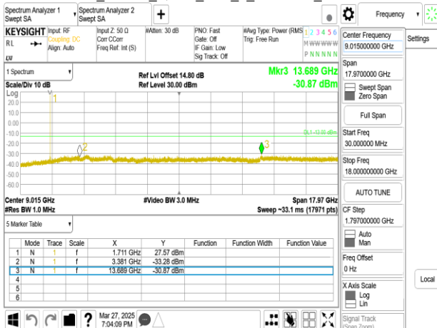
Band4_20MHz_QPSK_RB1_0_CH20175_below 18G
