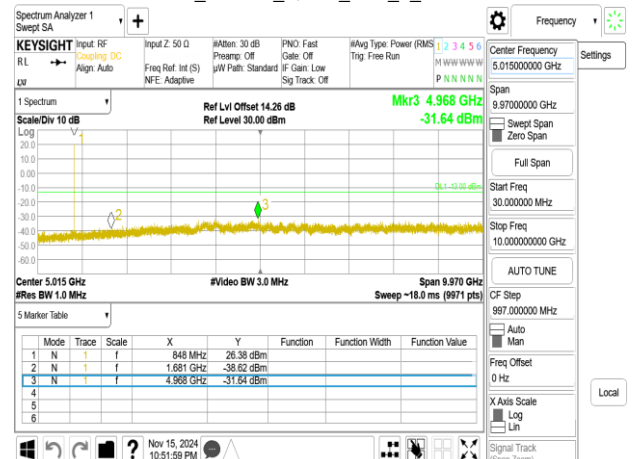
Band5_1.4MHz_QPSK_RB1_0_CH20643
