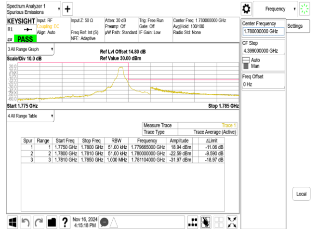
Band66_5MHz_QPSK_RB25_0_CH132647
