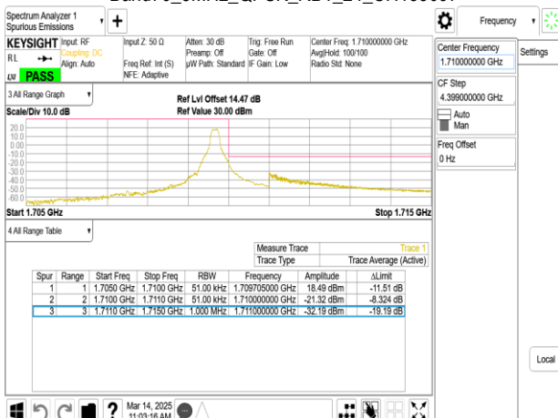
Band70_5MHz_QPSK_RB1_24_CH133097
