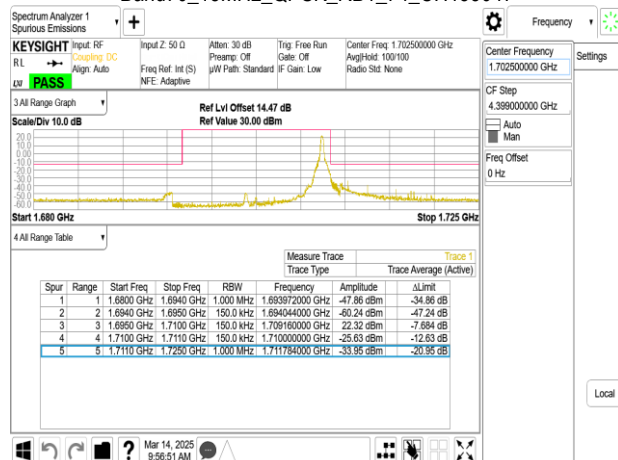
Band70_15MHz_QPSK_RB75_0_CH133047
