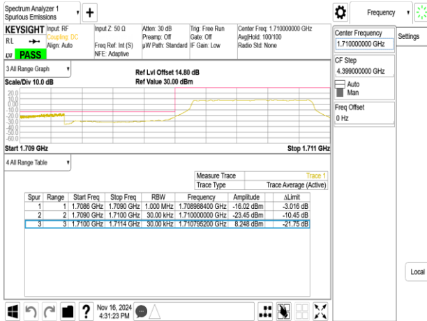
Band66_1.4MHz_QPSK_RB1_5_CH132665
