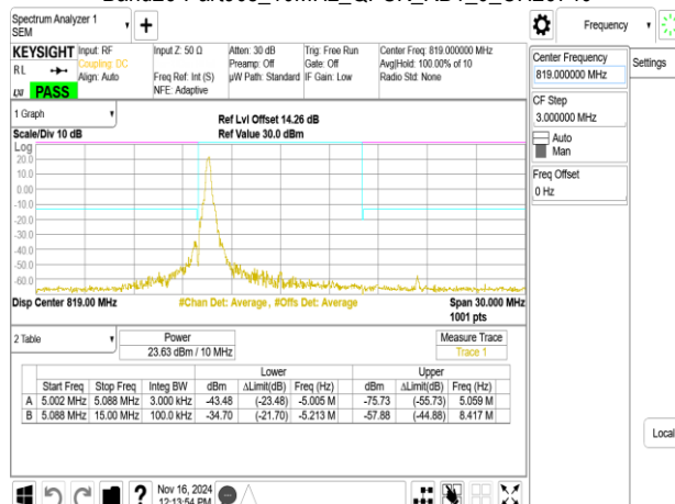
Band26-Part90s_10MHz_QPSK_RB1_0_CH26740
