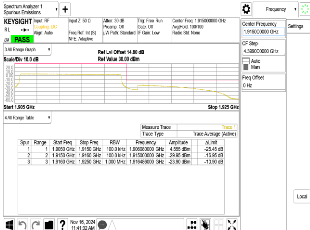
Band25_10MHz_QPSK_RB50_0_CH26640
