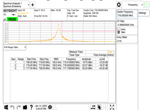
Band17_10MHz_QPSK_RB50_0_CH23800
