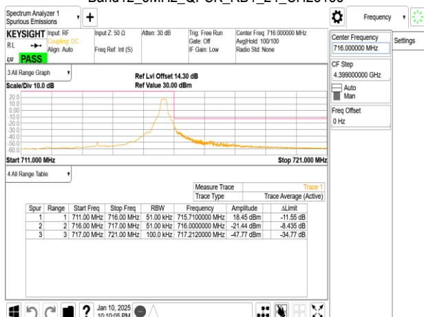
Band12_5MHz_QPSK_RB1_24_CH23155
