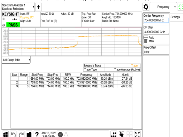
Band17_10MHz_QPSK_RB50_0_CH23780
