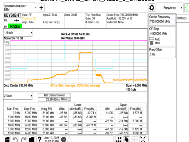
Band14_5MHz_QPSK_RB25_0_CH23355
