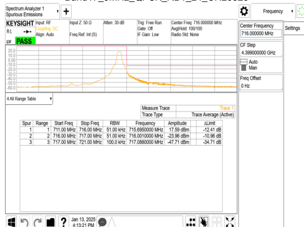
Band17_5MHz_QPSK_RB1_24_CH23825
