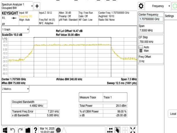
Band70_5MHz_64QAM_25_0_CH133097
