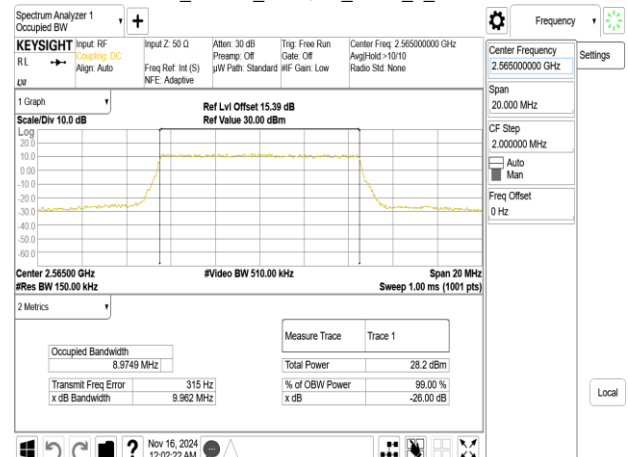
Band7_10MHz_256QAM_RB50_0_CH21400
