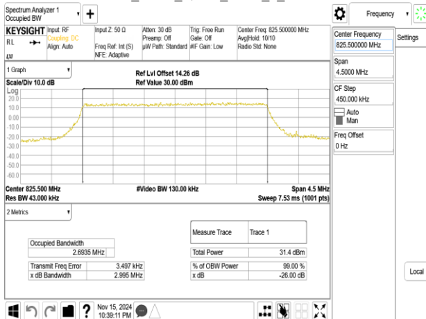
Band5_3MHz_16QAM_RB15_0_CH20415
