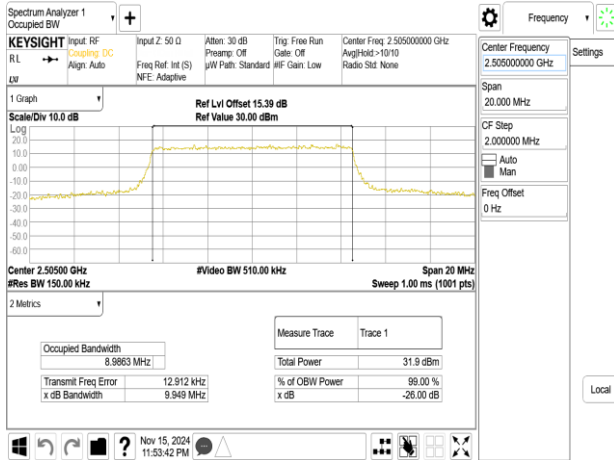
Band7_10MHz_16QAM_RB50_0_CH20800
