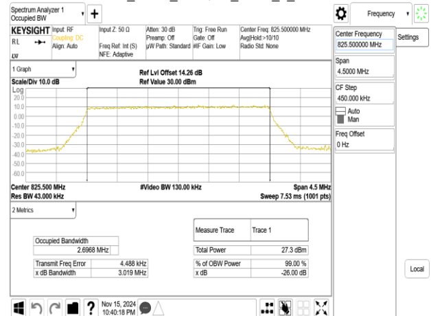
Band5_3MHz_QPSK_RB15_0_CH20525
