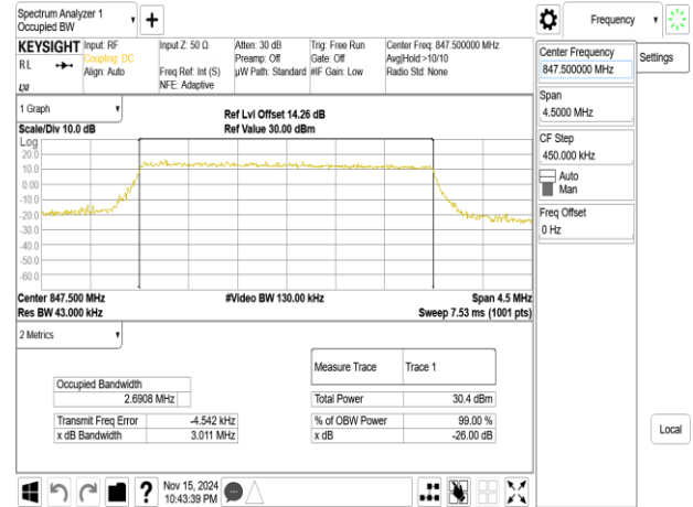
Band5_3MHz_64QAM_RB15_0_CH20635
