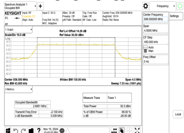
Band5_3MHz_16QAM_RB15_0_CH20525
