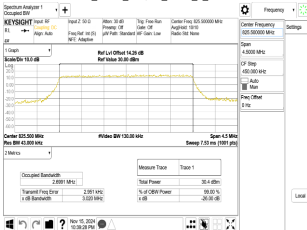
Band5_3MHz_64QAM_RB15_0_CH20415
