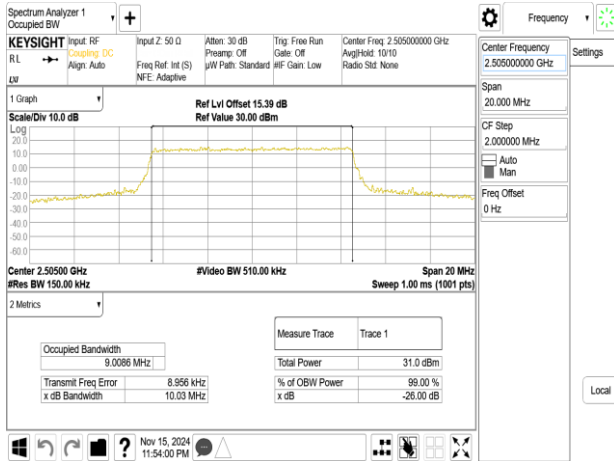
Band7_10MHz_64QAM_RB50_0_CH20800
