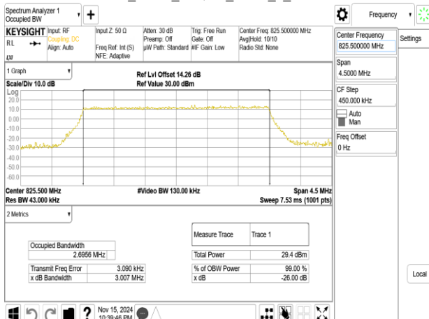
Band5_3MHz_64QAM_RB15_0_CH20415
