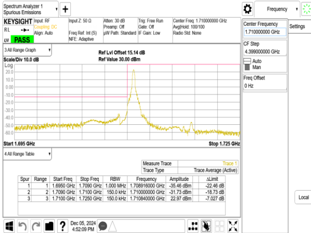
Band66_15MHz_QPSK_RB75_0_CH132047
