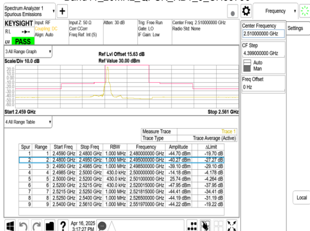
Band41_20MHz_QPSK_RB1_99_CH39790
