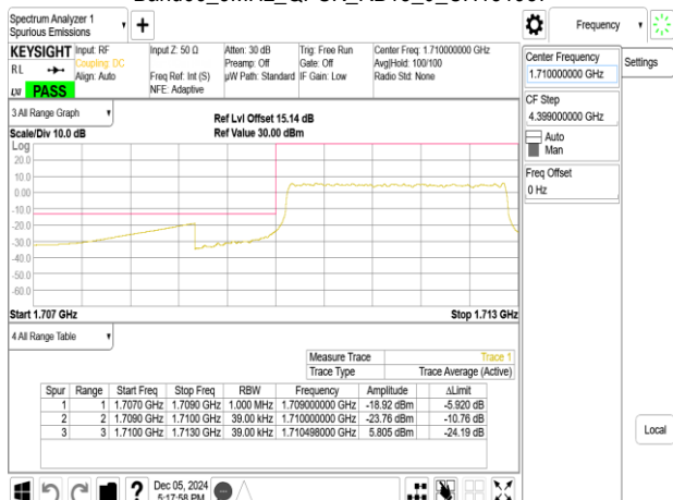
Band66_3MHz_QPSK_RB15_0_CH131987
