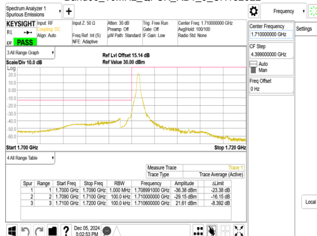
Band66_10MHz_QPSK_RB50_0_CH132022
