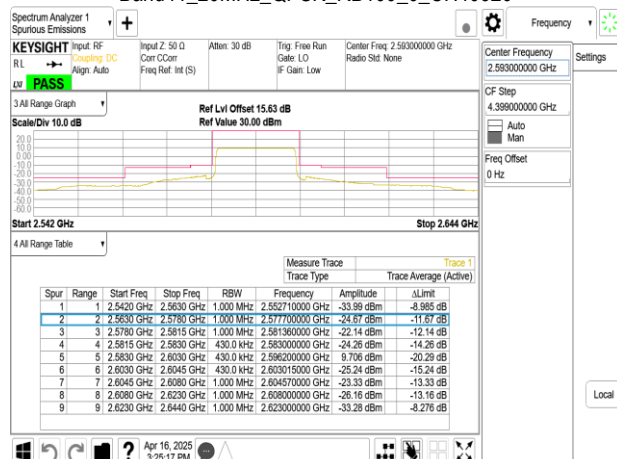
Band41_20MHz_QPSK_RB100_0_CH40620
