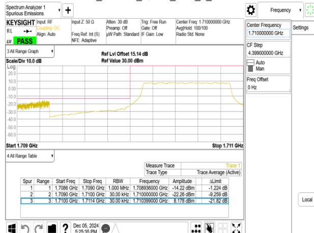
Band66_1.4MHz_QPSK_RB1_5_CH132665
