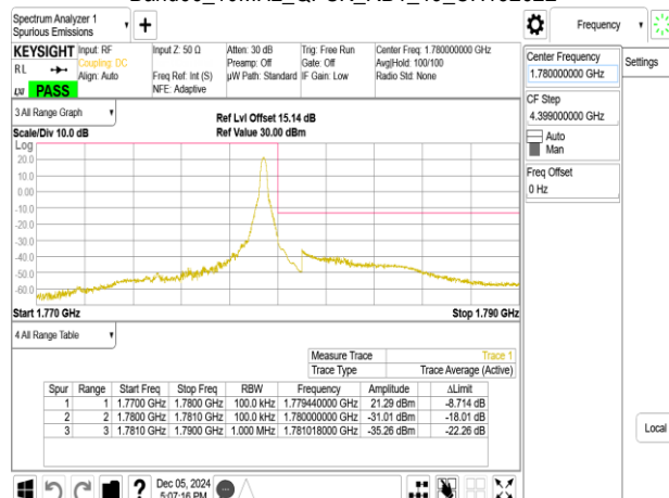
Band66_10MHz_QPSK_RB1_49_CH132622
