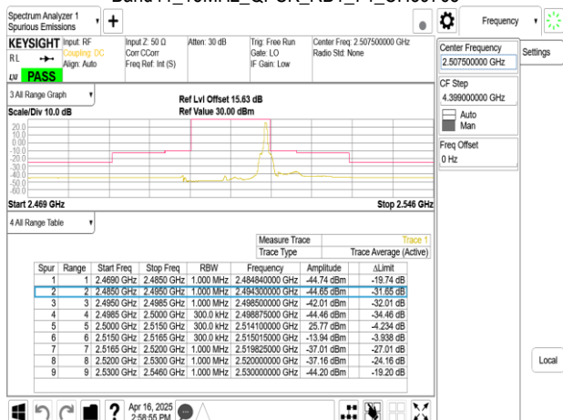
Band41_15MHz_QPSK_RB75_0_CH39765
