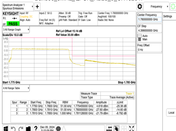
Band66_5MHz_QPSK_RB25_0_CH132647
