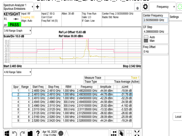
Band41_15MHz_QPSK_RB75_0_CH39725
