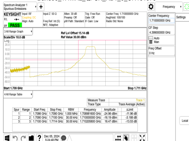
Band66_1.4MHz_QPSK_RB6_0_CH131979
